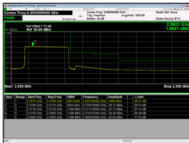
LTE Band7 64QAM BW=10MHz HighChannel=21400 RB Size=50 Position=#0
