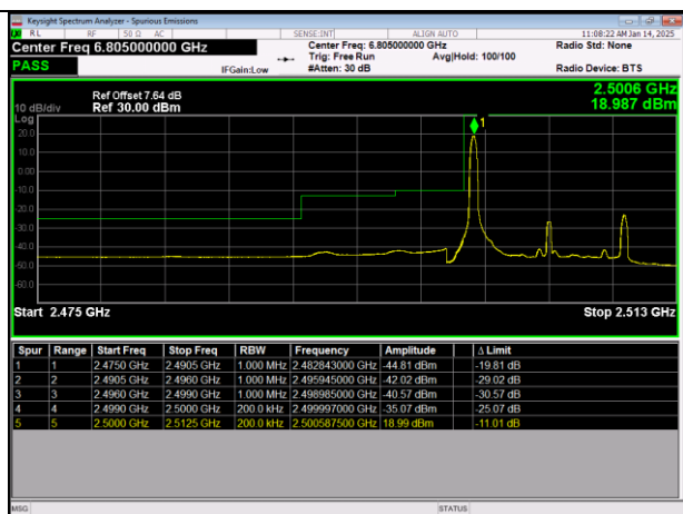
LTE Band7 64QAM BW=10MHz LowChannel=20800 RB Size=1 Position=#0
