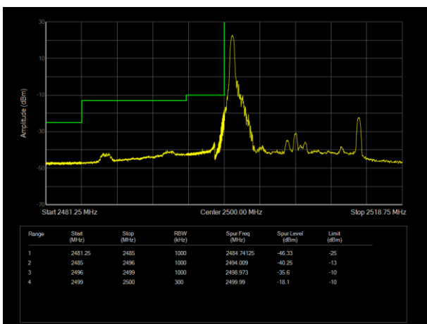
LTE Band7 16QAM BW=15MHz Channel=20825 RB Size=1 Position=#0
