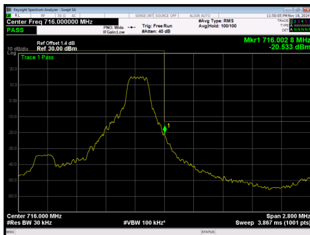
LTE Band12 16QAM BW=1.4MHz Channel=23173 RB Size=1 Position=#Max
