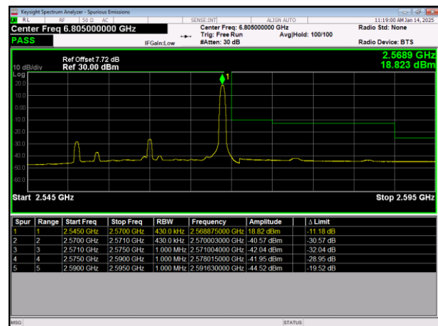
LTE Band7 64QAM BW=20MHz HighChannel=21350 RB Size=1 Position=#Max
