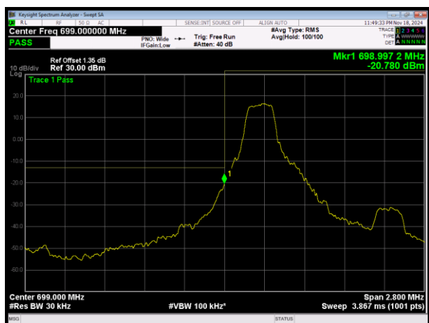
LTE Band12 QPSK BW=1.4MHz Channel=23017 RB Size=1 Position=#0
