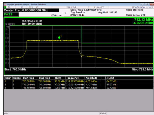
LTE Band12 64QAM BW=10MHz HighChannel=23130 RB Size=50 Position=#0
