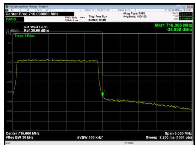
LTE Band12 16QAM BW=3MHz Channel=23165 RB Size=15 Position=#0
