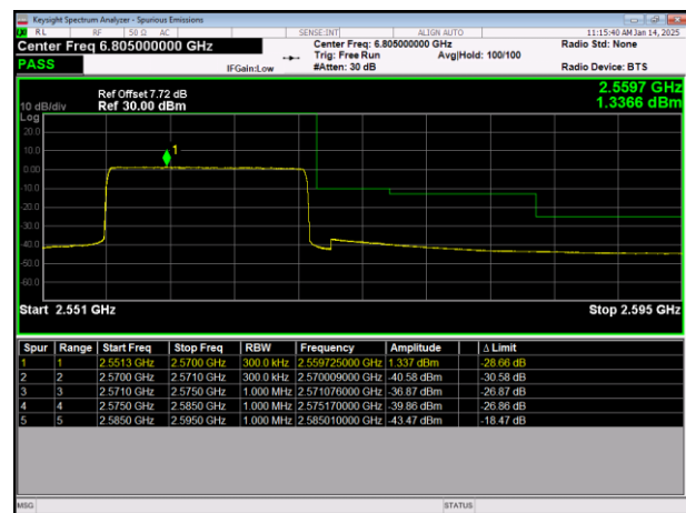
LTE Band7 64QAM BW=15MHz HighChannel=21375 RB Size=75 Position=#0
