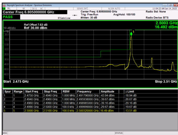
LTE Band7 64QAM BW=5MHz LowChannel=20775 RB Size=1 Position=#0
