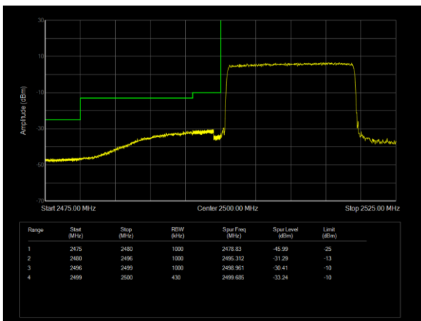
LTE Band7 16QAM BW=20MHz Channel=20850 RB Size=100 Position=#0
