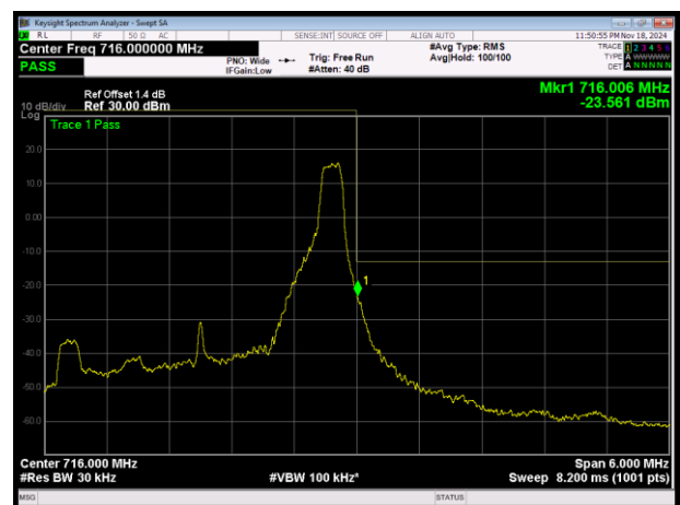
LTE Band12 16QAM BW=3MHz Channel=23165 RB Size=1 Position=#Max
