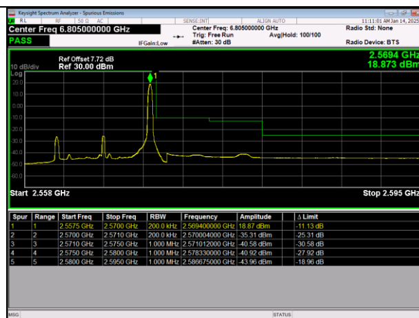
LTE Band7 64QAM BW=10MHz HighChannel=21400 RB Size=1 Position=#Max
