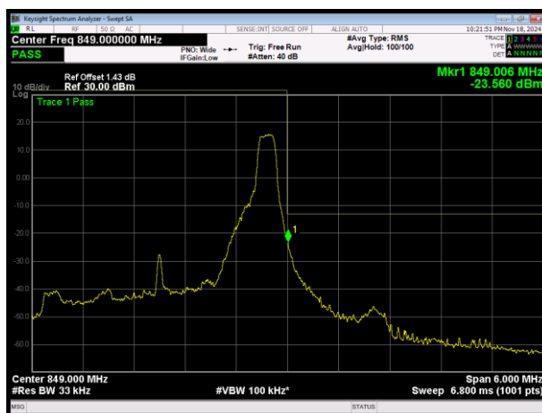
LTE Band5 16QAM BW=3MHz Channel=20635 RB Size=1 Position=#Max
