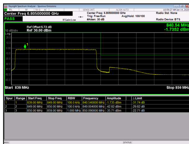
LTE Band5 64QAM BW=10MHz HighChannel=20600 RB Size=50 Position=#0
