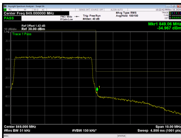
LTE Band5 16QAM BW=5MHz Channel=20625 RB Size=25 Position=#0
