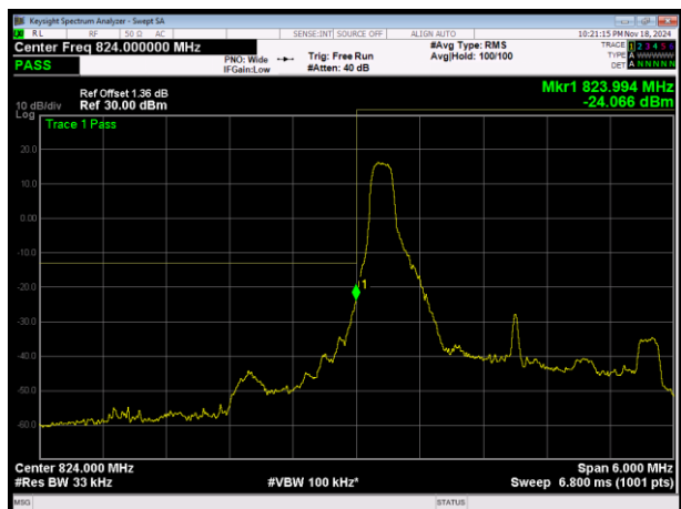
LTE Band5 QPSK BW=3MHz Channel=20415 RB Size=1 Position=#0
