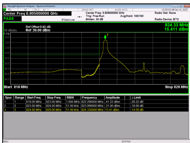
LTE Band5 64QAM BW=5MHz LowChannel=20425 RB Size=1 Position=#0
