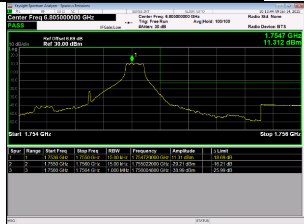
LTE Band4 64QAM BW=1.4MHz HighChannel=20393 RB Size=1 Position=#Max
