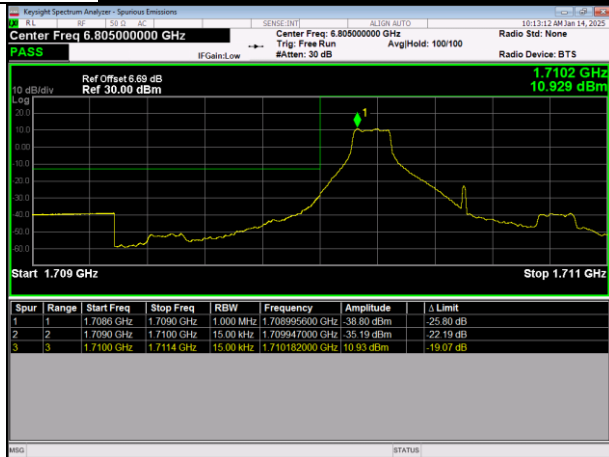
LTE Band4 64QAM BW=1.4MHz LowChannel=19957 RB Size=1 Position=#0
