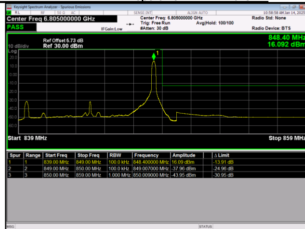
LTE Band5 64QAM BW=10MHz HighChannel=20600 RB Size=1 Position=#Max
