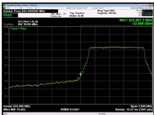
LTE Band5 16QAM BW=1.4MHz Channel=20407 RB Size=6 Position=#0
