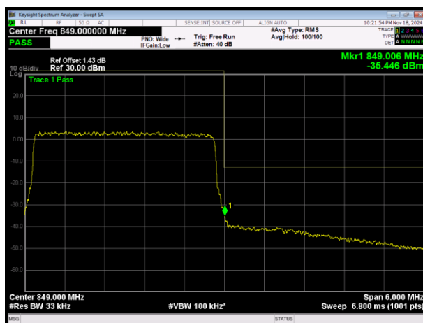
LTE Band5 16QAM BW=3MHz Channel=20635 RB Size=15 Position=#0
