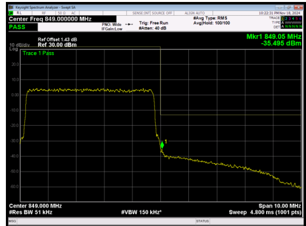
LTE Band5 QPSK BW=5MHz Channel=20625 RB Size=25 Position=#0
