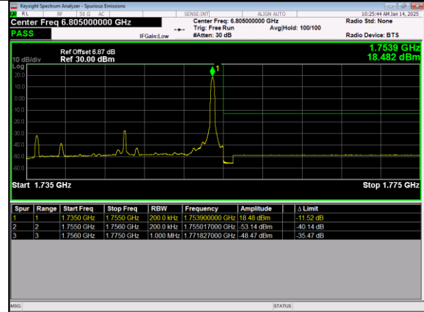
LTE Band4 64QAM BW=20MHz HighChannel=20300 RB Size=1 Position=#Max
