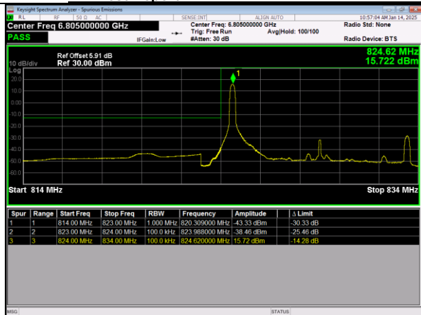
LTE Band5 64QAM BW=10MHz LowChannel=20450 RB Size=1 Position=#0
