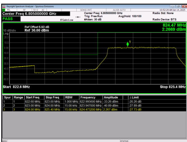
LTE Band5 64QAM BW=1.4MHz LowChannel=20407 RB Size=6 Position=#0
