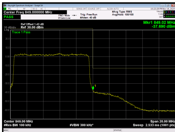
LTE Band5 16QAM BW=10MHz Channel=20600 RB Size=50 Position=#0
