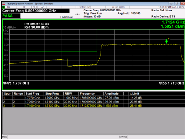
LTE Band4 64QAM BW=3MHz LowChannel=19965 RB Size=15 Position=#0
