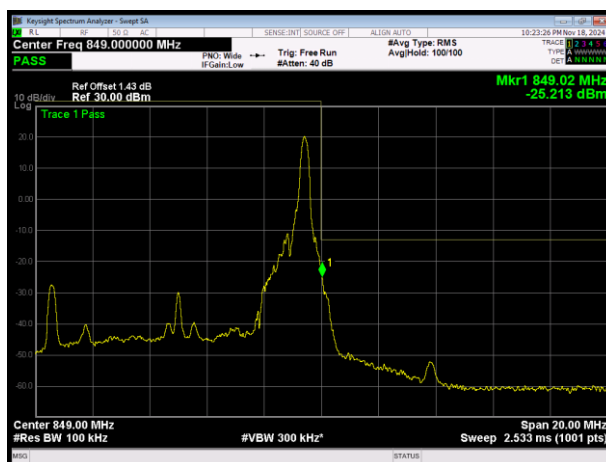
LTE Band5 16QAM BW=10MHz Channel=20600 RB Size=1 Position=#Max
