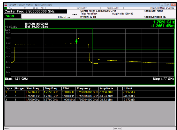
LTE Band4 64QAM BW=15MHz HighChannel=20325 RB Size=75 Position=#0
