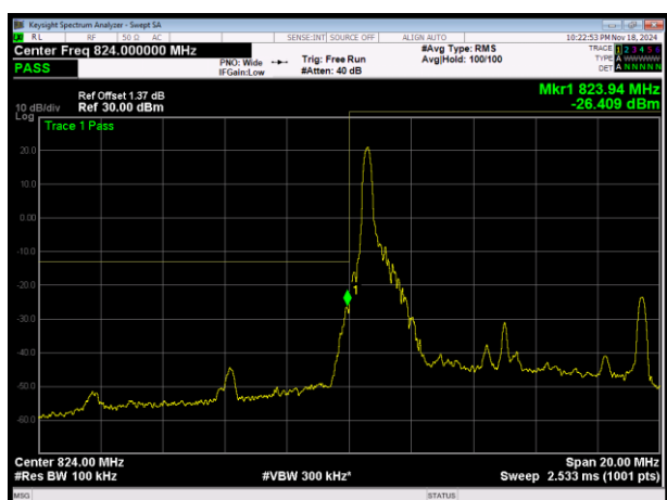
LTE Band5 QPSK BW=10MHz Channel=20450 RB Size=1 Position=#0
