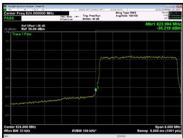
LTE Band5 16QAM BW=3MHz Channel=20415 RB Size=15 Position=#0
