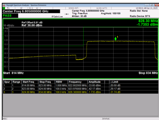
LTE Band5 64QAM BW=10MHz LowChannel=20450 RB Size=50 Position=#0
