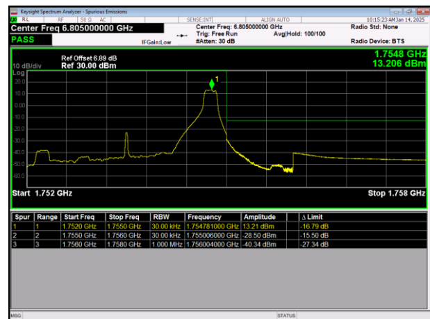
LTE Band4 64QAM BW=3MHz HighChannel=20385 RB Size=1 Position=#Max
