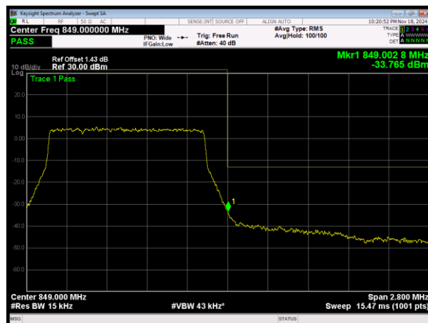
LTE Band5 QPSK BW=1.4MHz Channel=20643 RB Size=6 Position=#0
