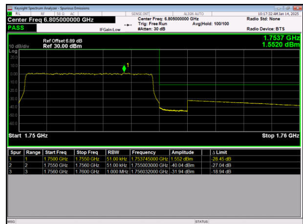
LTE Band4 64QAM BW=5MHz HighChannel=20375 RB Size=25 Position=#0
