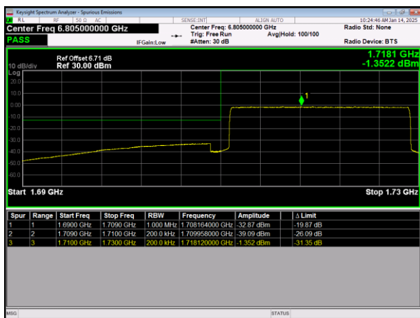
LTE Band4 64QAM BW=20MHz LowChannel=20050 RB Size=100 Position=#0
