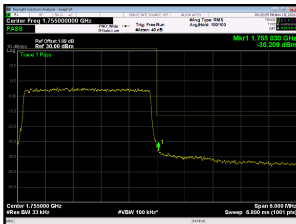
LTE Band4 QPSK BW=3MHz Channel=20385 RB Size=15 Position=#0
