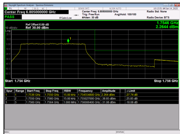
LTE Band4 64QAM BW=1.4MHz HighChannel=20393 RB Size=6 Position=#0
