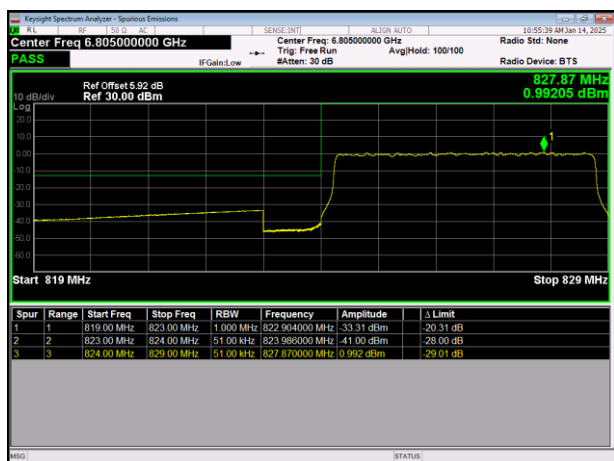
LTE Band5 64QAM BW=5MHz LowChannel=20425 RB Size=25 Position=#0
