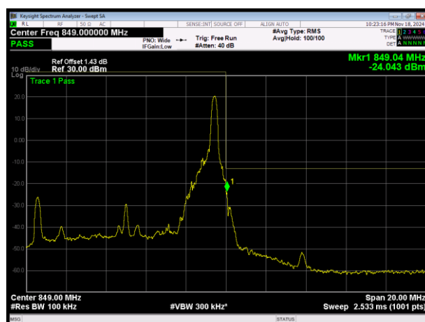
LTE Band5 QPSK BW=10MHz Channel=20600 RB Size=1 Position=#Max
