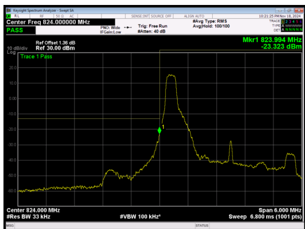
LTE Band5 16QAM BW=3MHz Channel=20415 RB Size=1 Position=#0
