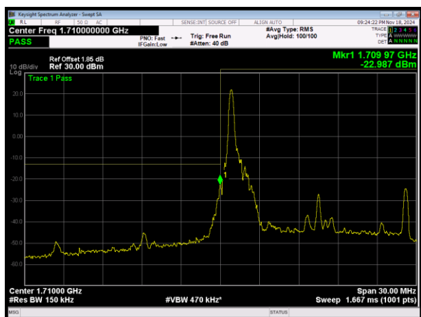
LTE Band4 QPSK BW=15MHz Channel=20025 RB Size=1 Position=#0
