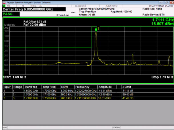
LTE Band4 64QAM BW=20MHz LowChannel=20050 RB Size=1 Position=#0
