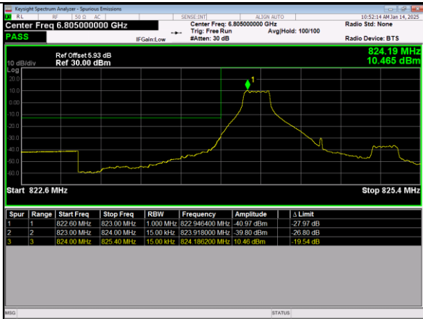
LTE Band5 64QAM BW=1.4MHz LowChannel=20407 RB Size=1 Position=#0
