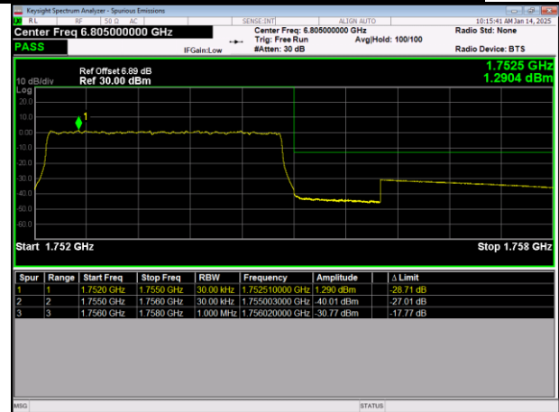
LTE Band4 64QAM BW=3MHz HighChannel=20385 RB Size=15 Position=#0
