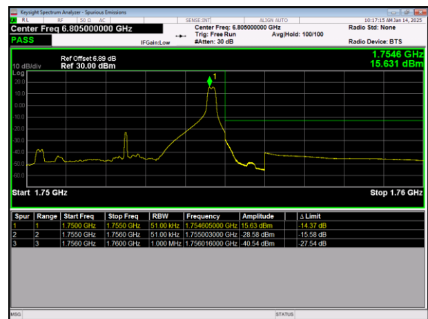
LTE Band4 64QAM BW=5MHz HighChannel=20375 RB Size=1 Position=#Max
