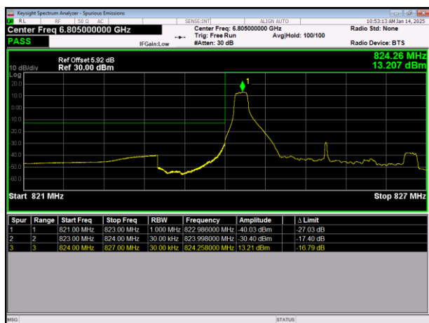
LTE Band5 64QAM BW=3MHz LowChannel=20415 RB Size=1 Position=#0
