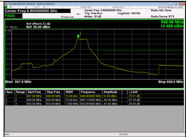
LTE Band5 64QAM BW=1.4MHz HighChannel=20643 RB Size=1 Position=#Max
