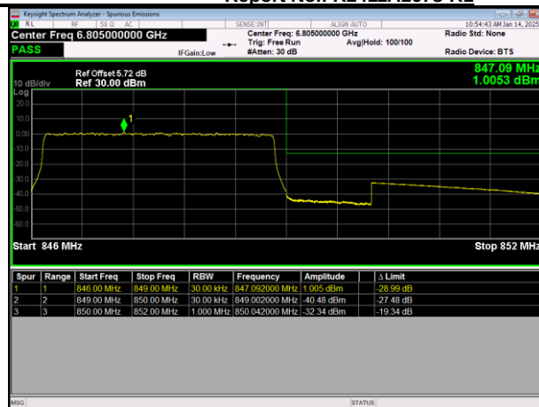
LTE Band5 64QAM BW=3MHz HighChannel=20635 RB Size=15 Position=#0
