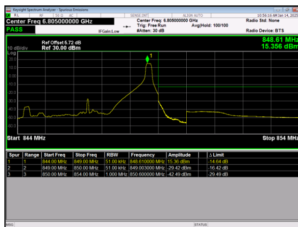
LTE Band5 64QAM BW=5MHz HighChannel=20625 RB Size=1 Position=#Max
