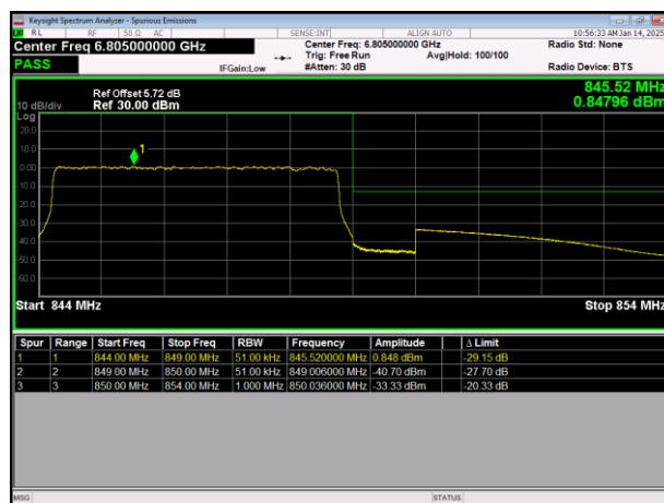
LTE Band5 64QAM BW=5MHz HighChannel=20625 RB Size=25 Position=#0
