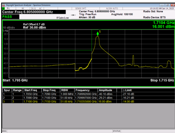
LTE Band4 64QAM BW=5MHz LowChannel=19975 RB Size=1 Position=#0
