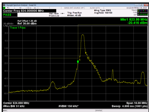
LTE Band5 QPSK BW=5MHz Channel=20425 RB Size=1 Position=#0
