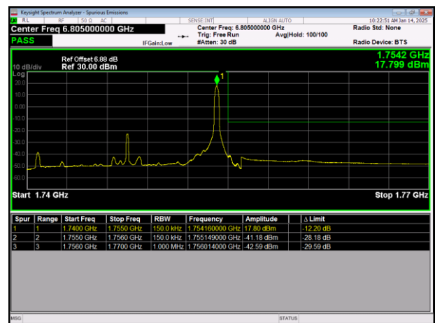
LTE Band4 64QAM BW=15MHz HighChannel=20325 RB Size=1 Position=#Max
