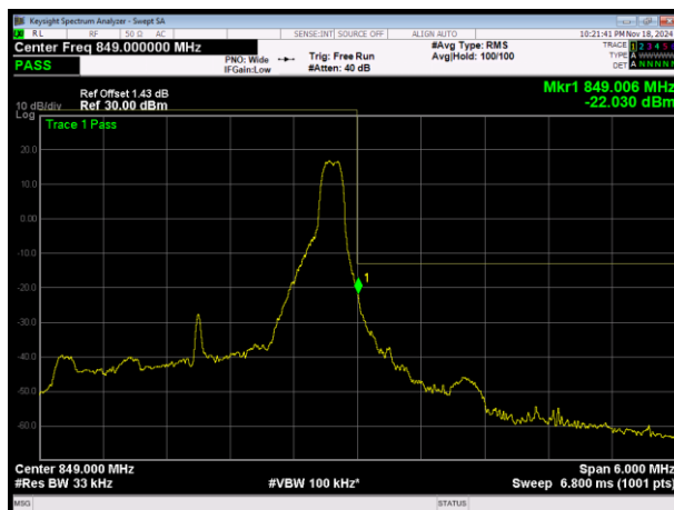
LTE Band5 QPSK BW=3MHz Channel=20635 RB Size=1 Position=#Max
