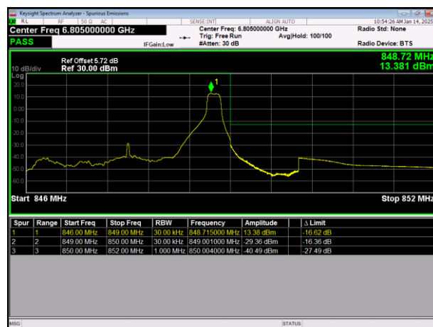
LTE Band5 64QAM BW=3MHz HighChannel=20635 RB Size=1 Position=#Max
