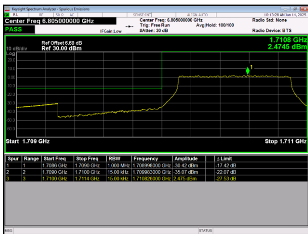
LTE Band4 64QAM BW=1.4MHz LowChannel=19957 RB Size=6 Position=#0
