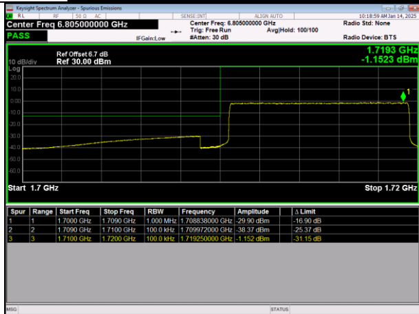
LTE Band4 64QAM BW=10MHz LowChannel=20000 RB Size=50 Position=#0
