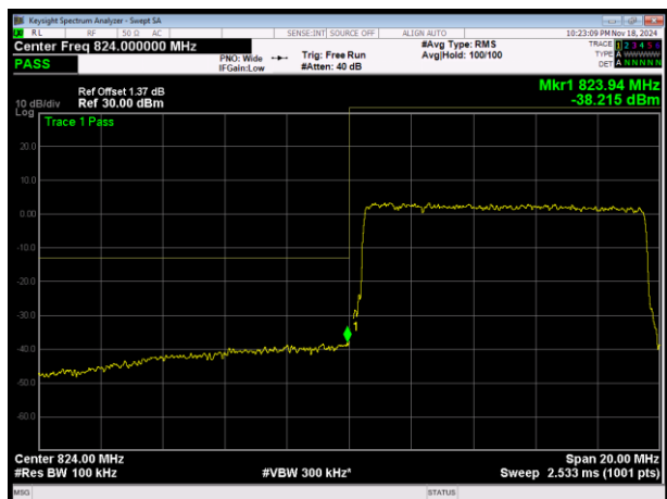
LTE Band5 16QAM BW=10MHz Channel=20450 RB Size=50 Position=#0
