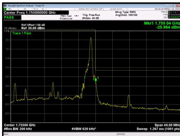
LTE Band4 QPSK BW=20MHz Channel=20300 RB Size=1 Position=#Max
