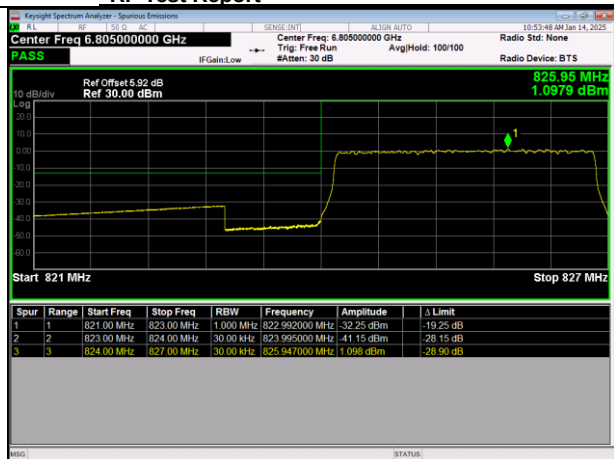
LTE Band5 64QAM BW=3MHz LowChannel=20415 RB Size=15 Position=#0
