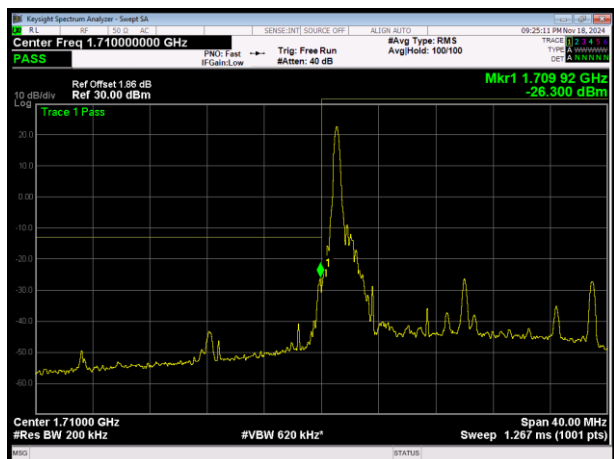
LTE Band4 QPSK BW=20MHz Channel=20050 RB Size=1 Position=#0
