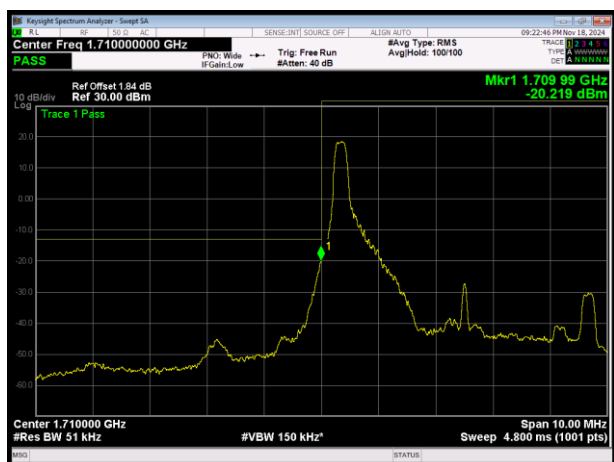
LTE Band4 QPSK BW=5MHz Channel=19975 RB Size=1 Position=#0
