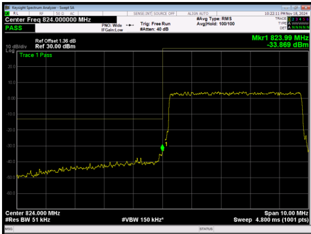
LTE Band5 QPSK BW=5MHz Channel=20425 RB Size=25 Position=#0
