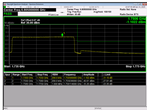
LTE Band4 64QAM BW=20MHz HighChannel=20300 RB Size=100 Position=#0
