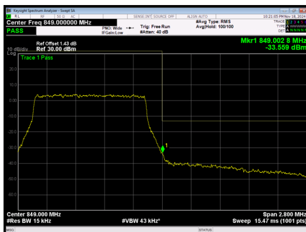
LTE Band5 16QAM BW=1.4MHz Channel=20643 RB Size=6 Position=#0
