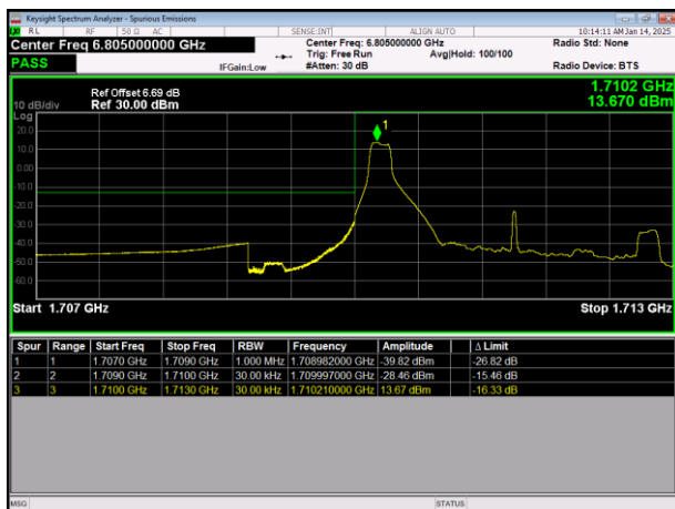
LTE Band4 64QAM BW=3MHz LowChannel=19965 RB Size=1 Position=#0
