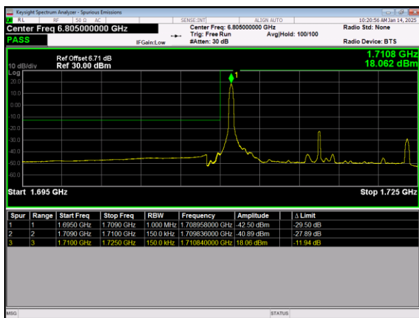
LTE Band4 64QAM BW=15MHz LowChannel=20025 RB Size=1 Position=#0
