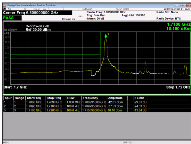
LTE Band4 64QAM BW=10MHz LowChannel=20000 RB Size=1 Position=#0
