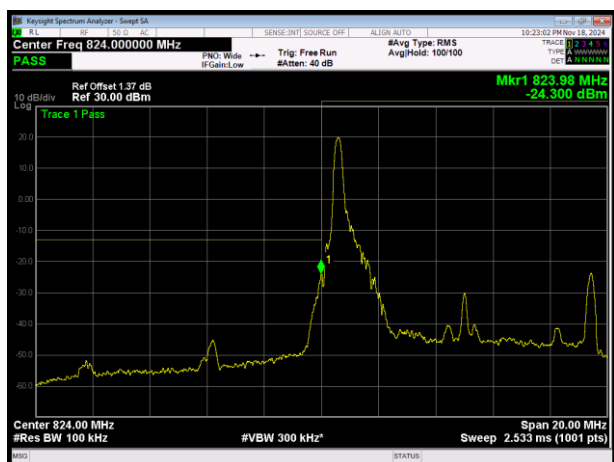
LTE Band5 16QAM BW=10MHz Channel=20450 RB Size=1 Position=#0
