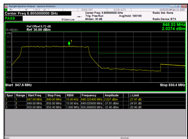
LTE Band5 64QAM BW=1.4MHz HighChannel=20643 RB Size=6 Position=#0
