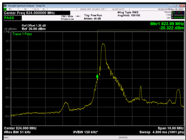
LTE Band5 16QAM BW=5MHz Channel=20425 RB Size=1 Position=#0
