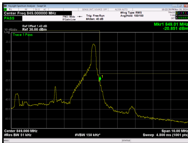
LTE Band5 16QAM BW=5MHz Channel=20625 RB Size=1 Position=#Max
