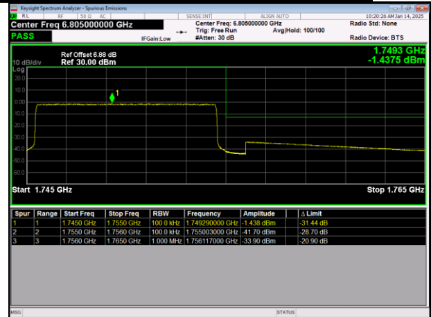
LTE Band4 64QAM BW=10MHz HighChannel=20350 RB Size=50 Position=#0
