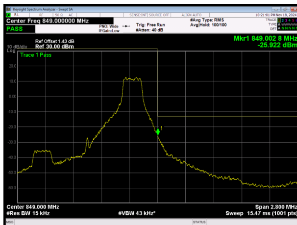
LTE Band5 16QAM BW=1.4MHz Channel=20643 RB Size=1 Position=#Max
