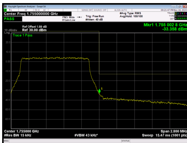
LTE Band4 16QAM BW=1.4MHz Channel=20393 RB Size=6 Position=#0
