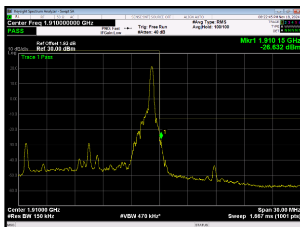
LTE Band2 QPSK BW=15MHz Channel=19125 RB Size=1 Position=#Max
