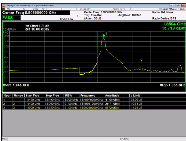
LTE Band2 64QAM BW=5MHz LowChannel=18625 RB Size=1 Position=#0
