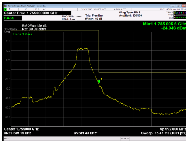
LTE Band4 16QAM BW=1.4MHz Channel=20393 RB Size=1 Position=#Max
