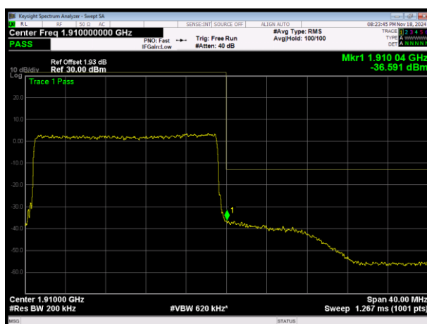
LTE Band2 16QAM BW=20MHz Channel=19100 RB Size=100 Position=#0
