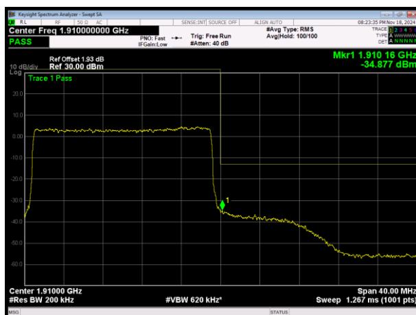
LTE Band2 QPSK BW=20MHz Channel=19100 RB Size=100 Position=#0
