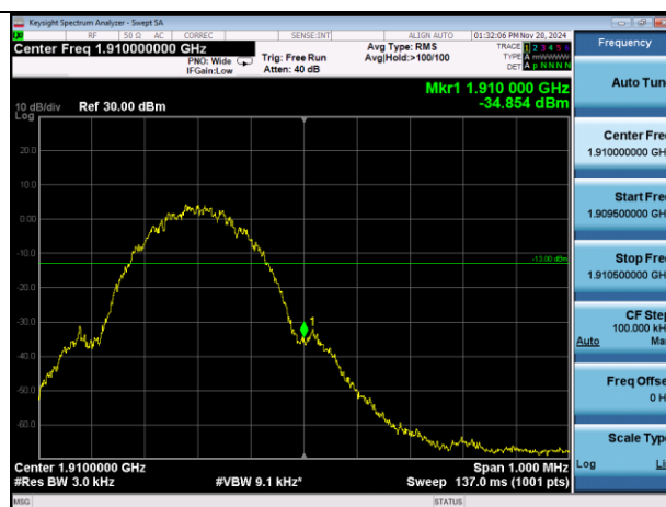
GPRS1900H
