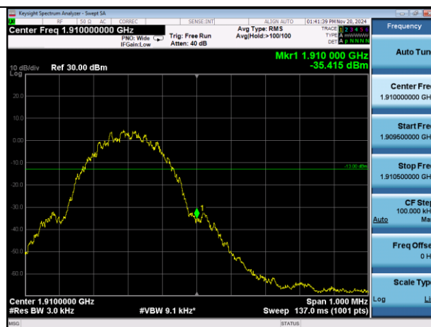
EGPRS1900H
