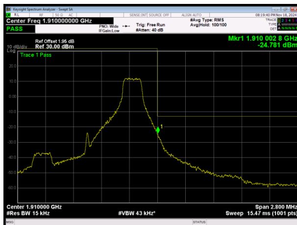
LTE Band2 16QAM BW=1.4MHz Channel=19193 RB Size=1 Position=#Max
