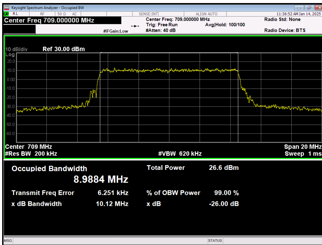
LTE Band17 64QAM BW=10MHz Channel=23780 RB Size=50 Position=#0
