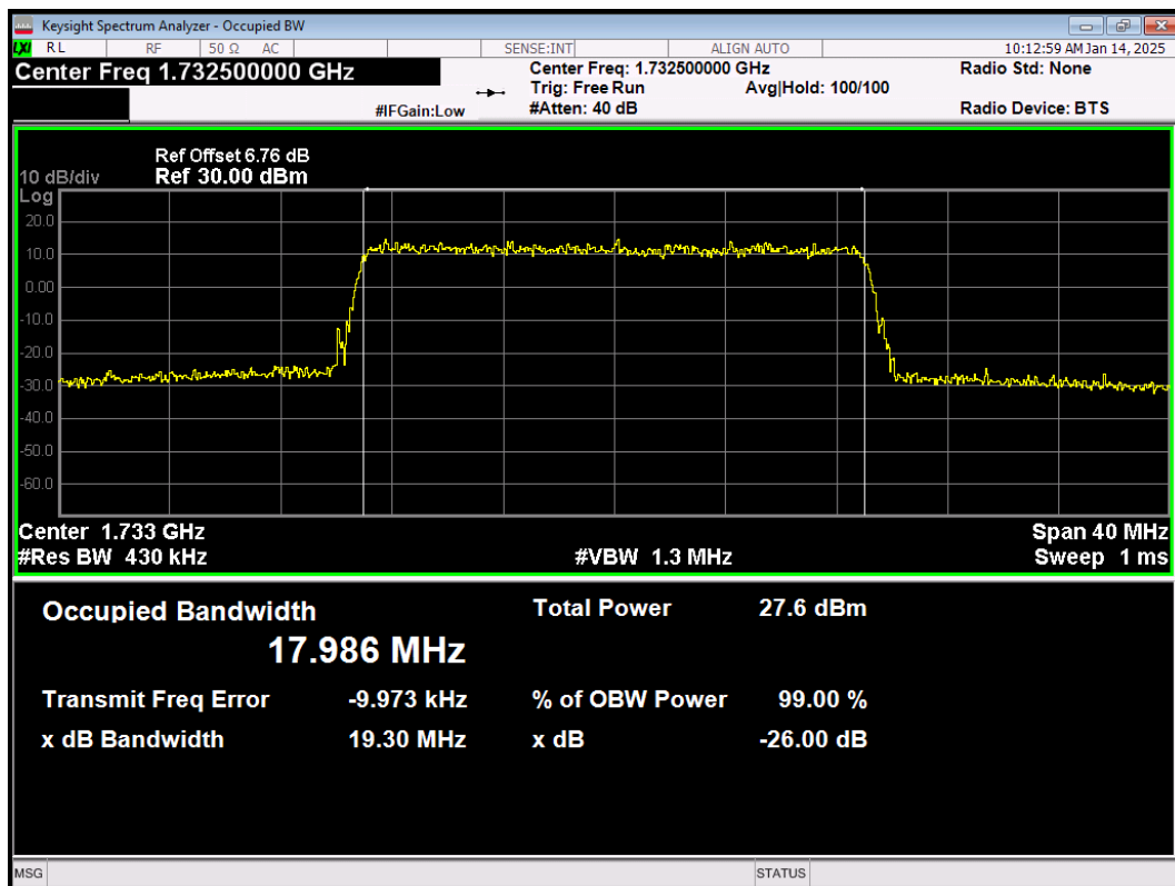
LTE Band4 64QAM BW=20MHz Channel=20175 RB Size=100 Position=#0
