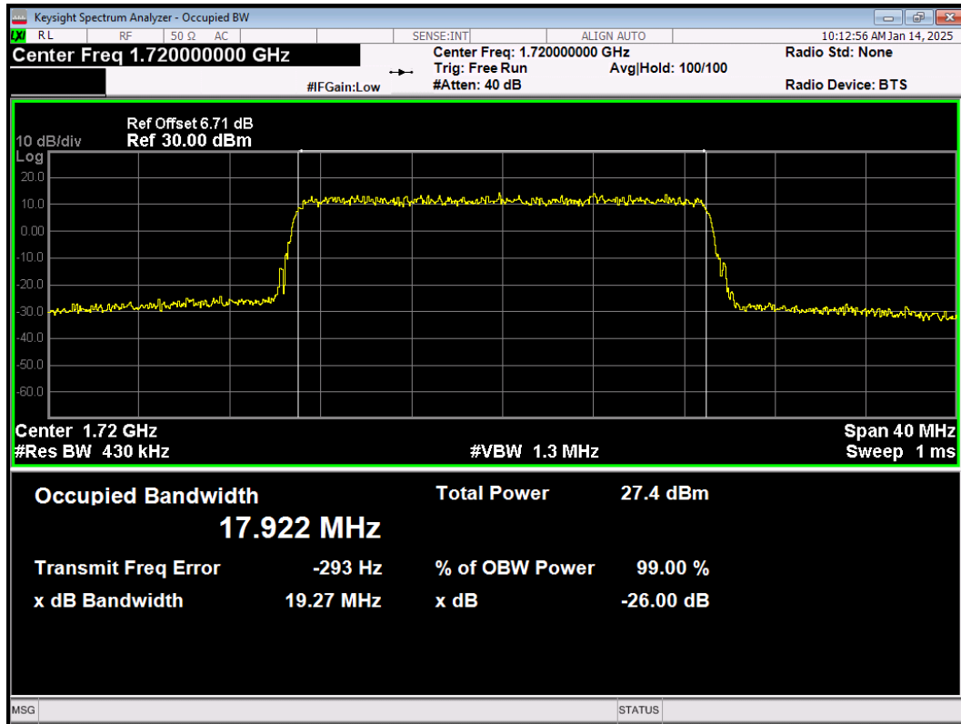
LTE Band4 64QAM BW=20MHz Channel=20050 RB Size=100 Position=#0
