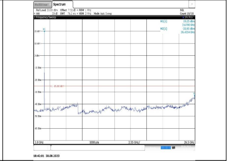
Band41-20MHz-16QAM-39750-1RB#0-Range2:1000~26500MHz
