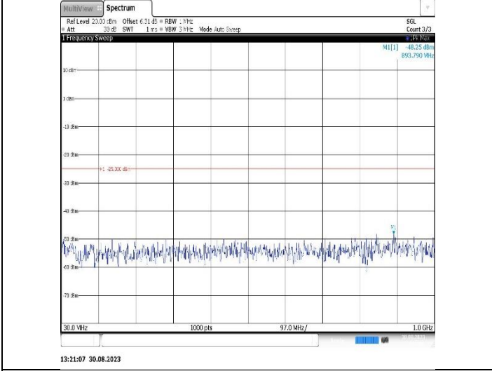
Band38-5MHz-16QAM-37775-1RB#0-Range1:30~1000MHz
