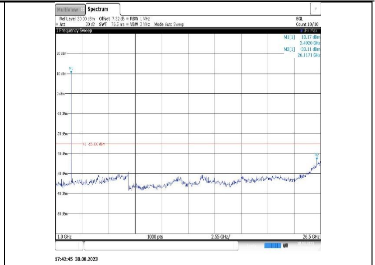
Band41-10MHz-16QAM-40620-1RB#0-Range2:1000~26500MHz
