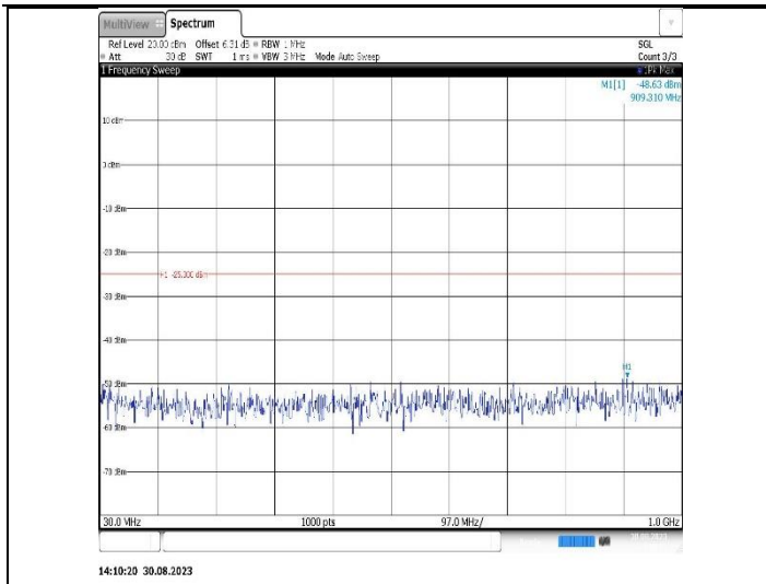
Band38-10MHz-QPSK-38000-1RB#0-Range1:30~1000MHz
