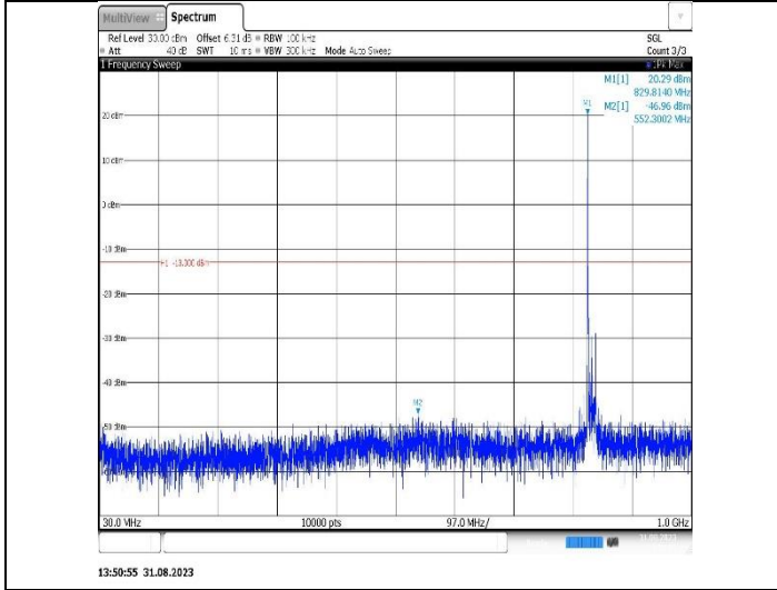
Band26(824-849)-15MHz-QPSK-26965-1RB#0-Range1:30~1000MHz
