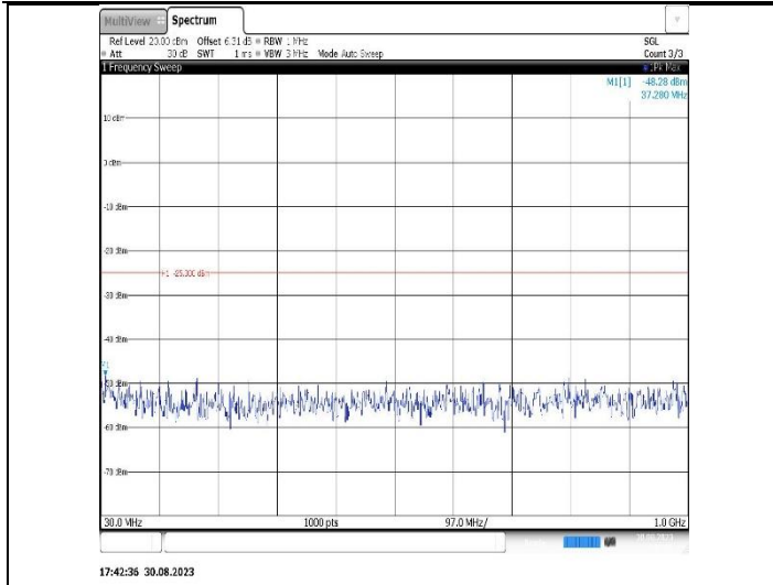
Band41-10MHz-16QAM-40620-1RB#0-Range1:30~1000MHz
