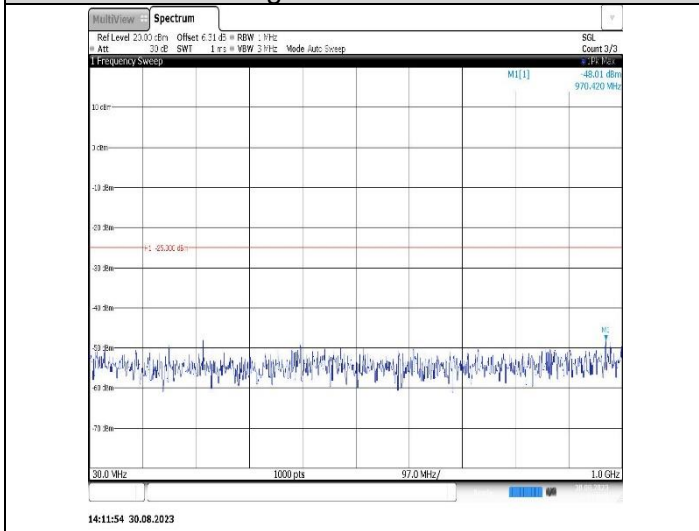
Band38-15MHz-QPSK-37825-1RB#0-Range1:30~1000MHz
