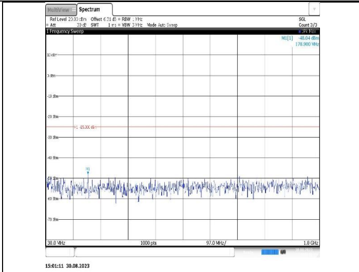
Band38-15MHz-16QAM-38000-1RB#0-Range1:30~1000MHz
