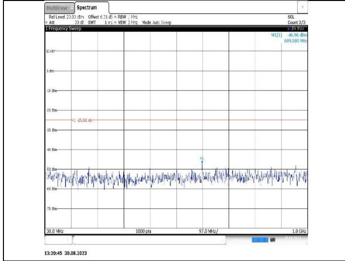
Band38-5MHz-16QAM-38225-1RB#0-Range1:30~1000MHz
