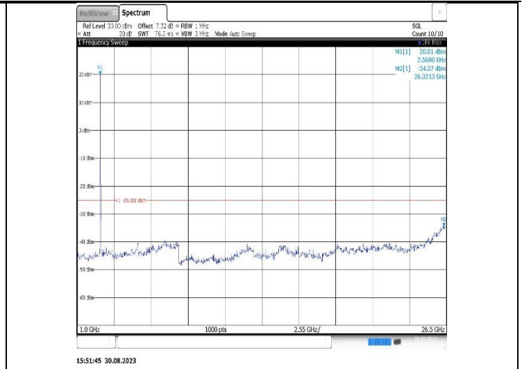
Band38-20MHz-16QAM-38000-1RB#0-Range2:1000~26500MHz
