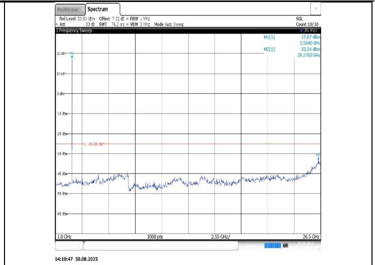
Band38-10MHz-16QAM-38000-1RB#0-Range2:1000~26500MHz
