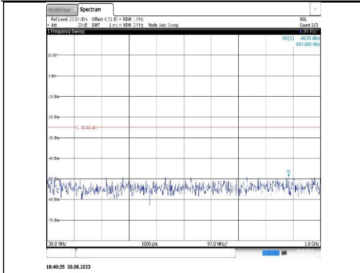
Band41-20MHz-QPSK-40620-1RB#0-Range1:30~1000MHz
