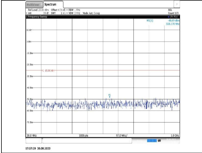
Band41-15MHz-QPSK-41515-1RB#0-Range1:30~1000MHz
