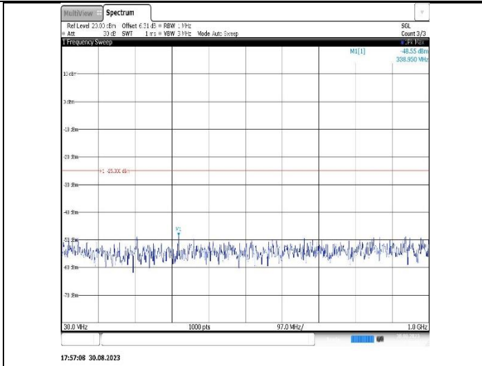
Band41-15MHz-16QAM-40620-1RB#0-Range1:30~1000MHz
