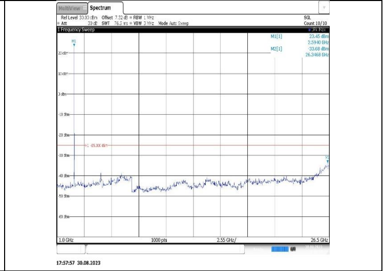
Band41-15MHz-16QAM-41515-1RB#0-Range2:1000~26500MHz
