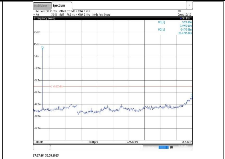
Band41-15MHz-16QAM-40620-1RB#0-Range2:1000~26500MHz
