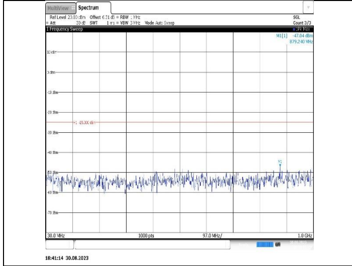
Band41-20MHz-QPSK-41490-1RB#0-Range1:30~1000MHz
