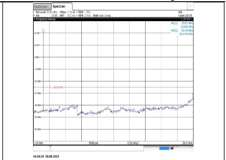
Band38-10MHz-QPSK-38000-1RB#0-Range2:1000~26500MHz
