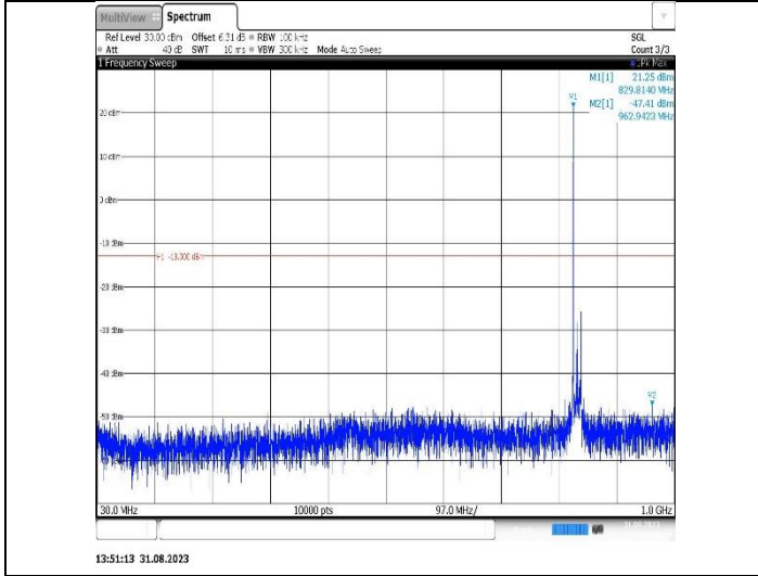
Band26(824-849)-15MHz-16QAM-26965-1RB#0-Range1:30~1000MHz
