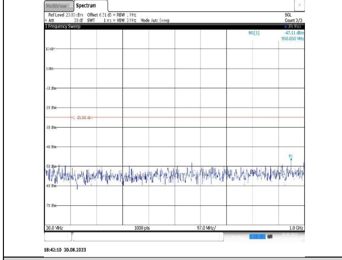
Band66-1.4MHz-QPSK-131979-1RB#0-Range1:30~1000MHz
