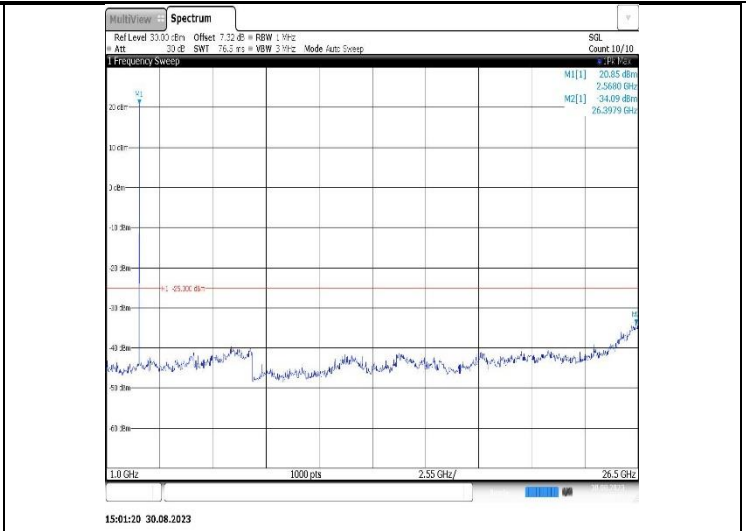
Band38-15MHz-16QAM-38000-1RB#0-Range2:1000~26500MHz
