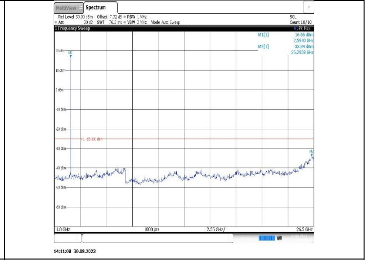
Band38-10MHz-QPSK-38200-1RB#0-Range2:1000~26500MHz
