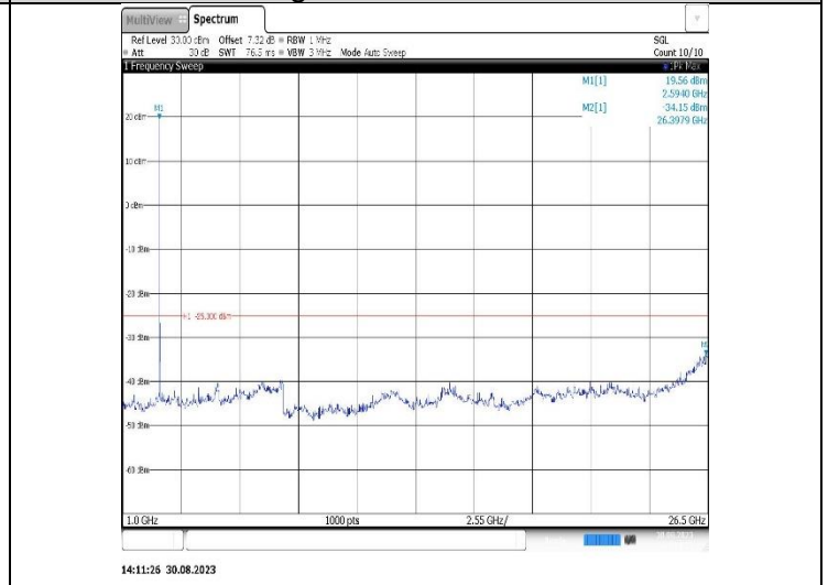
Band38-10MHz-16QAM-38200-1RB#0-Range2:1000~26500MHz
