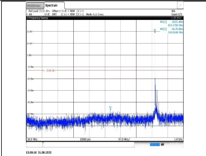
Band26(824-849)-15MHz-QPSK-26915-1RB#0-Range1:30~1000MHz
