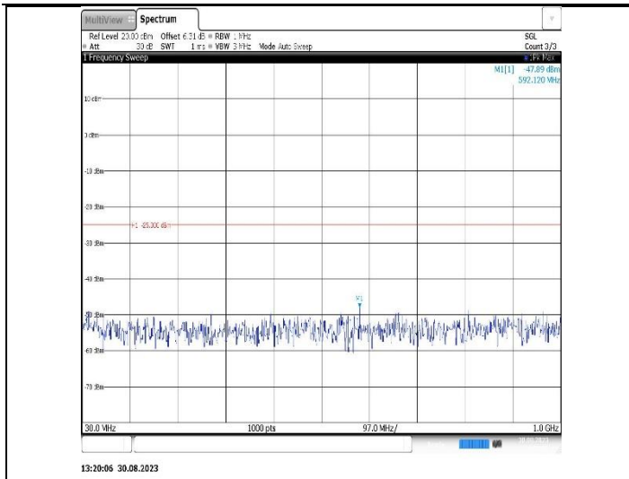
Band38-5MHz-16QAM-38000-1RB#0-Range1:30~1000MHz
