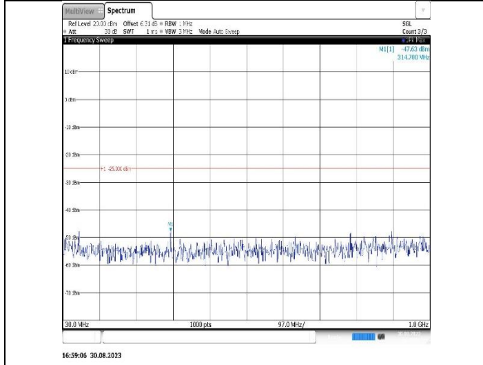
Band41-5MHz-QPSK-41565-1RB#0-Range1:30~1000MHz
