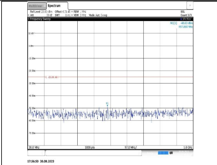
Band41-15MHz-QPSK-40620-1RB#0-Range1:30~1000MHz
