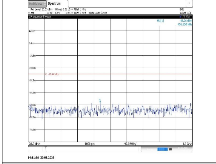
Band38-10MHz-16QAM-37800-1RB#0-Range1:30~1000MHz
