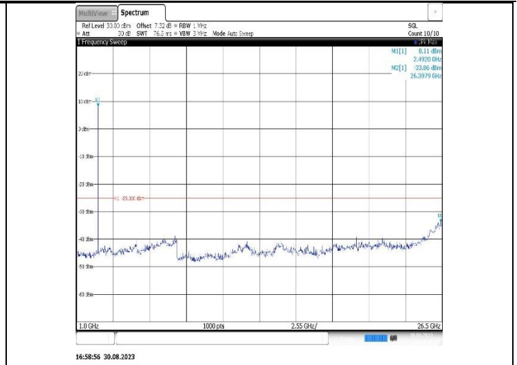
Band41-5MHz-16QAM-40620-1RB#0-Range2:1000~26500MHz
