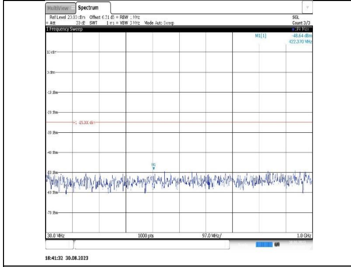
Band41-20MHz-16QAM-41490-1RB#0-Range1:30~1000MHz
