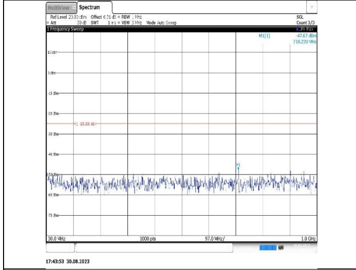
Band41-15MHz-QPSK-39725-1RB#0-Range1:30~1000MHz
