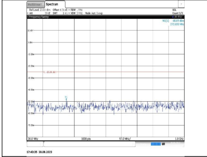
Band41-10MHz-16QAM-39700-1RB#0-Range1:30~1000MHz
