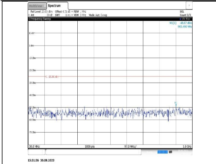
Band38-20MHz-16QAM-38000-1RB#0-Range1:30~1000MHz
