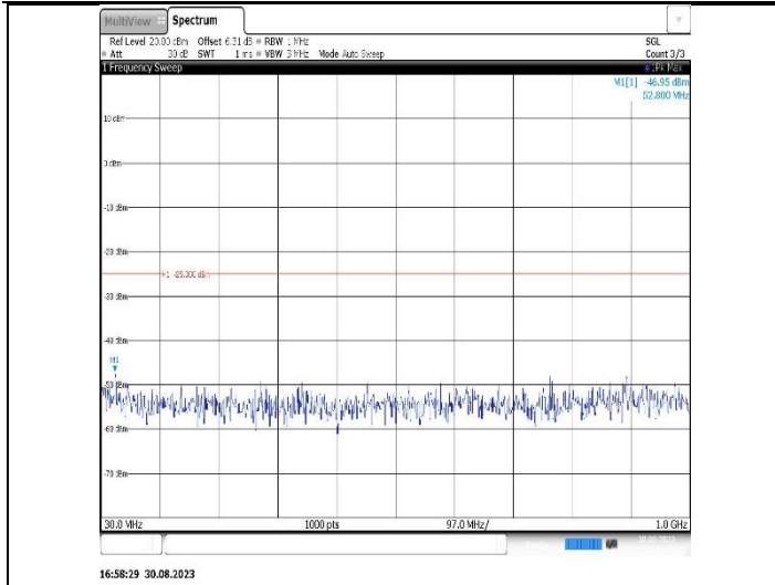
Band41-5MHz-QPSK-40620-1RB#0-Range1:30~1000MHz
