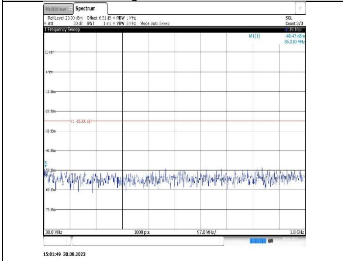
Band38-15MHz-16QAM-38175-1RB#0-Range1:30~1000MHz
