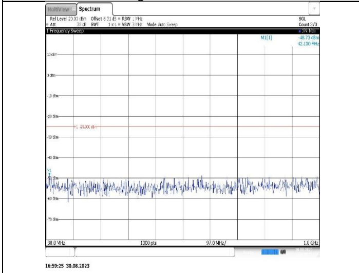
Band41-5MHz-16QAM-41565-1RB#0-Range1:30~1000MHz
