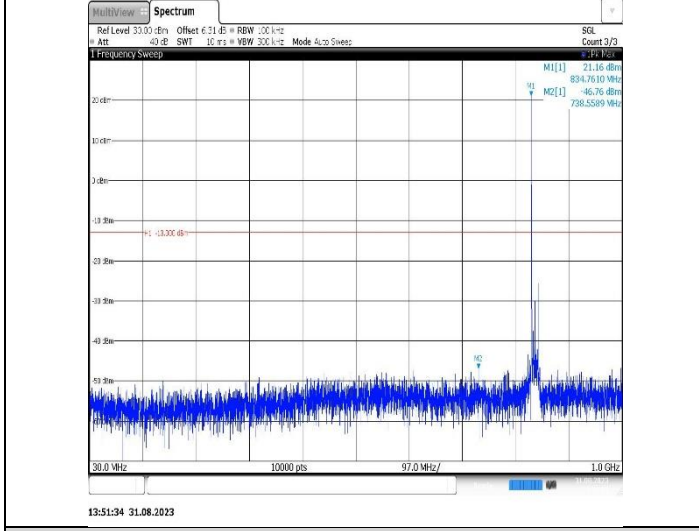
Band26(824-849)-15MHz-16QAM-26865-1RB#0-Range1:30~1000MHz
