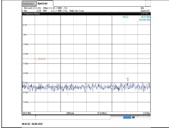
Band41-20MHz-16QAM-39750-1RB#0-Range1:30~1000MHz
