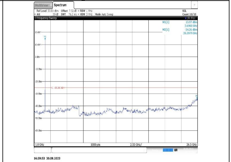
Band41-5MHz-16QAM-39675-1RB#0-Range2:1000~26500MHz
