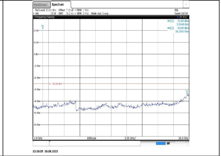
Band38-5MHz-16QAM-38225-1RB#0-Range2:1000~26500MHz
