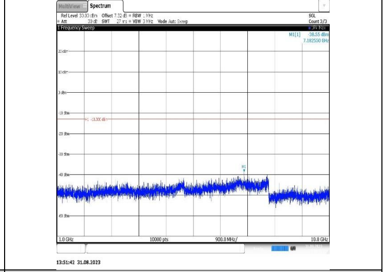
Band26(824-849)-15MHz-16QAM-26865-1RB#0-Range2:1000~10000MHz
