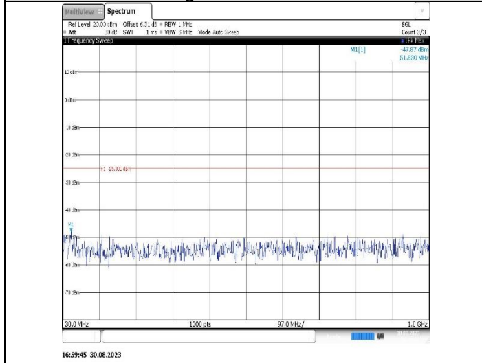
Band41-5MHz-16QAM-39675-1RB#0-Range1:30~1000MHz
