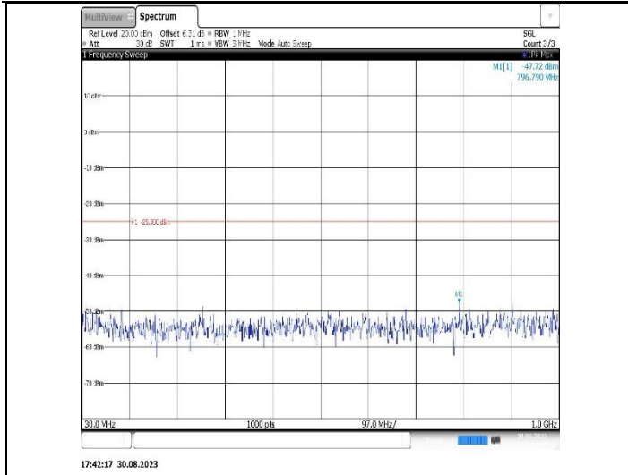
Band41-10MHz-QPSK-40620-1RB#0-Range1:30~1000MHz
