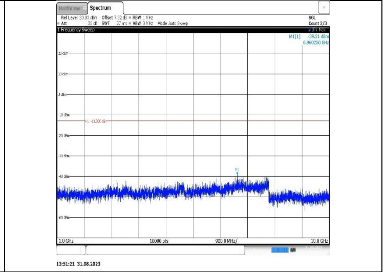
Band26(824-849)-15MHz-16QAM-26965-1RB#0-Range2:1000~10000MHz
