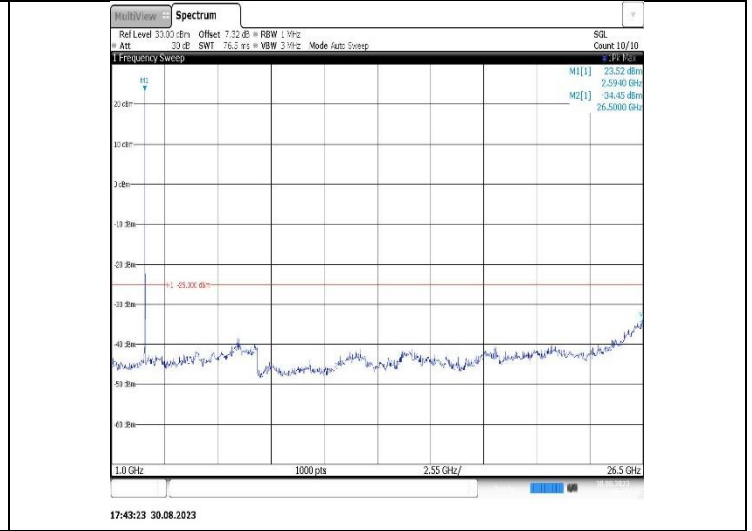
Band41-10MHz-16QAM-41540-1RB#0-Range2:1000~26500MHz
