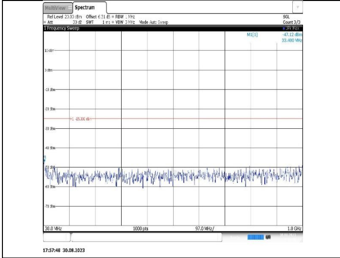
Band41-15MHz-16QAM-41515-1RB#0-Range1:30~1000MHz
