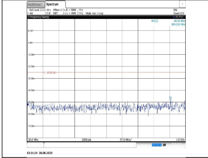
Band38-10MHz-QPSK-37800-1RB#0-Range1:30~1000MHz
