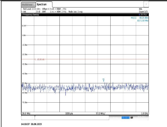
Band38-10MHz-16QAM-38000-1RB#0-Range1:30~1000MHz
