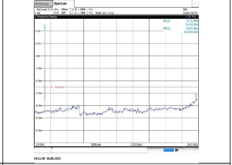
Band38-10MHz-16QAM-37800-1RB#0-Range2:1000~26500MHz
