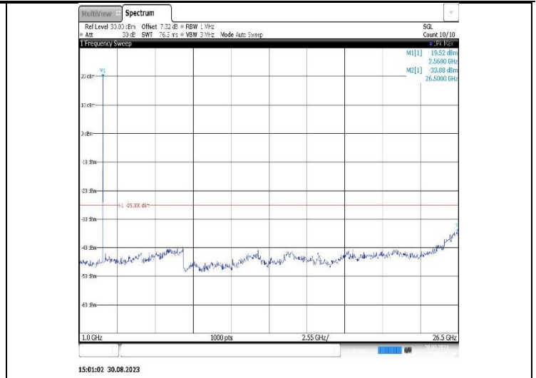
Band38-15MHz-QPSK-38000-1RB#0-Range2:1000~26500MHz
