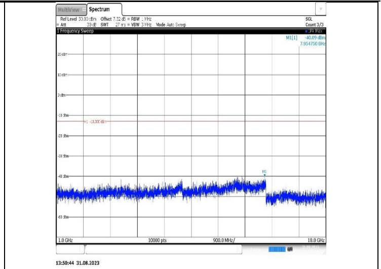
Band26(824-849)-15MHz-16QAM-26915-1RB#0-Range2:1000~10000MHz
