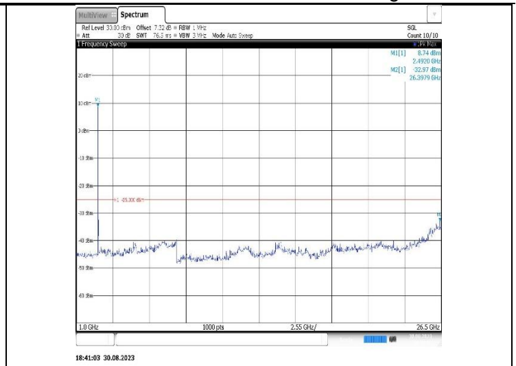
Band41-20MHz-16QAM-40620-1RB#0-Range2:1000~26500MHz
