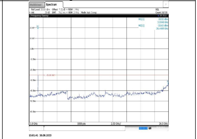
Band38-15MHz-QPSK-38175-1RB#0-Range2:1000~26500MHz
