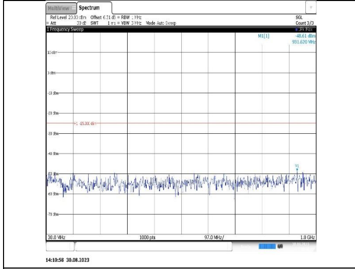
Band38-10MHz-QPSK-38200-1RB#0-Range1:30~1000MHz
