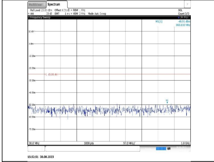
Band41-5MHz-QPSK-39675-1RB#0-Range1:30~1000MHz
