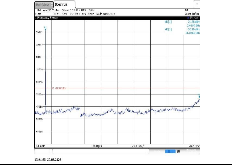
Band38-10MHz-QPSK-37800-1RB#0-Range2:1000~26500MHz
