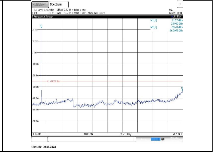
Band41-20MHz-16QAM-41490-1RB#0-Range2:1000~26500MHz
