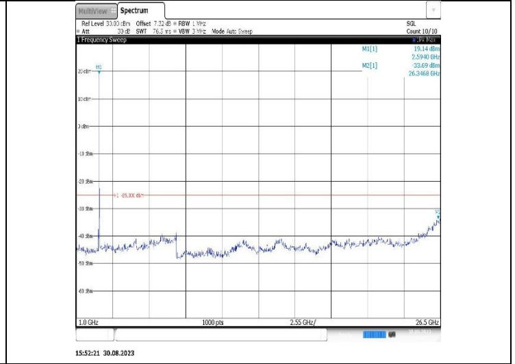
Band38-20MHz-16QAM-38150-1RB#0-Range2:1000~26500MHz
