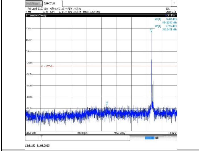
.Band38-5MHz-QPSK-37775-1RB#0-Range1:30~1000MHz
