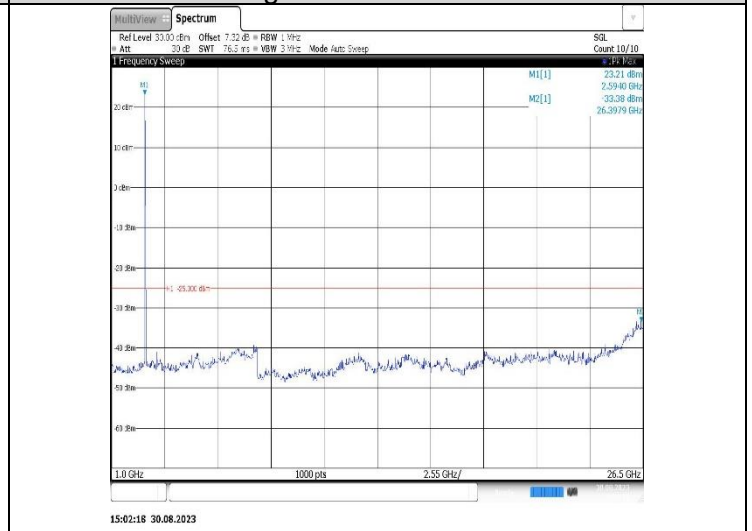
Band38-15MHz-16QAM-37825-1RB#0-Range2:1000~26500MHz
