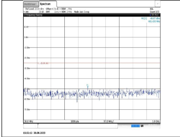
Band38-20MHz-16QAM-38150-1RB#0-Range1:30~1000MHz
