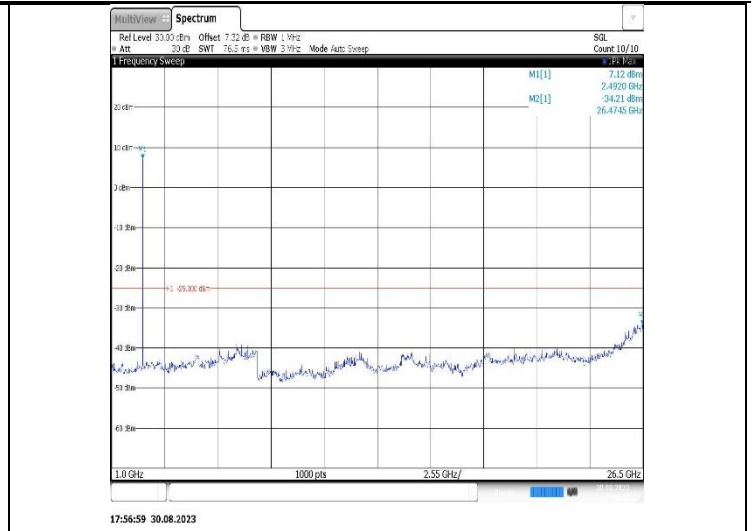
Band41-15MHz-QPSK-40620-1RB#0-Range2:1000~26500MHz
