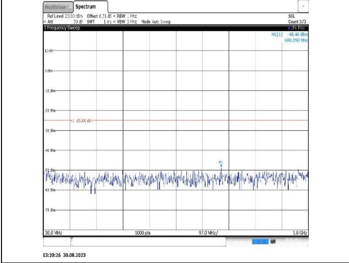
Band38-5MHz-QPSK-38225-1RB#0-Range1:30~1000MHz
