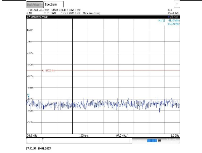
Band41-10MHz-QPSK-41540-1RB#0-Range1:30~1000MHz
