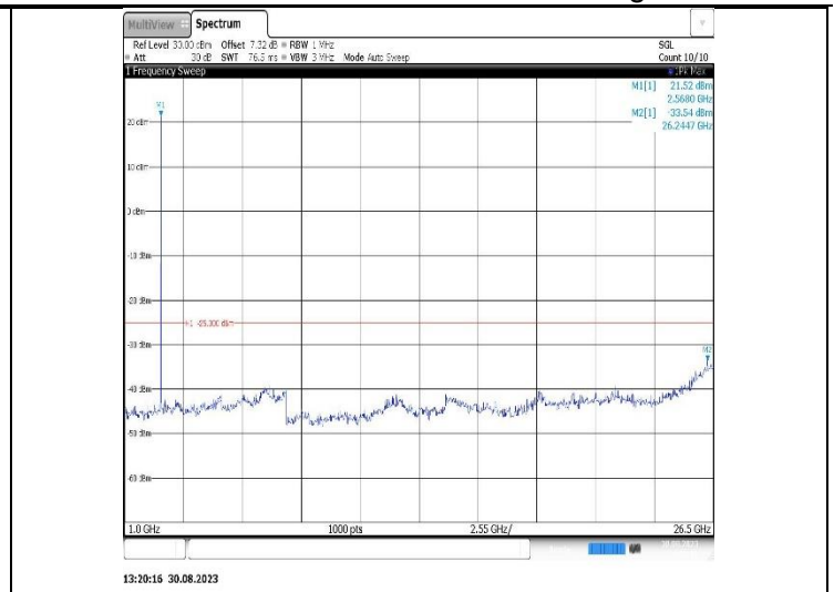
Band38-5MHz-16QAM-38000-1RB#0-Range2:1000~26500MHz
