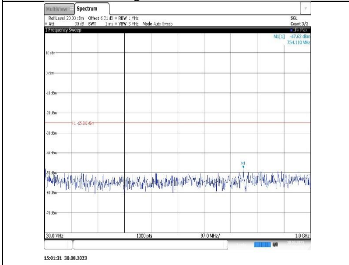
Band38-15MHz-QPSK-38175-1RB#0-Range1:30~1000MHz
