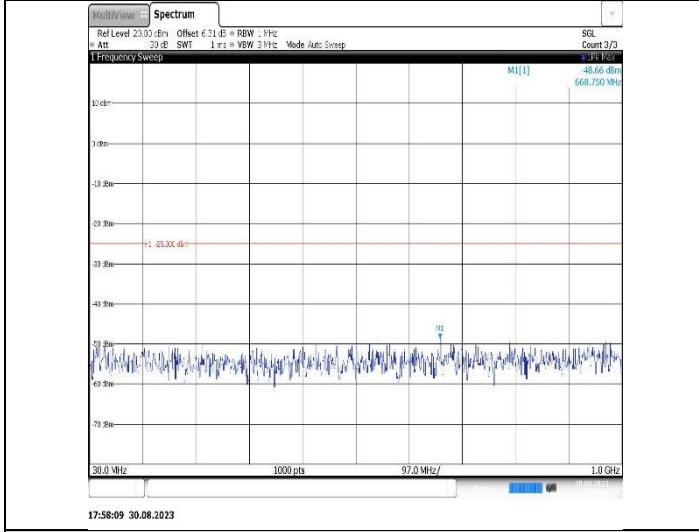
Band41-15MHz-16QAM-39725-1RB#0-Range1:30~1000MHz
