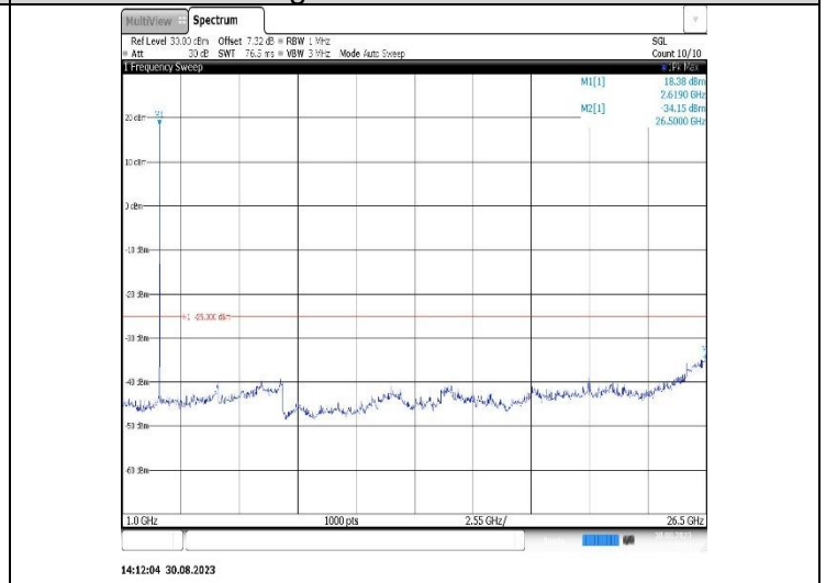
Band38-15MHz-QPSK-37825-1RB#0-Range2:1000~26500MHz
