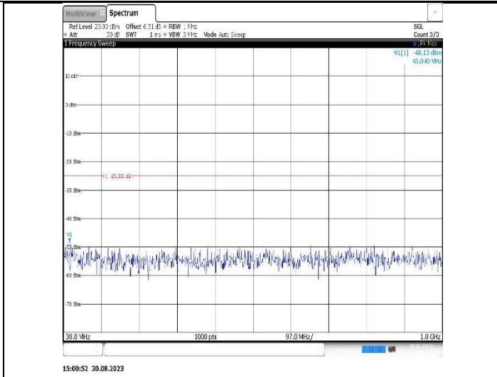
Band38-15MHz-QPSK-38000-1RB#0-Range1:30~1000MHz
