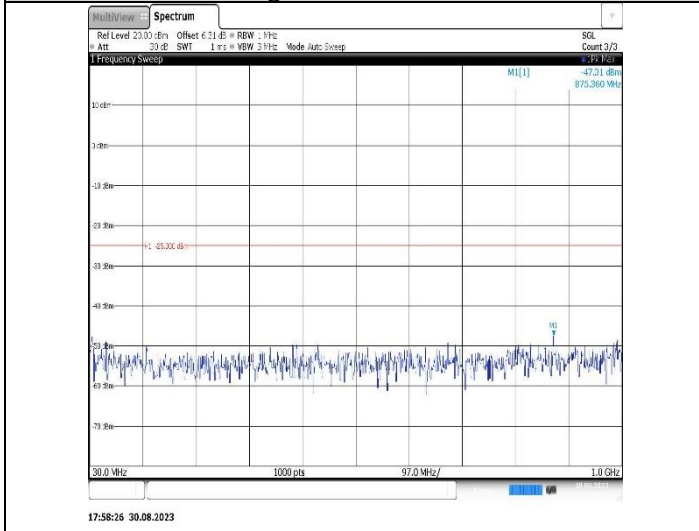
Band41-20MHz-QPSK-39750-1RB#0-Range1:30~1000MHz
