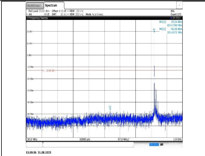
Band26(824-849)-15MHz-16QAM-26915-1RB#0-Range1:30~1000MHz
