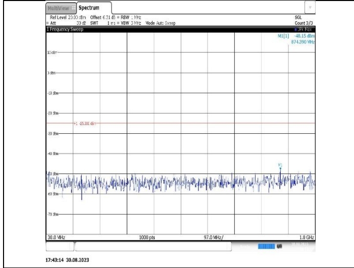
Band41-10MHz-16QAM-41540-1RB#0-Range1:30~1000MHz
