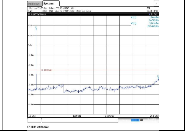
Band41-10MHz-16QAM-39700-1RB#0-Range2:1000~26500MHz
