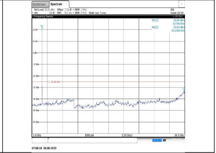
Band41-15MHz-16QAM-39725-1RB#0-Range2:1000~26500MHz
