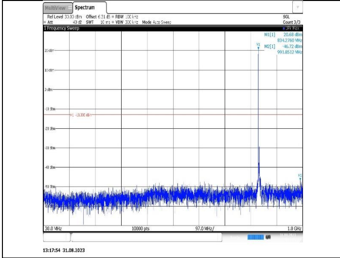
Band26(824-849)-5MHz-16QAM-27015-1RB#0-Range1:30~1000MHz
