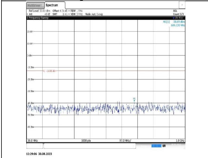
Band25-20MHz-16QAM-26365-1RB#0-Range1:30~1000MHz
