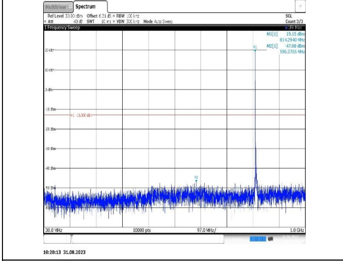
Band26(814-824)-5MHz-16QAM-26740-1RB#0-Range1:30~1000MHz
