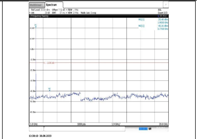
Band25-20MHz-16QAM-26140-1RB#0-Range2:1000~20000MHz
