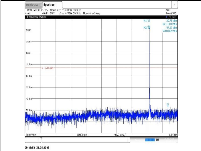
Band26(814-824)-5MHz-QPSK-26715-1RB#0-Range1:30~1000MHz
