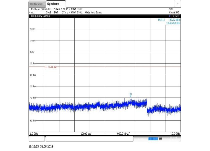
Band26(814-824)-5MHz-QPSK-26740-1RB#0-Range2:1000~10000MHz
