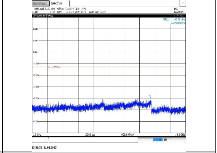
Band26(824-849)-10MHz-16QAM-26840-1RB#0-Range2:1000~10000MHz
