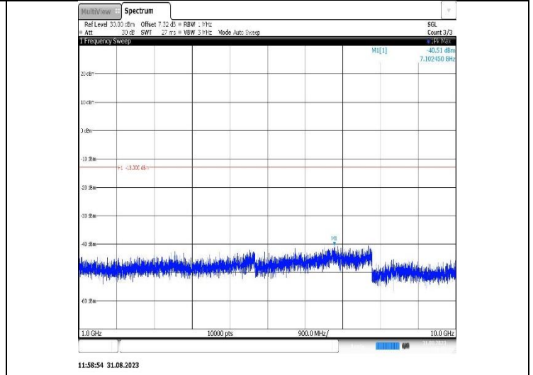
Band26(824-849)-1.4MHz-16QAM-27033-1RB#0-Range2:1000~10000MHz
