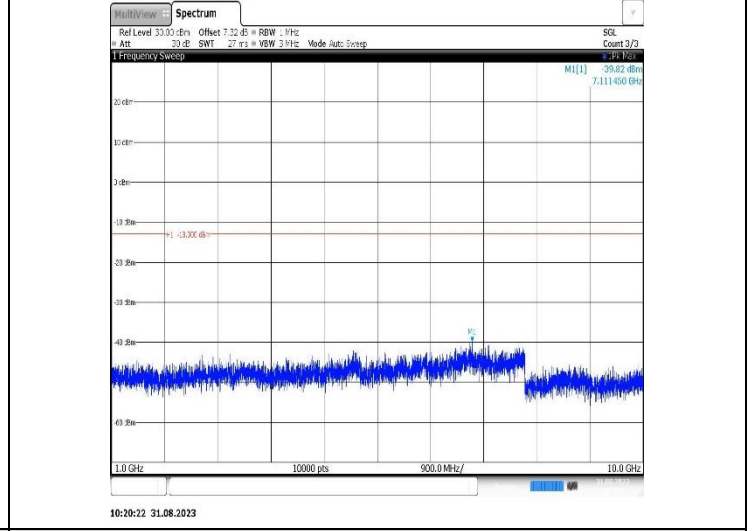
Band26(814-824)-5MHz-16QAM-26740-1RB#0-Range2:1000~10000MHz
