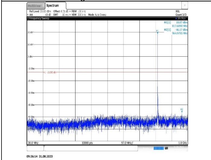
Band26(814-824)-3MHz-16QAM-26775-1RB#0-Range1:30~1000MHz
