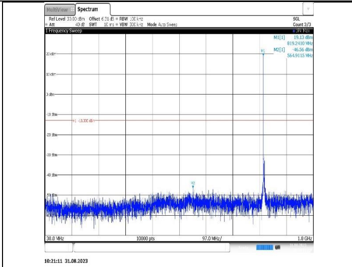
Band26(814-824)-5MHz-16QAM-26715-1RB#0-Range1:30~1000MHz
