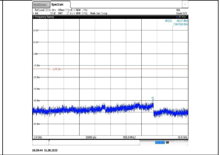
Band26(814-824)-10MHz-16QAM-26740-1RB#0-Range2:1000~10000MHz
