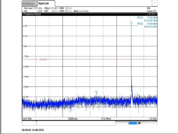
Band26(814-824)-5MHz-QPSK-26740-1RB#0-Range1:30~1000MHz
