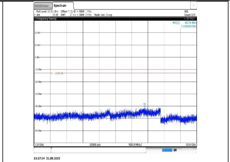
Band26(824-849)-5MHz-16QAM-26915-1RB#0-Range2:1000~10000MHz
