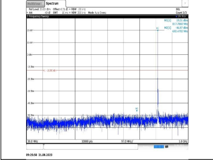
Band26(814-824)-3MHz-QPSK-26775-1RB#0-Range1:30~1000MHz
