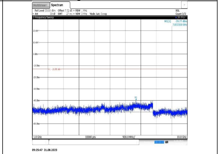
Band26(814-824)-3MHz-16QAM-26740-1RB#0-Range2:1000~10000MHz
