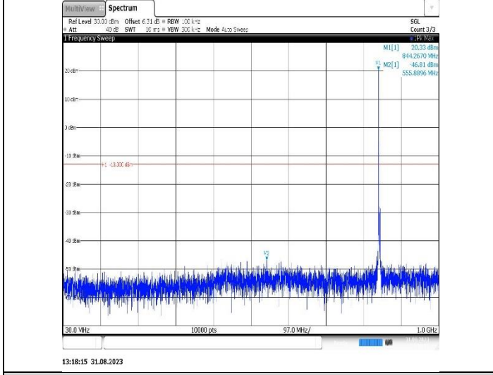
Band26(824-849)-5MHz-16QAM-26815-1RB#0-Range1:30~1000MHz
