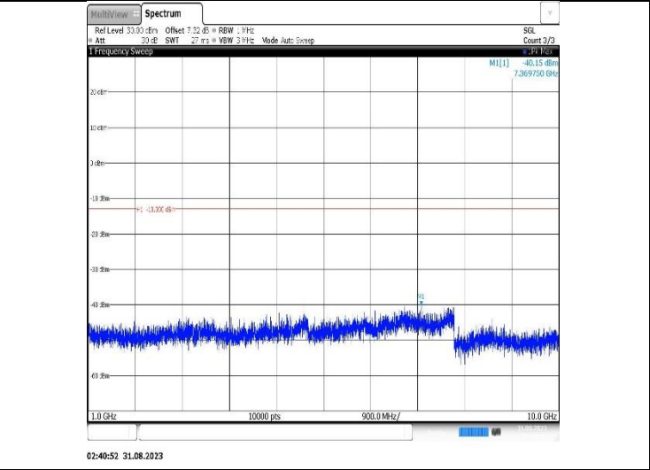
Band26(814-824)-1.4MHz-QPSK-26740-1RB#0-Range2:1000~10000MHz
