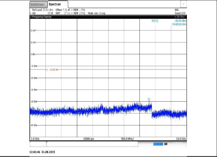
Band26(824-849)-3MHz-16QAM-26805-1RB#0-Range2:1000~10000MHz
