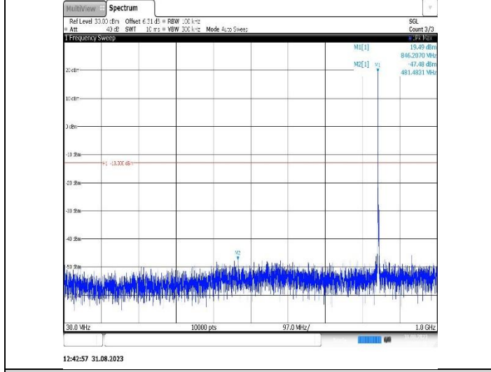
Band26(824-849)-5MHz-QPSK-26815-1RB#0-Range1:30~1000MHz
