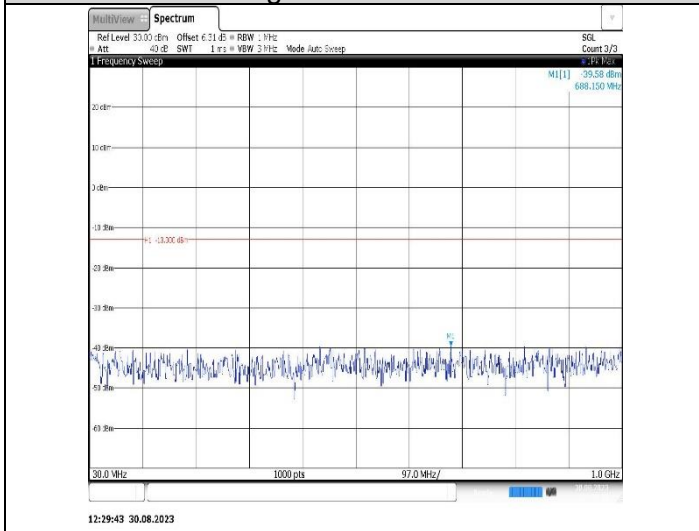
Band25-20MHz-16QAM-26590-1RB#0-Range1:30~1000MHz
