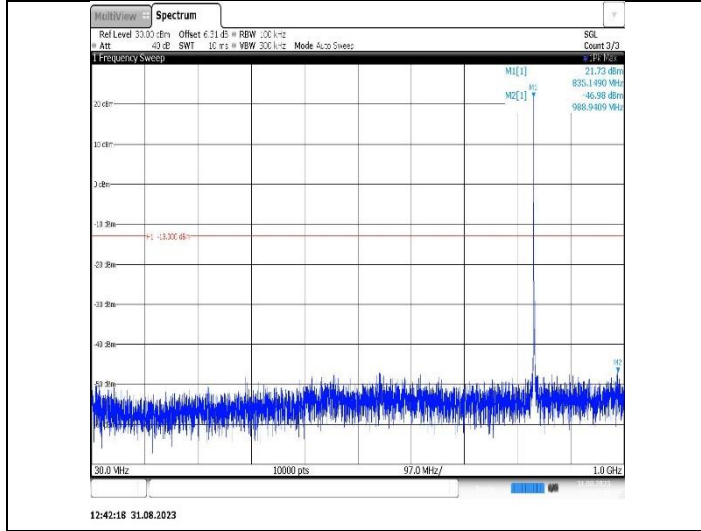
Band26(824-849)-3MHz-16QAM-27025-1RB#0-Range1:30~1000MHz
