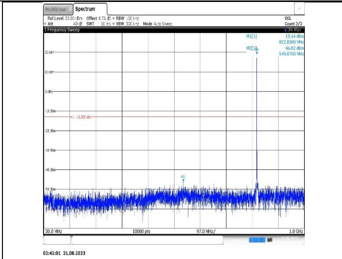
Band26(814-824)-1.4MHz-16QAM-26697-1RB#0-Range1:30~1000MHz
