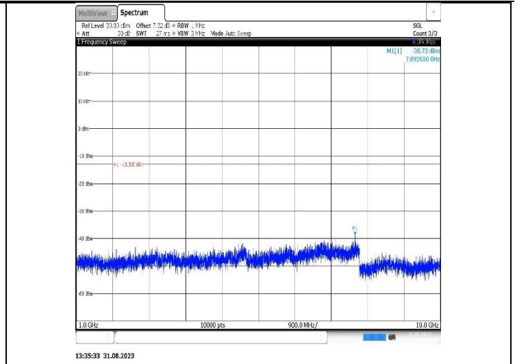
Band26(824-849)-10MHz-16QAM-26915-1RB#0-Range2:1000~10000MHz
