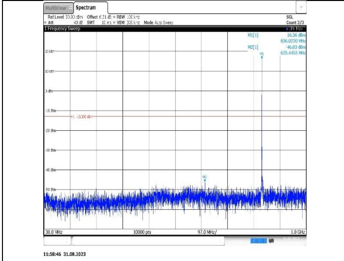
Band26(824-849)-1.4MHz-16QAM-27033-1RB#0-Range1:30~1000MHz
