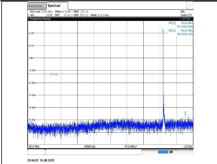
Band26(824-849)-5MHz-QPSK-26915-1RB#0-Range1:30~1000MHz
