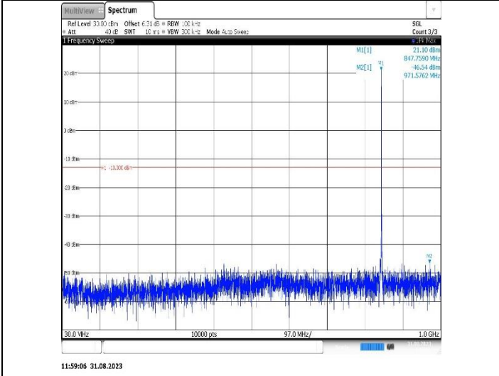
Band26(824-849)-1.4MHz-16QAM-26797-1RB#0-Range1:30~1000MHz
