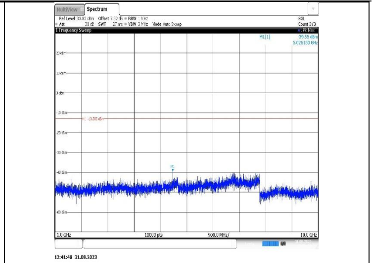
Band26(824-849)-3MHz-16QAM-26915-1RB#0-Range2:1000~10000MHz
