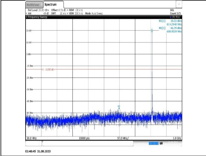
Band26(814-824)-1.4MHz-QPSK-26740-1RB#0-Range1:30~1000MHz
