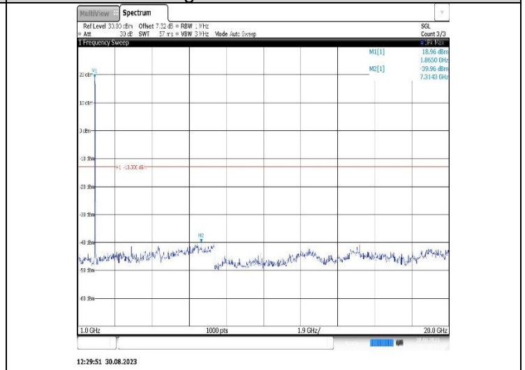
Band25-20MHz-16QAM-26590-1RB#0-Range2:1000~20000MHz
