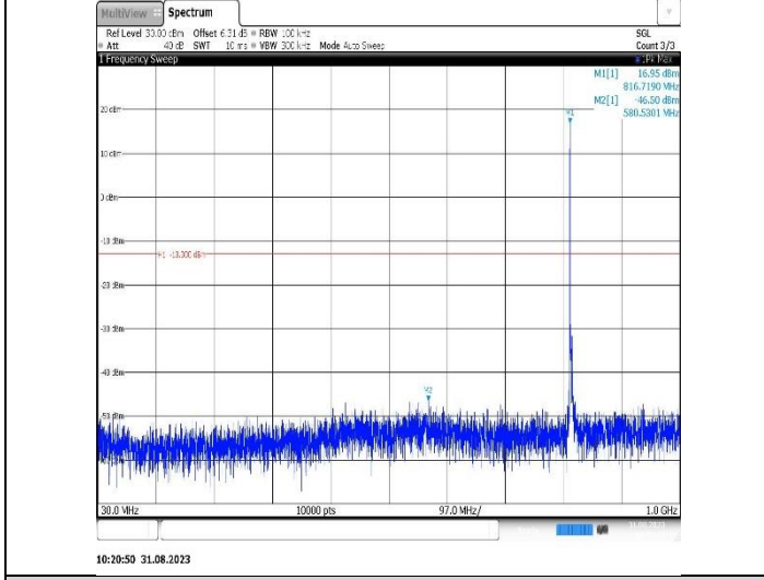
Band26(814-824)-5MHz-16QAM-26765-1RB#0-Range1:30~1000MHz
