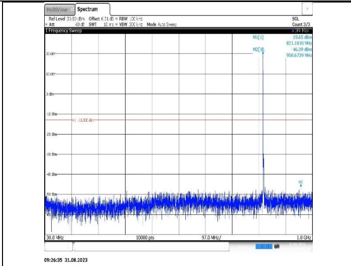
Band26(814-824)-3MHz-16QAM-26705-1RB#0-Range1:30~1000MHz
