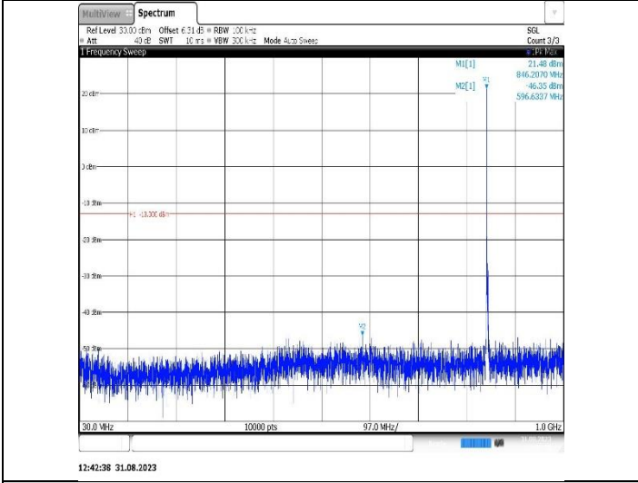
Band26(824-849)-3MHz-16QAM-26805-1RB#0-Range1:30~1000MHz
