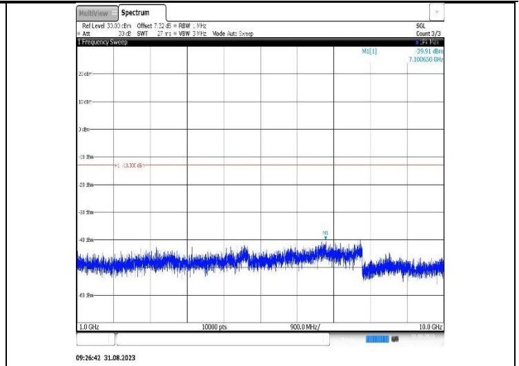
Band26(814-824)-3MHz-16QAM-26705-1RB#0-Range2:1000~10000MHz
