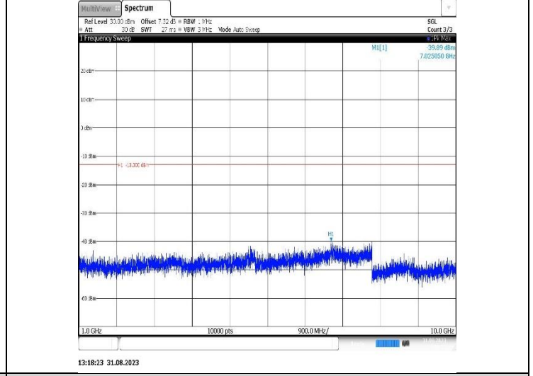
Band26(824-849)-5MHz-16QAM-26815-1RB#0-Range2:1000~10000MHz
