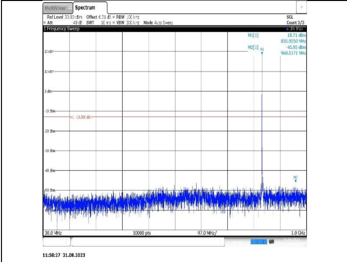
Band26(824-849)-1.4MHz-QPSK-27033-1RB#0-Range1:30~1000MHz
