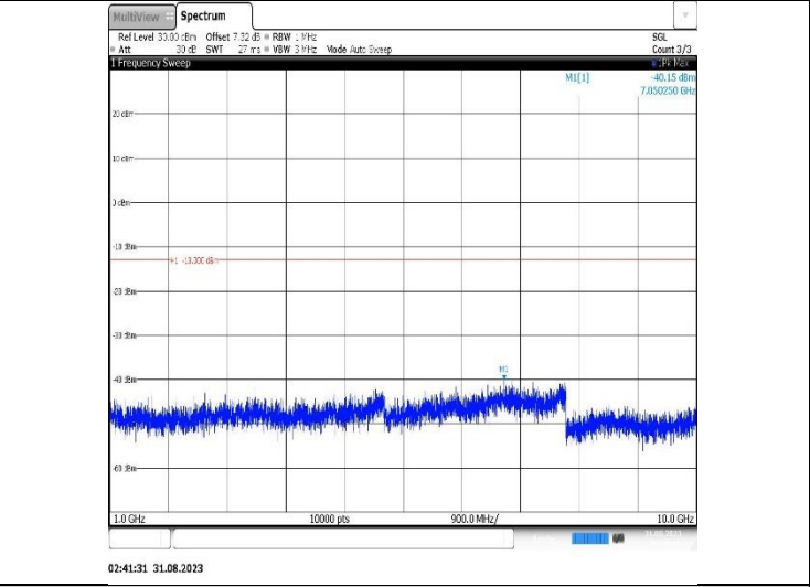
Band26(814-824)-1.4MHz-QPSK-26783-1RB#0-Range2:1000~10000MHz
