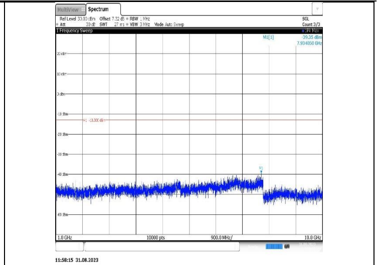
Band26(824-849)-1.4MHz-16QAM-26915-1RB#0-Range2:1000~10000MHz
