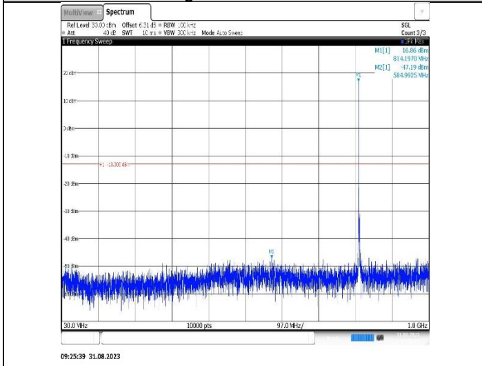
Band26(814-824)-3MHz-16QAM-26740-1RB#0-Range1:30~1000MHz
