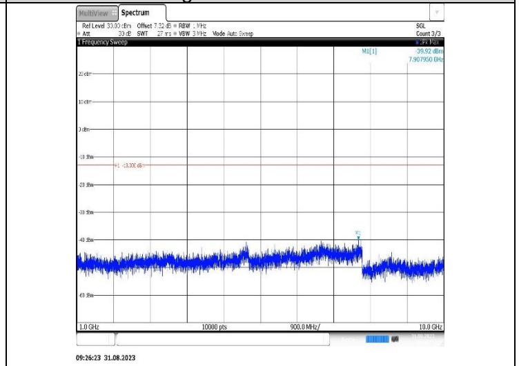
Band26(814-824)-3MHz-16QAM-26775-1RB#0-Range2:1000~10000MHz
