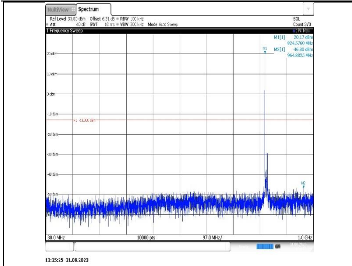
Band26(824-849)-10MHz-16QAM-26915-1RB#0-Range1:30~1000MHz
