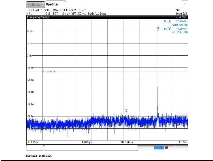
Band26(814-824)-1.4MHz-QPSK-26783-1RB#0-Range1:30~1000MHz
