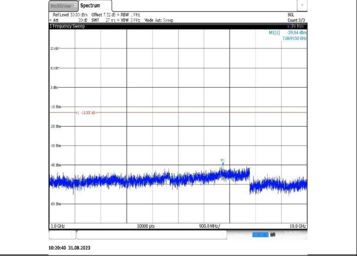
Band26(814-824)-5MHz-QPSK-26765-1RB#0-Range2:1000~10000MHz
