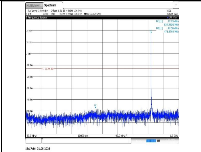
Band26(824-849)-5MHz-16QAM-26915-1RB#0-Range1:30~1000MHz
