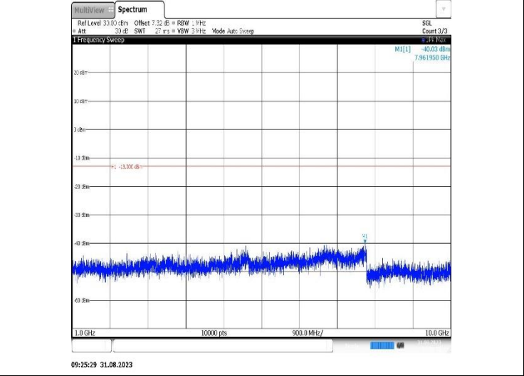
Band26(814-824)-3MHz-QPSK-26740-1RB#0-Range2:1000~10000MHz
