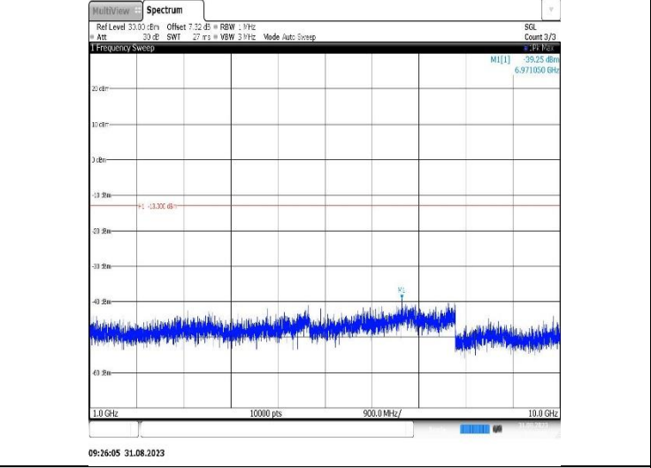
Band26(814-824)-3MHz-QPSK-26775-1RB#0-Range2:1000~10000MHz
