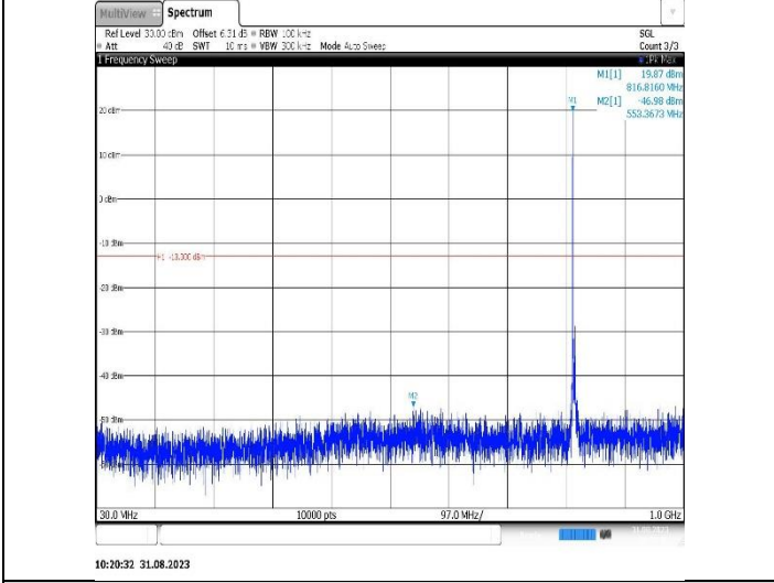
Band26(814-824)-5MHz-QPSK-26765-1RB#0-Range1:30~1000MHz
