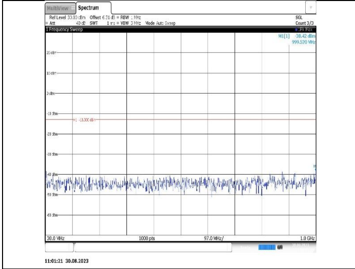
Band25-3MHz-QPSK-26365-1RB#0-Range1:30~1000MHz
