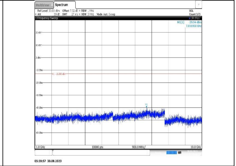
Band17-10MHz-16QAM-23790-1RB#0-Range2:1000~10000MHz
