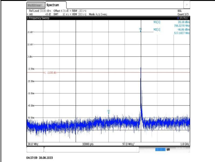
Band17-5MHz-QPSK-23755-1RB#0-Range1:30~1000MHz
