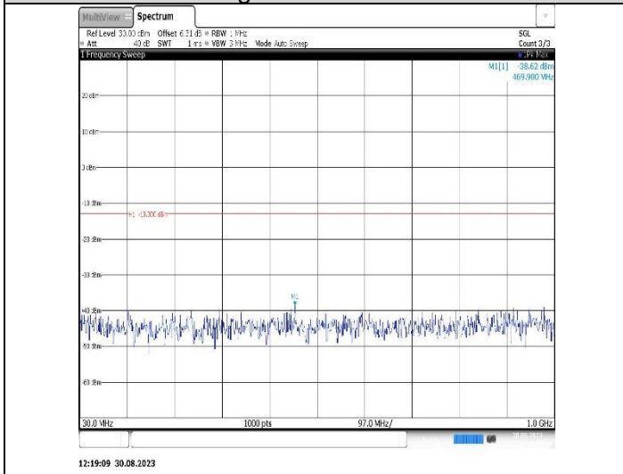
Band25-15MHz-QPSK-26615-1RB#0-Range1:30~1000MHz
