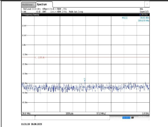
Band25-10MHz-QPSK-26090-1RB#0-Range1:30~1000MHz
