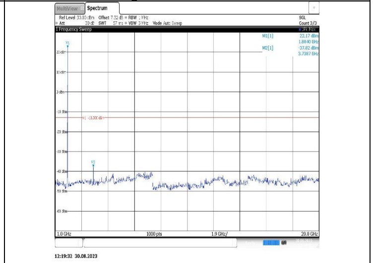
Band25-15MHz-16QAM-26615-1RB#0-Range2:1000~20000MHz
