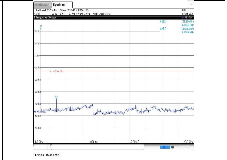
Band25-5MHz-16QAM-26365-1RB#0-Range2:1000~20000MHz
