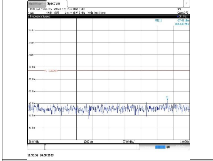
Band25-5MHz-16QAM-26665-1RB#0-Range1:30~1000MHz
