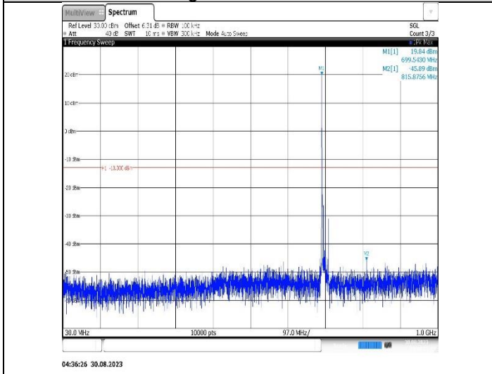
Band12-10MHz-QPSK-23095-1RB#0-Range1:30~1000MHz
