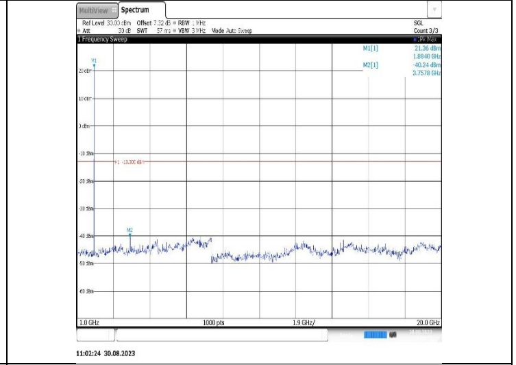
Band25-3MHz-16QAM-26675-1RB#0-Range2:1000~20000MHz
