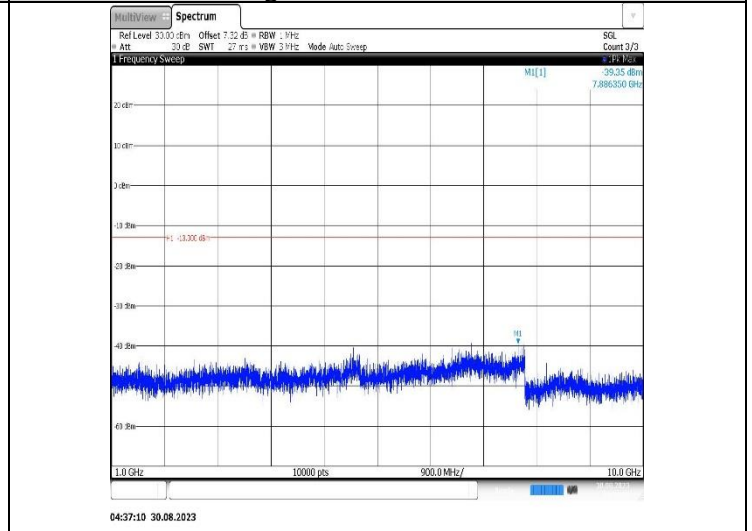
Band12-10MHz-QPSK-23130-1RB#0-Range2:1000~10000MHz
