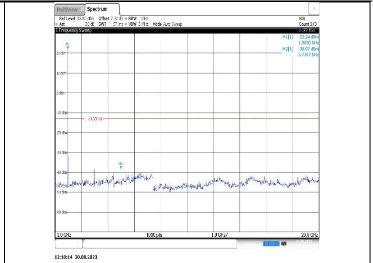
Band25-10MHz-16QAM-26090-1RB#0-Range2:1000~20000MHz
