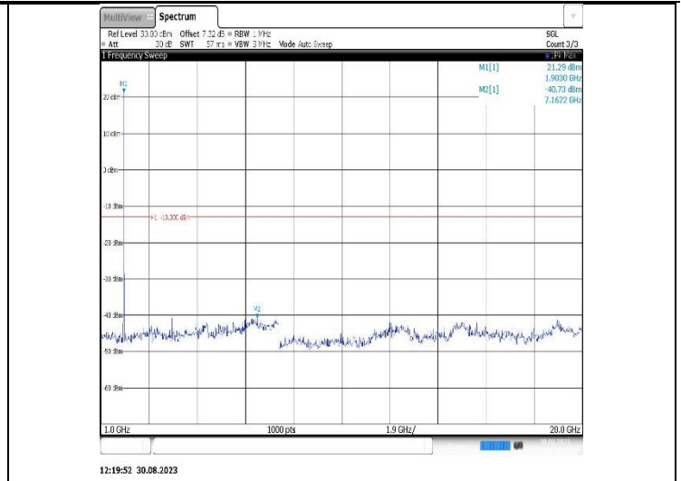
Band25-15MHz-16QAM-26115-1RB#0-Range2:1000~20000MHz
