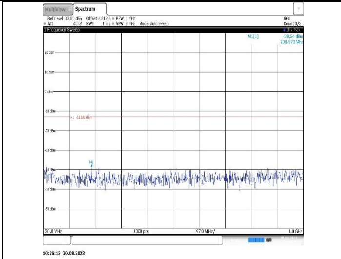
Band25-3MHz-QPSK-26055-1RB#0-Range1:30~1000MHz
