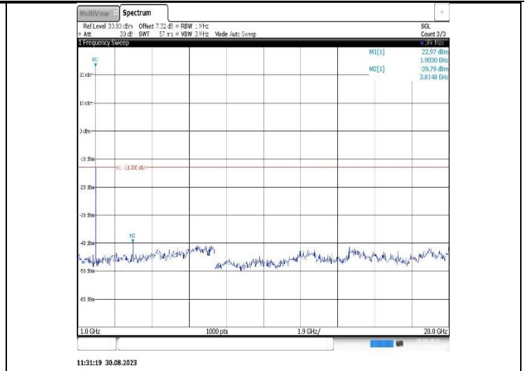
Band25-5MHz-16QAM-26065-1RB#0-Range2:1000~20000MHz
