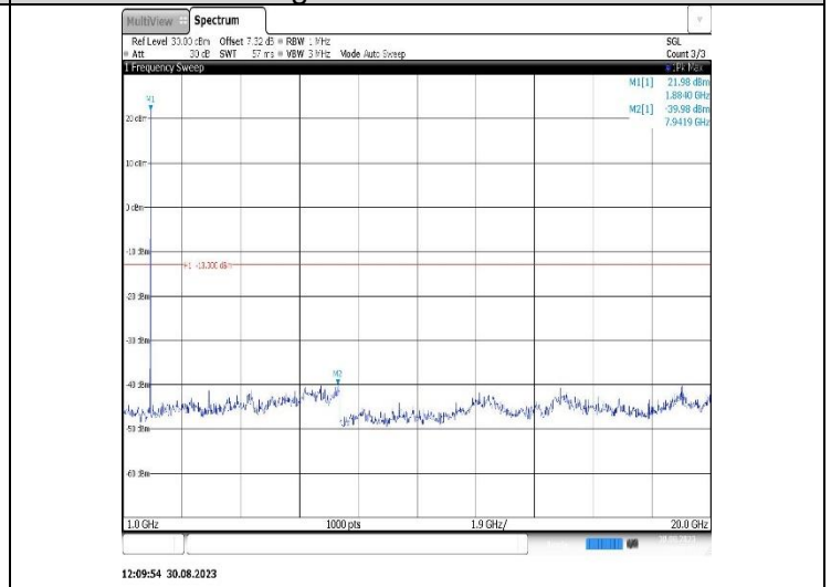
Band25-10MHz-16QAM-26640-1RB#0-Range2:1000~20000MHz
