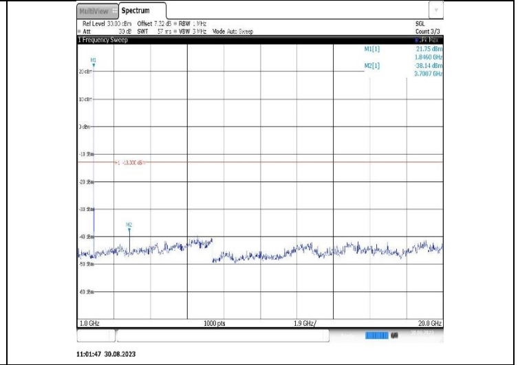
Band25-3MHz-16QAM-26365-1RB#0-Range2:1000~20000MHz
