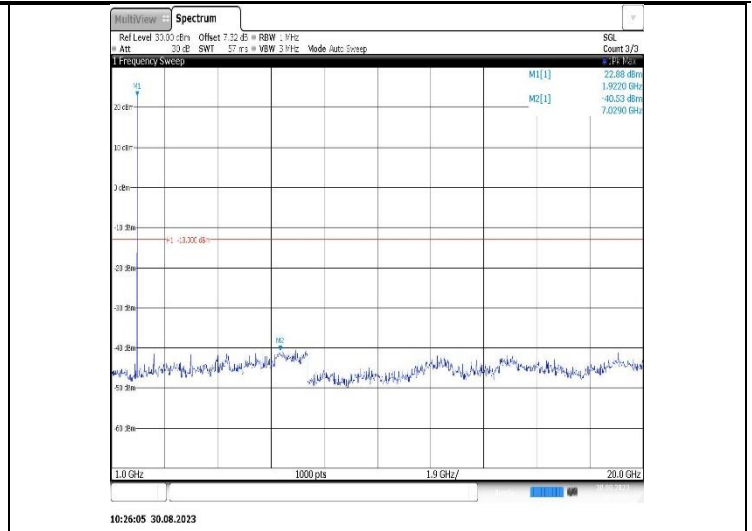
Band25-1.4MHz-16QAM-26047-1RB#0-Range2:1000~20000MHz
