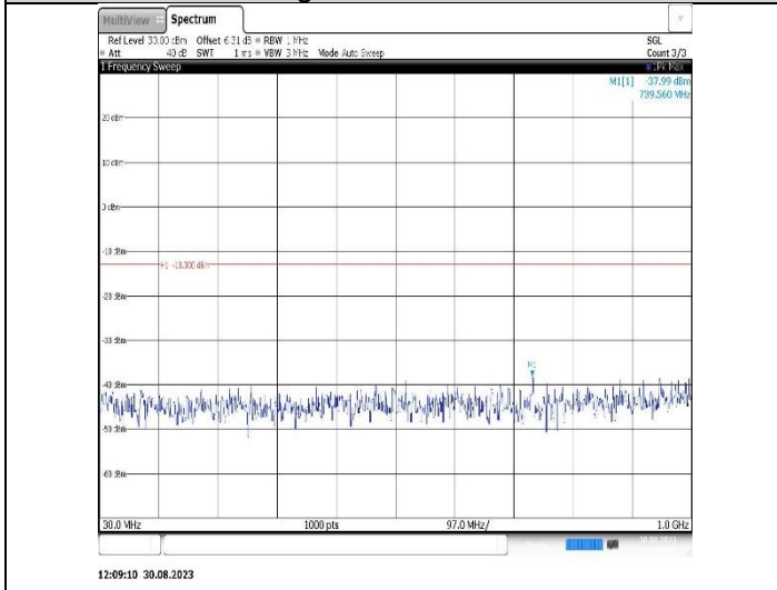
Band25-10MHz-16QAM-26365-1RB#0-Range1:30~1000MHz
