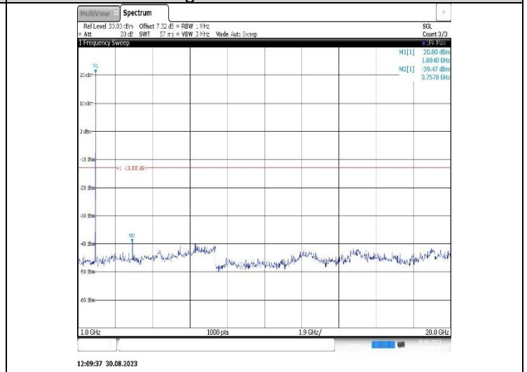
Band25-10MHz-QPSK-26640-1RB#0-Range2:1000~20000MHz
