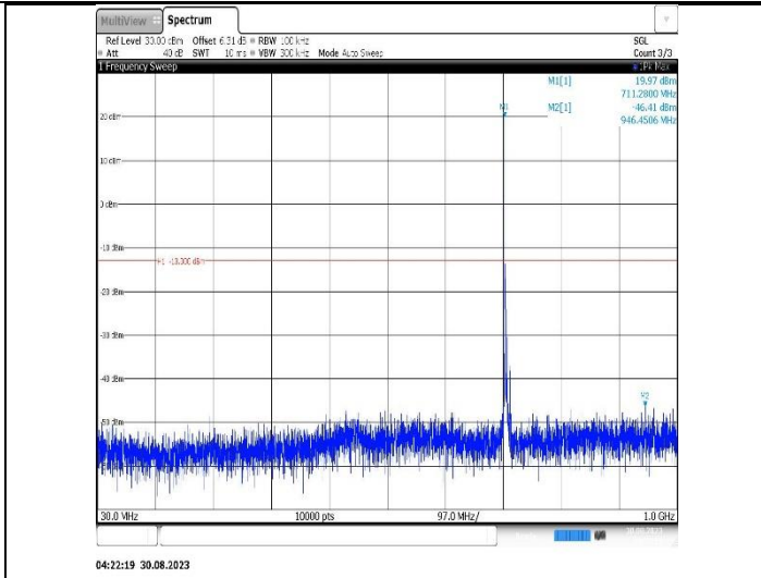
Band12-10MHz-QPSK-23060-1RB#0-Range1:30~1000MHz
