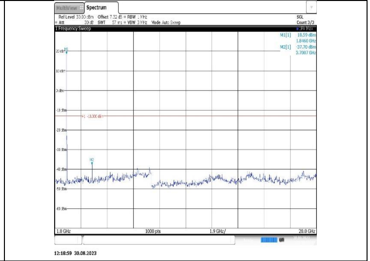
Band25-15MHz-16QAM-26365-1RB#0-Range2:1000~20000MHz
