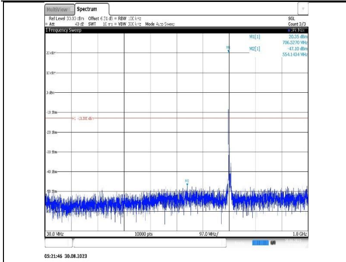
Band17-10MHz-16QAM-23780-1RB#0-Range1:30~1000MHz
