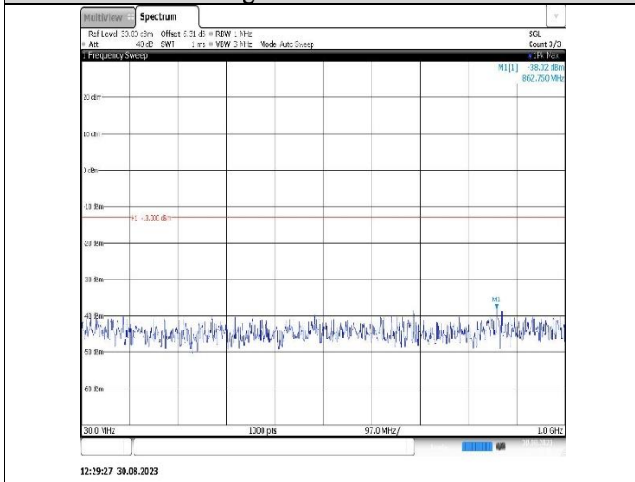
Band25-20MHz-QPSK-26590-1RB#0-Range1:30~1000MHz
