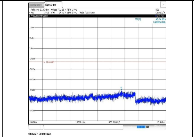
Band12-10MHz-QPSK-23060-1RB#0-Range2:1000~10000MHz
