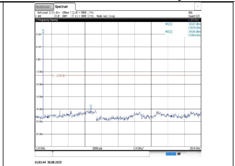
Band25-3MHz-16QAM-26055-1RB#0-Range2:1000~20000MHz
