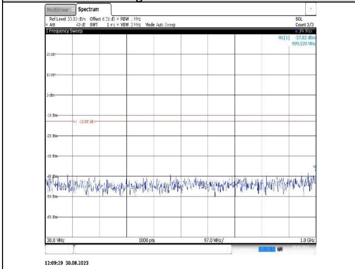
Band25-10MHz-QPSK-26640-1RB#0-Range1:30~1000MHz
