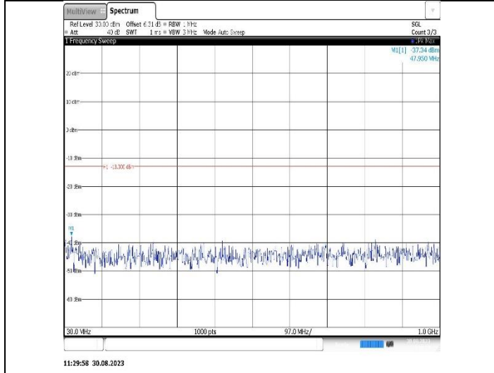
Band25-5MHz-QPSK-26365-1RB#0-Range1:30~1000MHz
