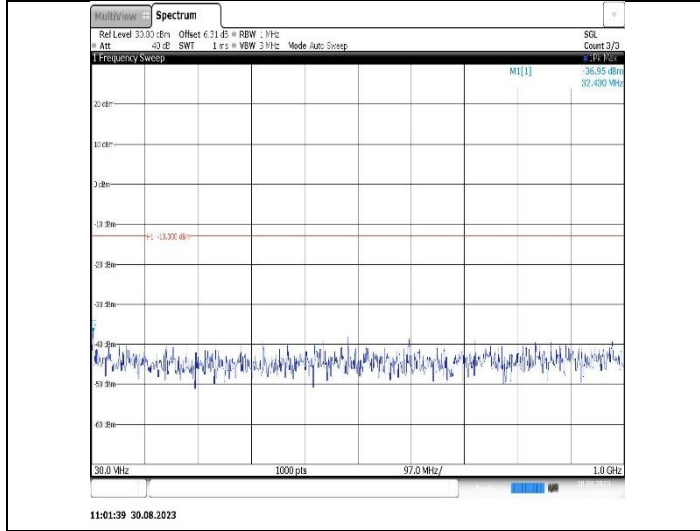
Band25-3MHz-16QAM-26365-1RB#0-Range1:30~1000MHz
