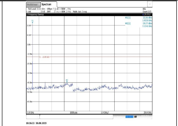
Band25-3MHz-QPSK-26055-1RB#0-Range2:1000~20000MHz
