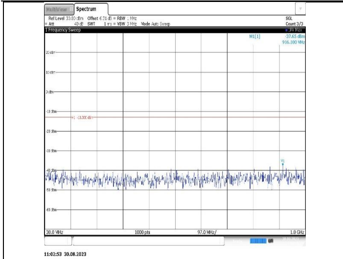
Band25-5MHz-QPSK-26065-1RB#0-Range1:30~1000MHz
