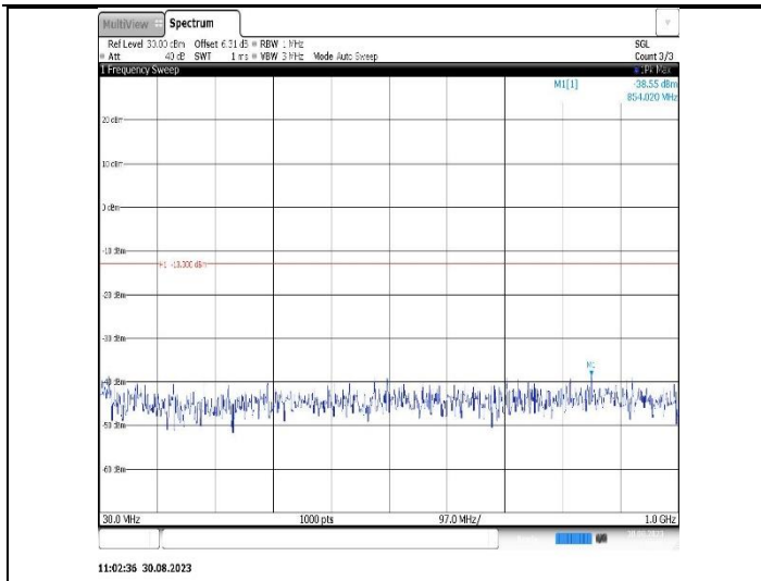
Band25-3MHz-16QAM-26055-1RB#0-Range1:30~1000MHz
