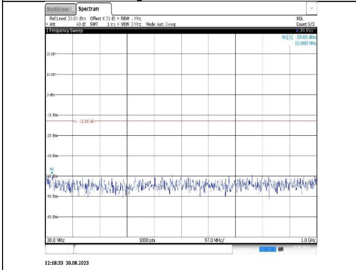
Band25-15MHz-QPSK-26365-1RB#0-Range1:30~1000MHz
