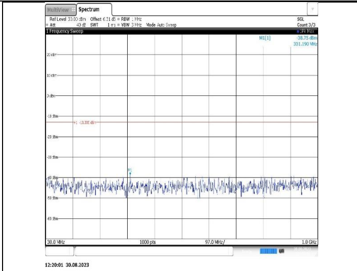
Band25-20MHz-QPSK-26140-1RB#0-Range1:30~1000MHz
