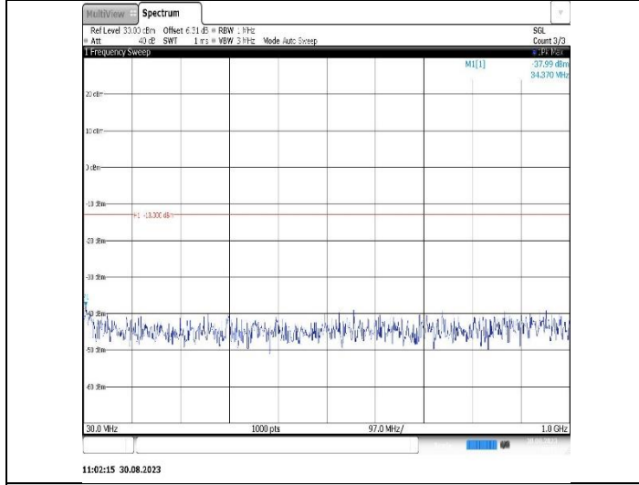
Band25-3MHz-16QAM-26675-1RB#0-Range1:30~1000MHz
