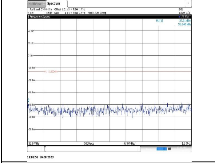
Band25-3MHz-QPSK-26675-1RB#0-Range1:30~1000MHz
