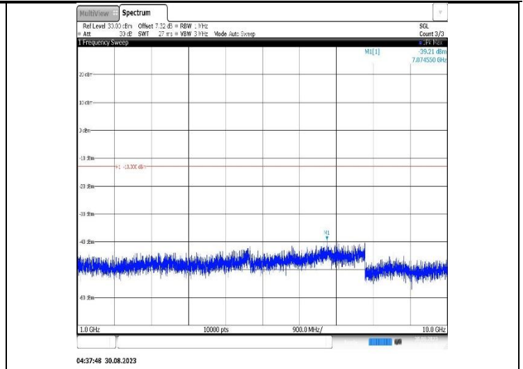
Band12-10MHz-16QAM-23060-1RB#0-Range2:1000~10000MHz
