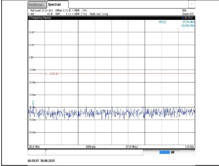
Band25-1.4MHz-16QAM-26683-1RB#0-Range1:30~1000MHz
