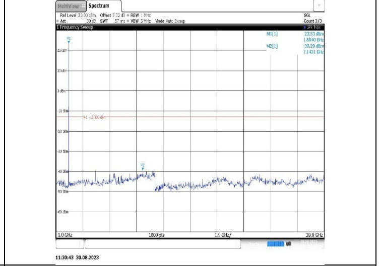
Band25-5MHz-QPSK-26665-1RB#0-Range2:1000~20000MHz
