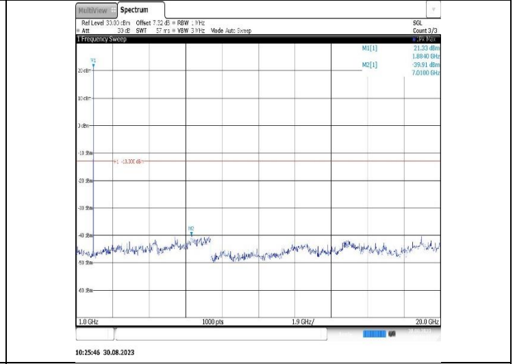
Band25-1.4MHz-16QAM-26683-1RB#0-Range2:1000~20000MHz
