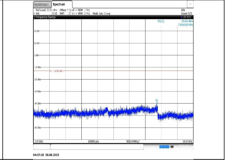
Band12-10MHz-16QAM-23130-1RB#0-Range2:1000~10000MHz
