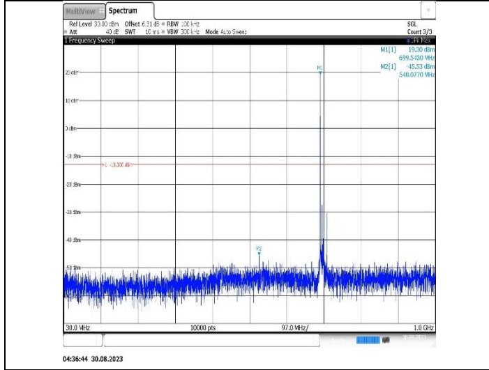
Band12-10MHz-16QAM-23095-1RB#0-Range1:30~1000MHz
