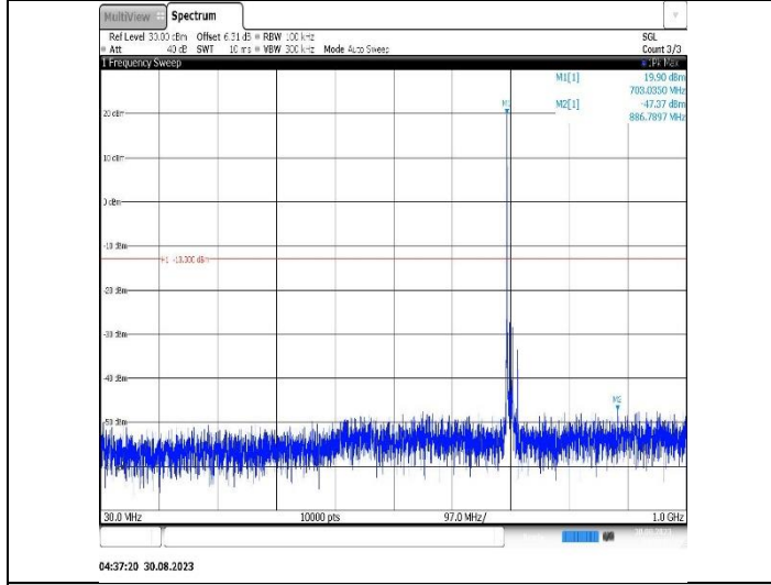
Band12-10MHz-16QAM-23130-1RB#0-Range1:30~1000MHz
