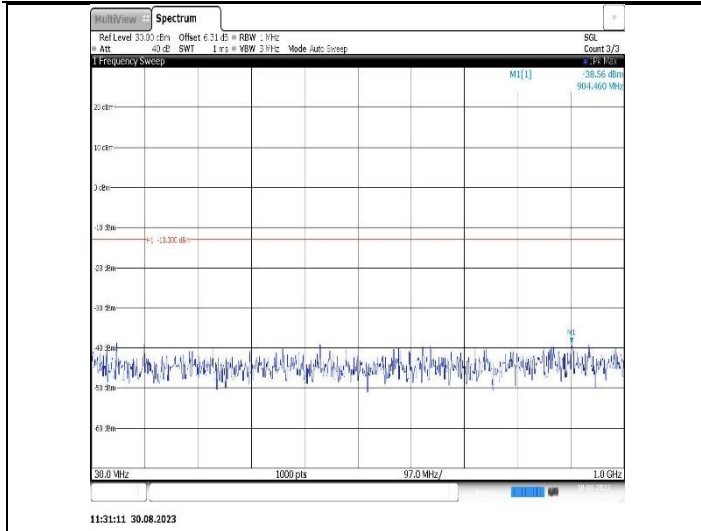
Band25-5MHz-16QAM-26065-1RB#0-Range1:30~1000MHz
