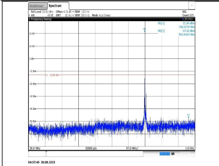
Band12-10MHz-16QAM-23060-1RB#0-Range1:30~1000MHz
