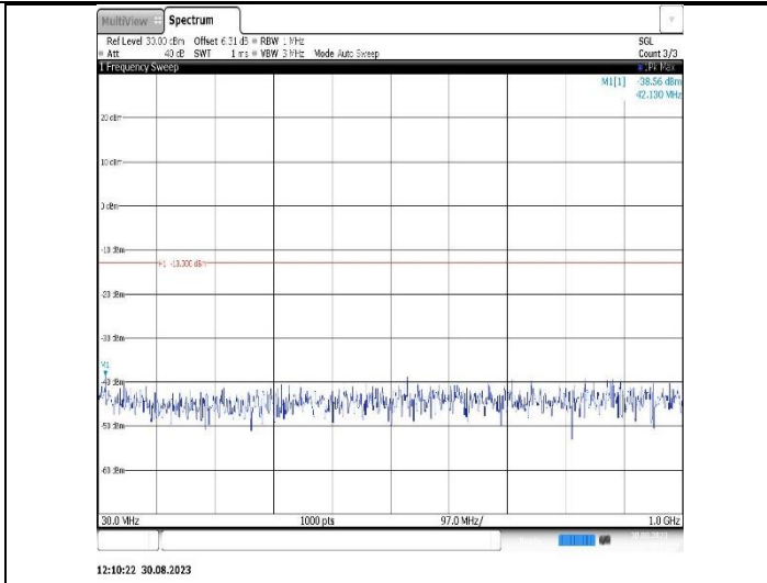
Band25-15MHz-QPSK-26115-1RB#0-Range1:30~1000MHz
