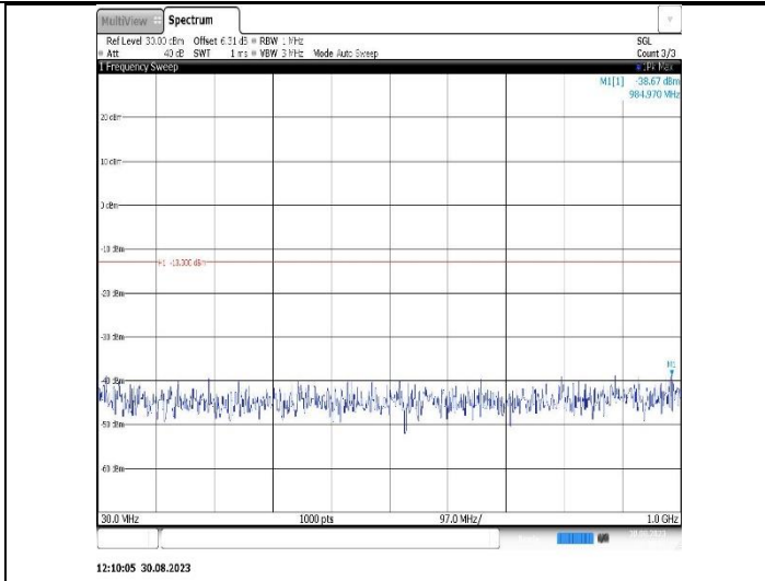
Band25-10MHz-16QAM-26090-1RB#0-Range1:30~1000MHz
