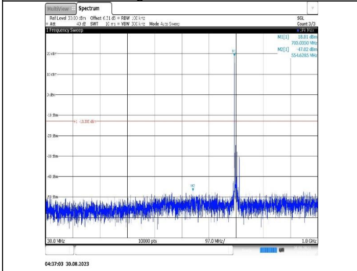
Band12-10MHz-QPSK-23130-1RB#0-Range1:30~1000MHz
