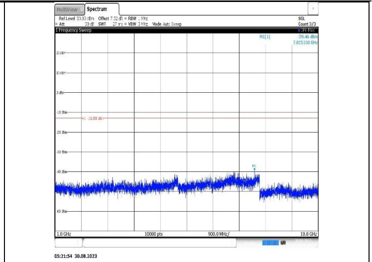
Band17-10MHz-16QAM-23780-1RB#0-Range2:1000~10000MHz
