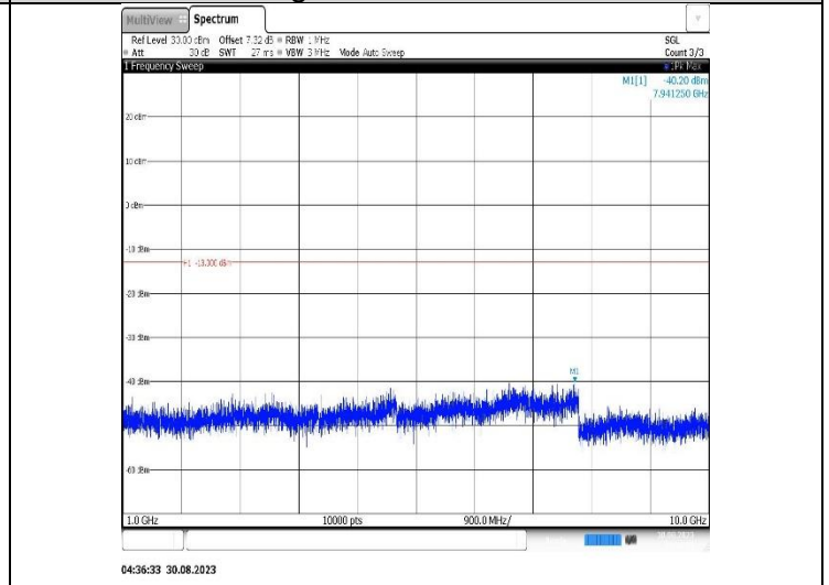
Band12-10MHz-QPSK-23095-1RB#0-Range2:1000~10000MHz
