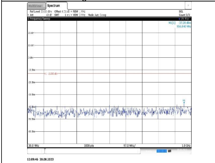
Band25-10MHz-16QAM-26640-1RB#0-Range1:30~1000MHz
