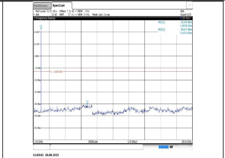
Band25-5MHz-QPSK-26065-1RB#0-Range2:1000~20000MHz
