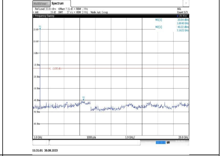
Band25-5MHz-16QAM-26665-1RB#0-Range2:1000~20000MHz
