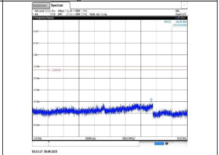
Band17-10MHz-QPSK-23800-1RB#0-Range2:1000~10000MHz
