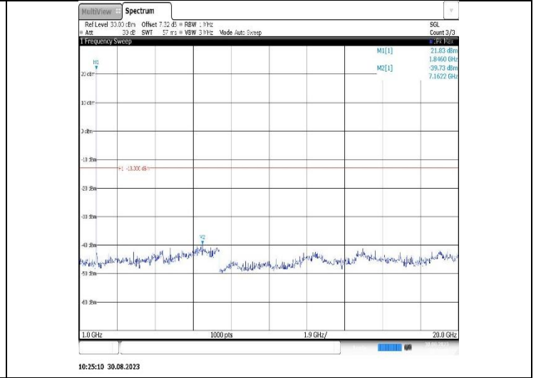
Band25-1.4MHz-16QAM-26365-1RB#0-Range2:1000~20000MHz
