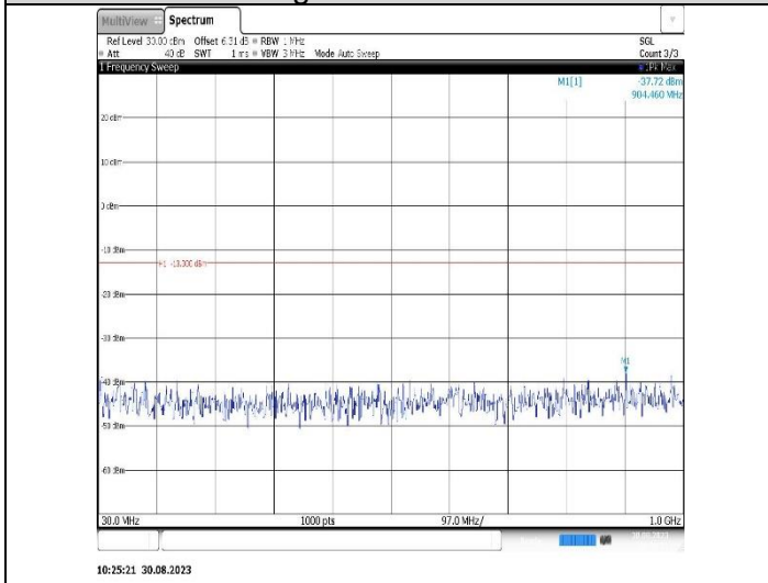
Band25-1.4MHz-QPSK-26683-1RB#0-Range1:30~1000MHz
