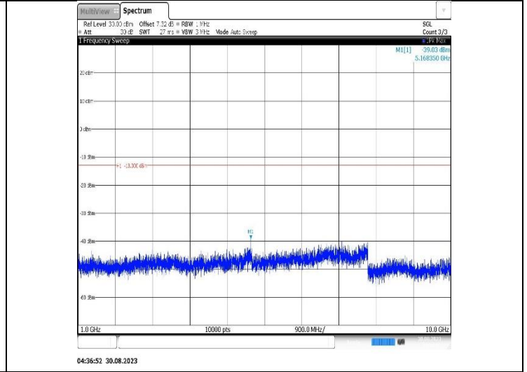
Band12-10MHz-16QAM-23095-1RB#0-Range2:1000~10000MHz
