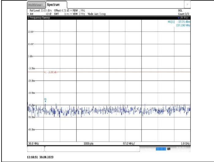
Band25-15MHz-16QAM-26365-1RB#0-Range1:30~1000MHz
