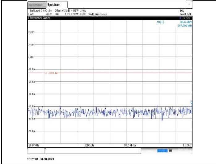
Band25-1.4MHz-16QAM-26365-1RB#0-Range1:30~1000MHz
