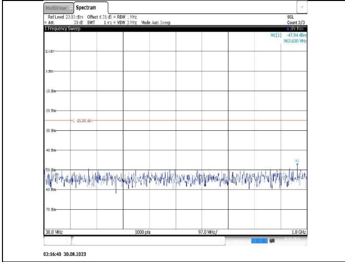
Band7-5MHz-QPSK-21100-1RB#0-Range1:30~1000MHz
