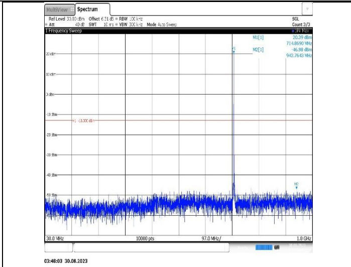
Band12-3MHz-QPSK-23025-1RB#0- Range1:30~1000MHz
