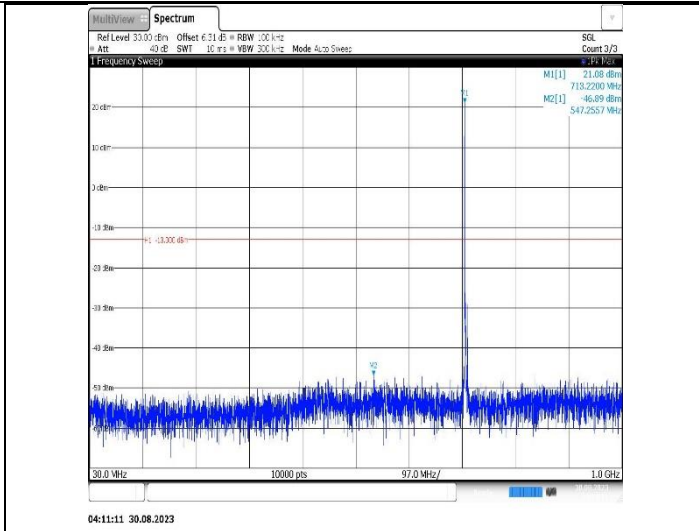
Band12-3MHz-16QAM-23025-1RB#0-Range1:30~1000MHz
