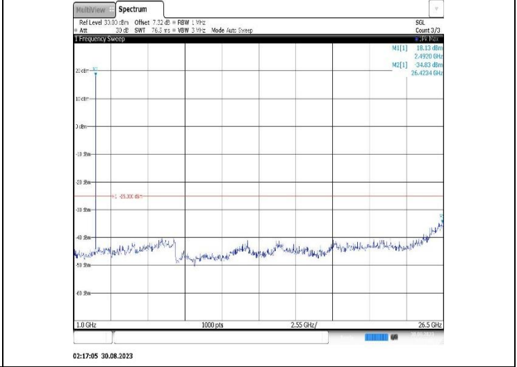
Band7-5MHz-16QAM-21100-1RB#0- Range2:1000~26500MHz
