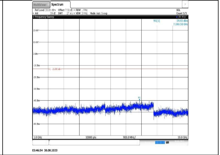
Band12-1.4MHz-16QAM-23095-1RB#0-Range2:1000~10000MHz
