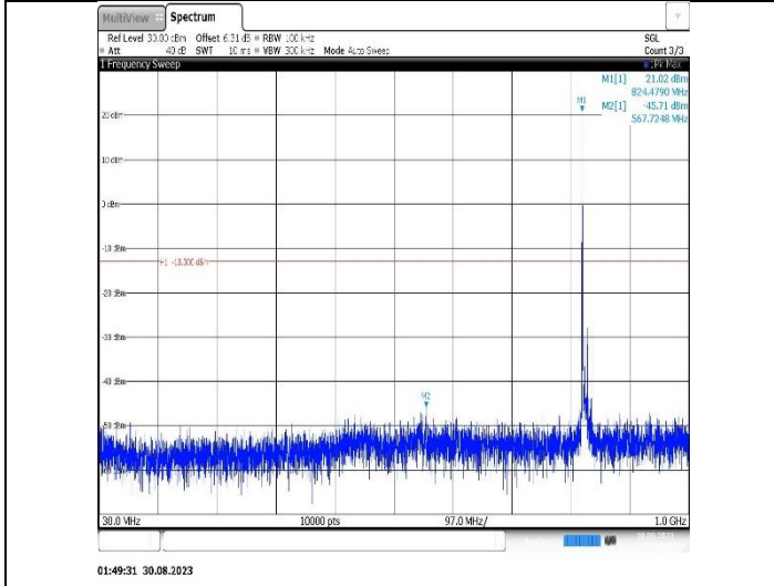
Band5-10MHz-QPSK-20525-1RB#0- Range1:30~1000MHz
