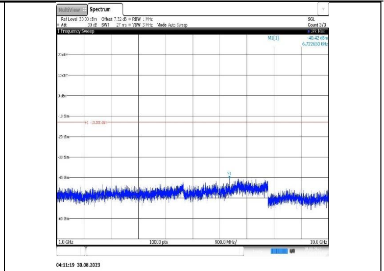
Band12-3MHz-16QAM-23025-1RB#0-Range2:1000~10000MHz
