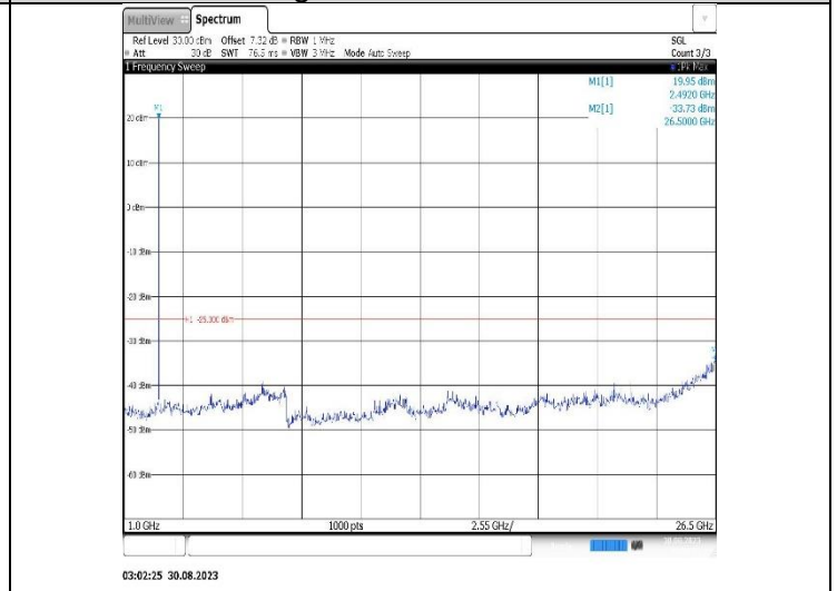
Band7-15MHz-16QAM-21100-1RB#0-Range2:1000~26500MHz
