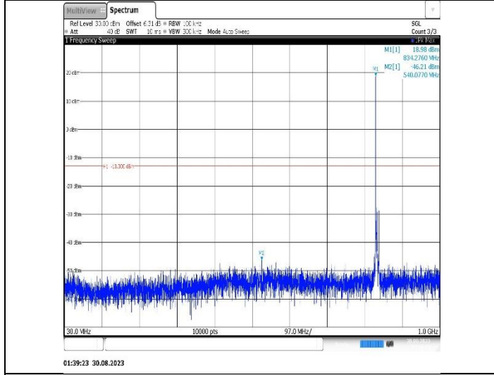
Band5-5MHz-16QAM-20625-1RB#0-Range1:30~1000MHz
