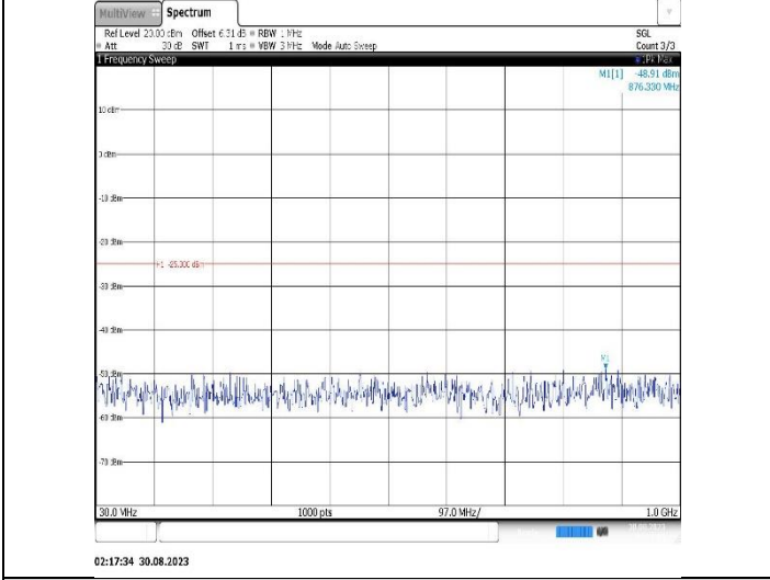
Band7-5MHz-16QAM-21425-1RB#0- Range1:30~1000MHz
