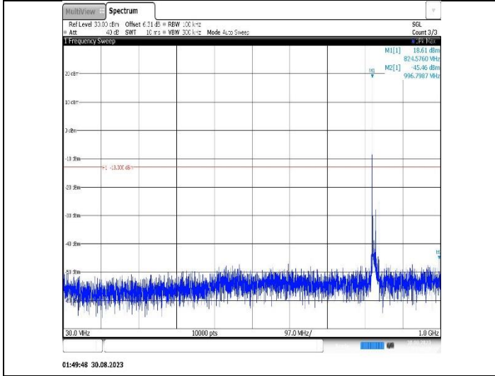
Band5-10MHz-16QAM-20525-1RB#0-Range1:30~1000MHz
