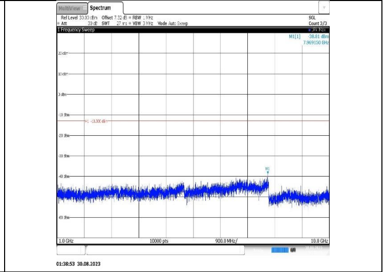
Band5-5MHz-16QAM-20525-1RB#0-Range2:1000~10000MHz
