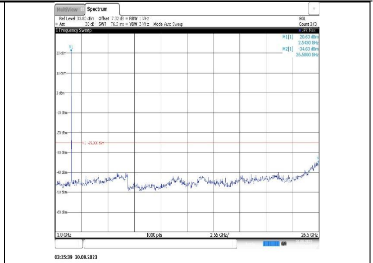
Band7-20MHz-16QAM-20850-1RB#0-Range2:1000~26500MHz
