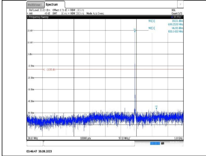
Band12-1.4MHz-16QAM-23095-1RB#0-Range1:30~1000MHz
