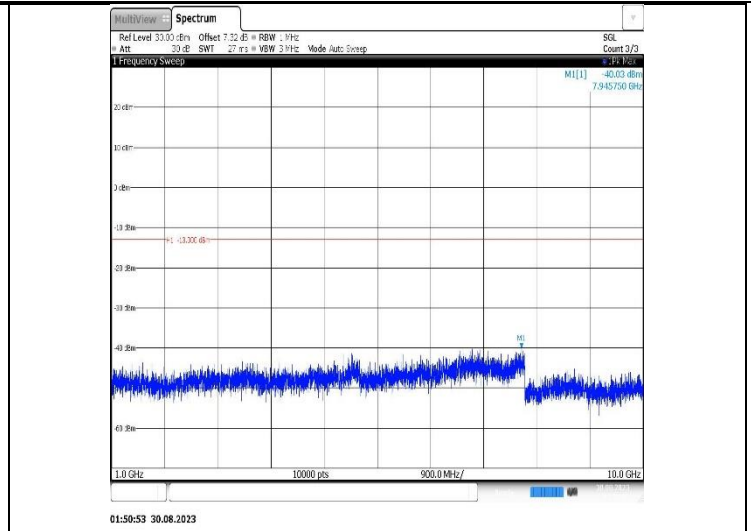
Band5-10MHz-16QAM-20450-1RB#0-Range2:1000~10000MHz
