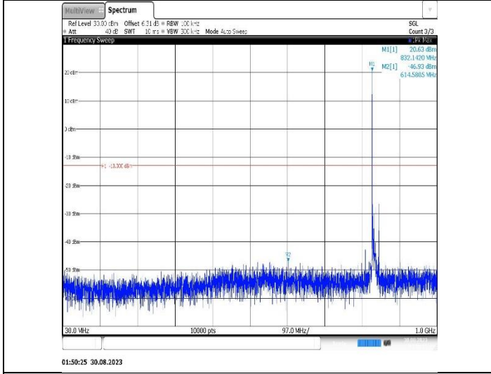
Band5-10MHz-16QAM-20600-1RB#0-Range1:30~1000MHz
