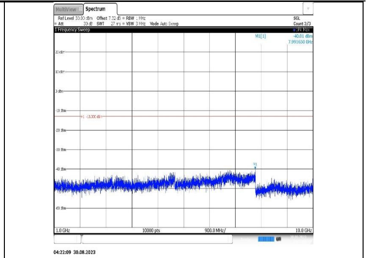
Band12-5MHz-16QAM-23035-1RB#0-Range2:1000~10000MHz
