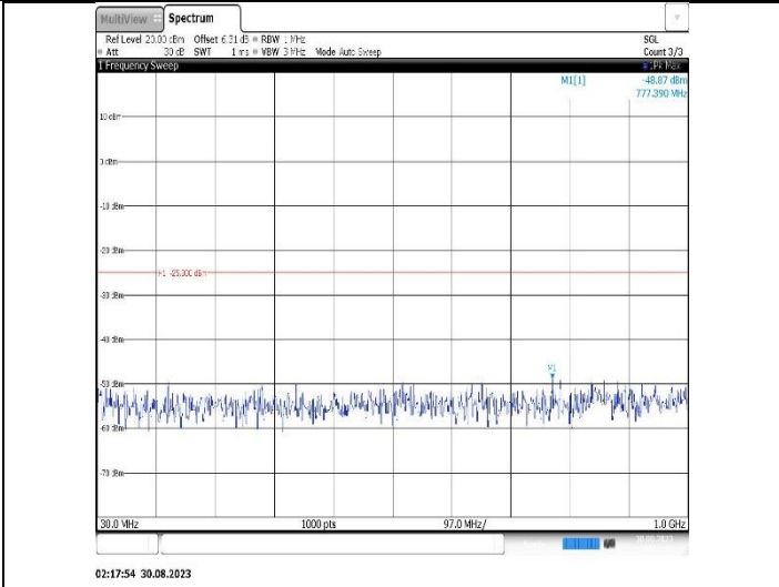
Band7-5MHz-16QAM-20775-1RB#0- Range1:30~1000MHz
