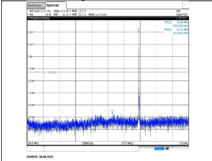
Band12-3MHz-QPSK-23095-1RB#0- Range1:30~1000MHz
