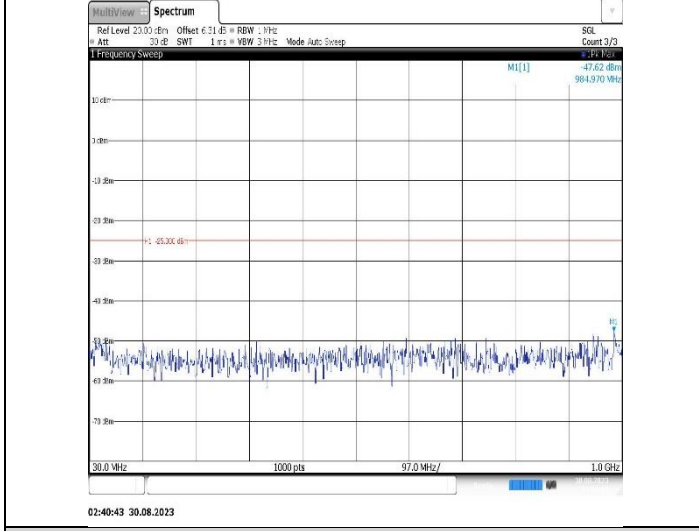
Band7-10MHz-QPSK-21400-1RB#0-Range1:30~1000MHz
