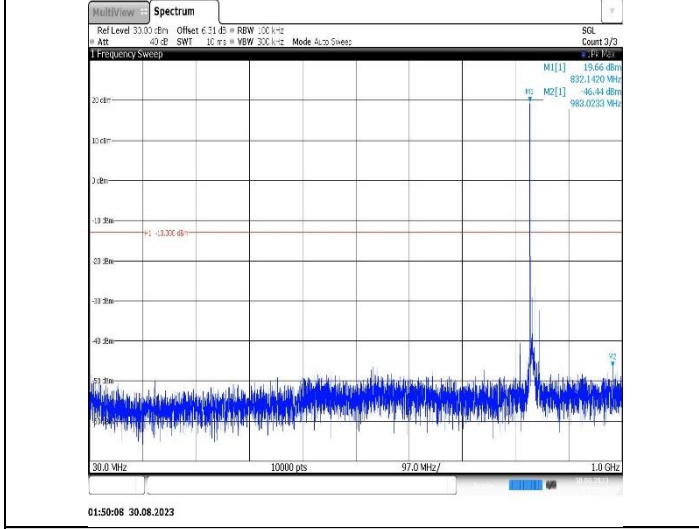
Band5-10MHz-QPSK-20600-1RB#0- Range1:30~1000MHz
