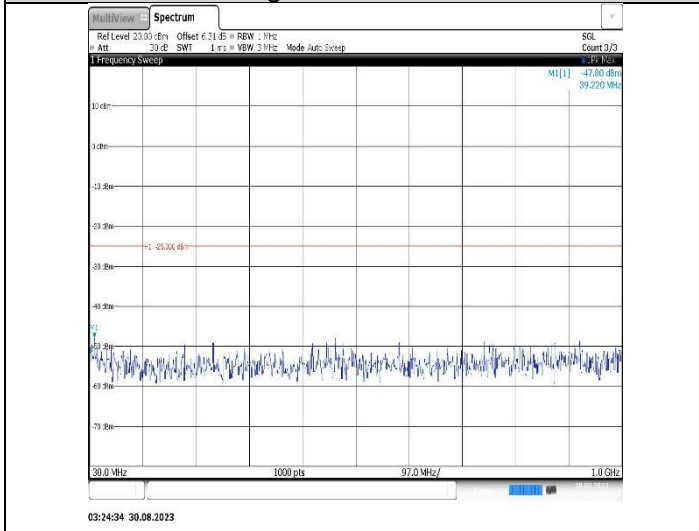
Band7-20MHz-16QAM-21100-1RB#0-Range1:30~1000MHz
