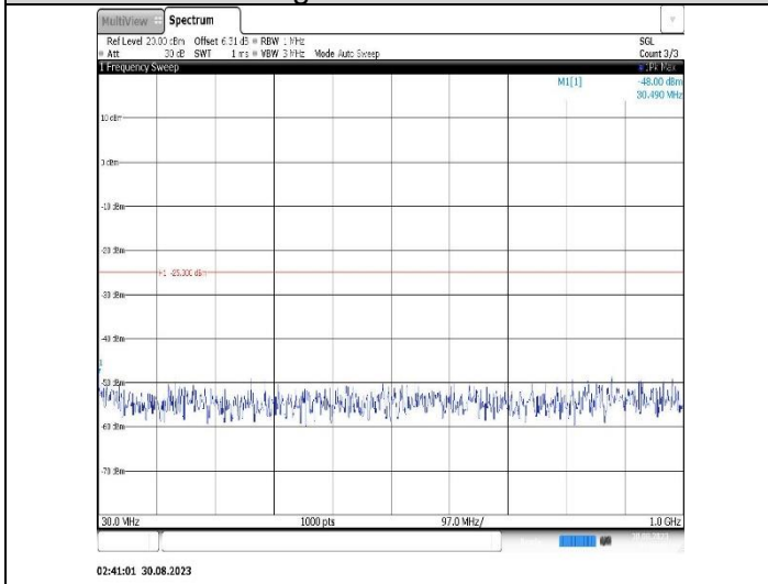
Band7-10MHz-16QAM-21400-1RB#0-Range1:30~1000MHz
