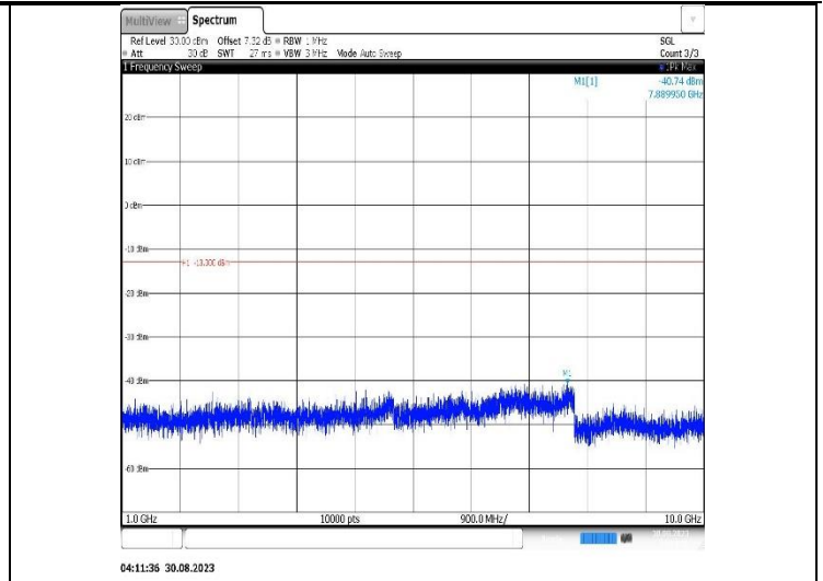
Band12-5MHz-QPSK-23035-1RB#0- Range2:1000~10000MHz
