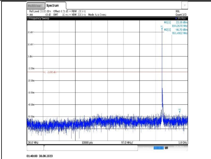
Band5-10MHz-QPSK-20450-1RB#0- Range1:30~1000MHz
