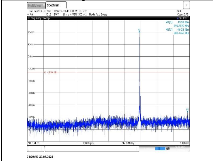
Band12-5MHz-QPSK-23095-1RB#0- Range1:30~1000MHz
