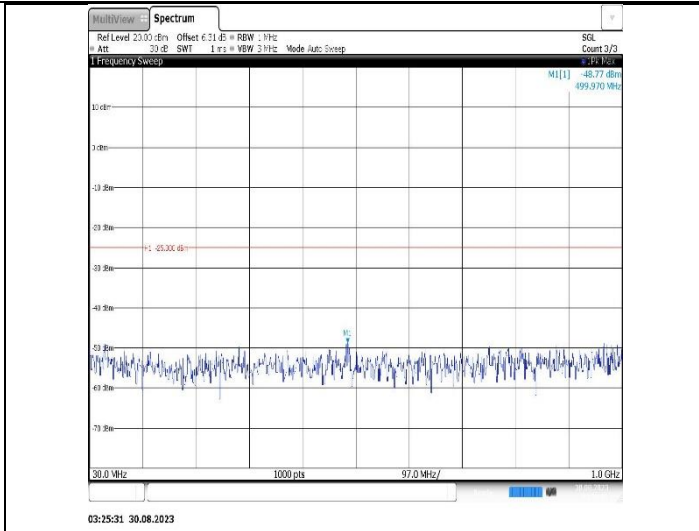
Band7-20MHz-16QAM-20850-1RB#0-Range1:30~1000MHz
