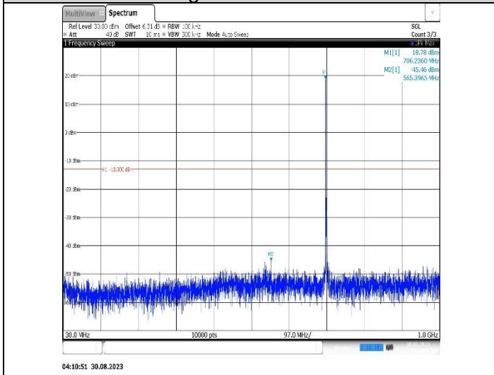
Band12-3MHz-16QAM-23165-1RB#0-Range1:30~1000MHz
