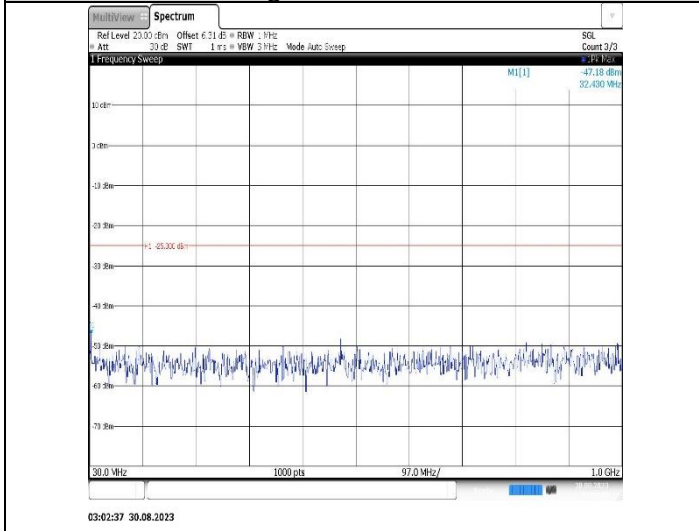
Band7-15MHz-QPSK-21375-1RB#0- Range1:30~1000MHz
