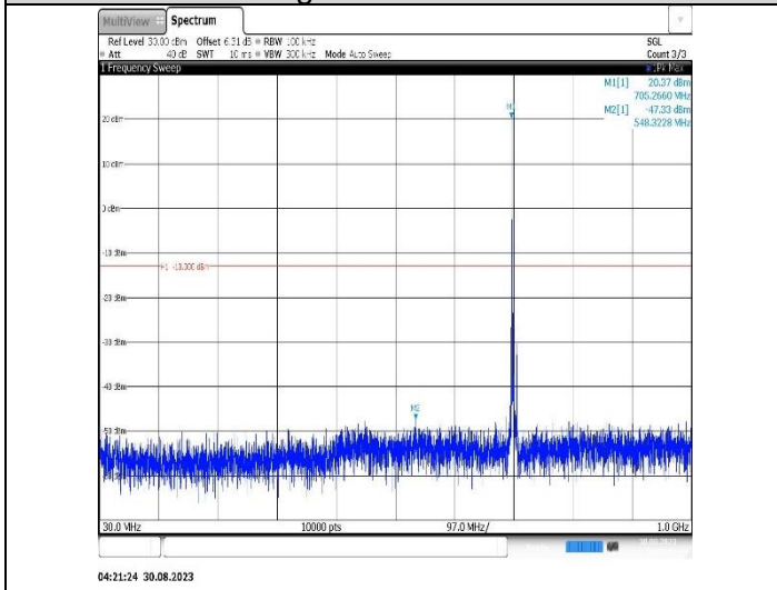
Band12-5MHz-QPSK-23155-1RB#0- Range1:30~1000MHz
