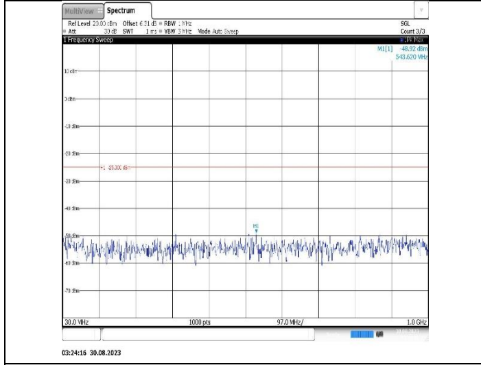
Band7-20MHz-QPSK-21100-1RB#0-Range1:30~1000MHz
