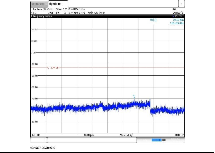
Band12-1.4MHz-QPSK-23095-1RB#0-Range2:1000~10000MHz
