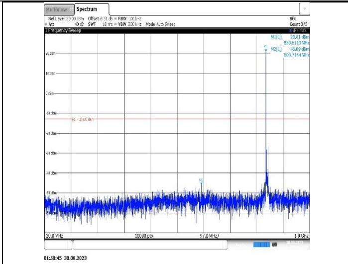
Band5-10MHz-16QAM-20450-1RB#0-Range1:30~1000MHz
