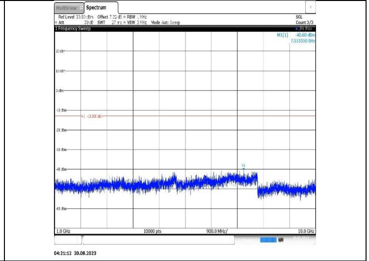
Band12-5MHz-16QAM-23095-1RB#0-Range2:1000~10000MHz
