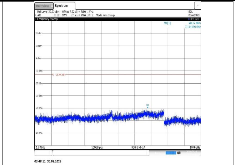
Band12-3MHz-QPSK-23025-1RB#0- Range2:1000~10000MHz
