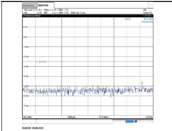
Band7-20MHz-QPSK-20850-1RB#0-Range1:30~1000MHz
