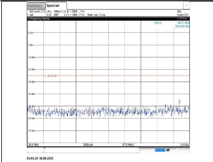
Band7-10MHz-16QAM-20800-1RB#0-Range1:30~1000MHz
