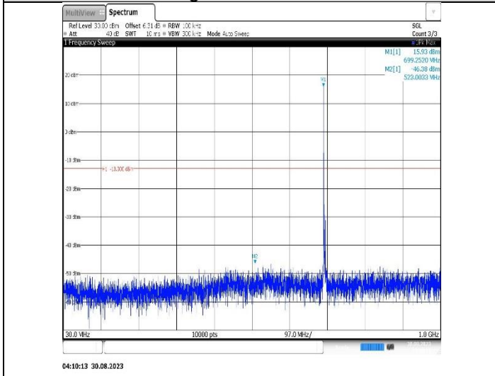
Band12-3MHz-16QAM-23095-1RB#0-Range1:30~1000MHz
