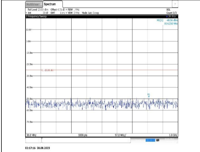
Band7-5MHz-QPSK-21425-1RB#0-Range1:30~1000MHz
