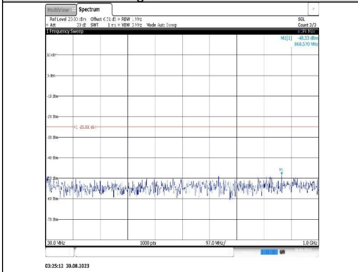
Band7-20MHz-16QAM-21350-1RB#0-Range1:30~1000MHz
