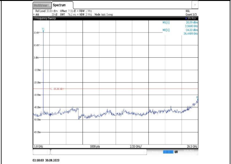
Band7-5MHz-16QAM-20775-1RB#0- Range2:1000~26500MHz
