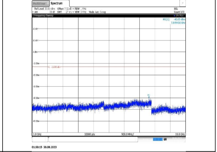
Band5-10MHz-QPSK-20600-1RB#0- Range2:1000~10000MHz
