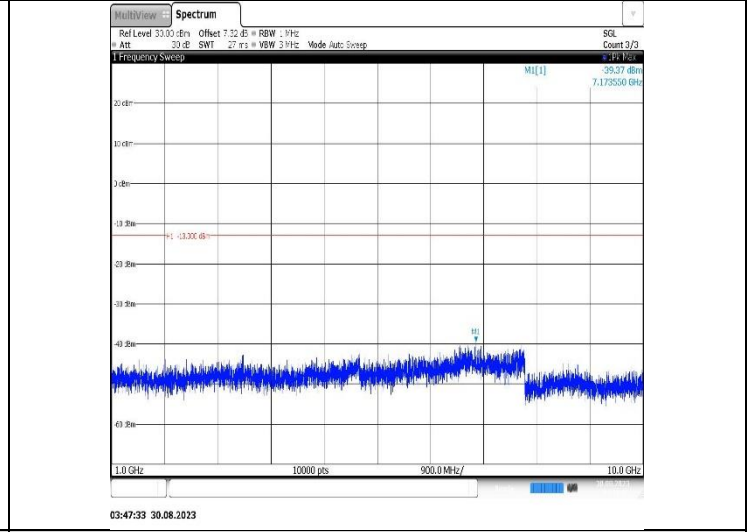
Band12-1.4MHz-16QAM-23173-1RB#0-Range2:1000~10000MHz
