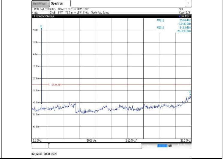
Band7-5MHz-16QAM-21425-1RB#0- Range2:1000~26500MHz
