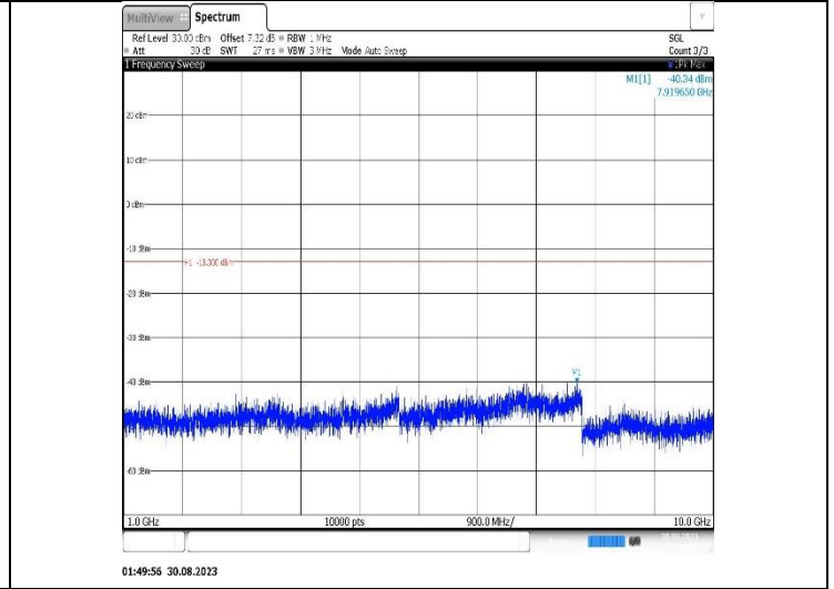
Band5-10MHz-16QAM-20525-1RB#0-Range2:1000~10000MHz
