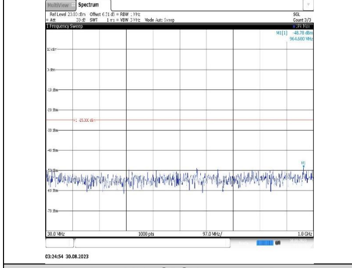
Band7-20MHz-QPSK-21350-1RB#0-Range1:30~1000MHz
