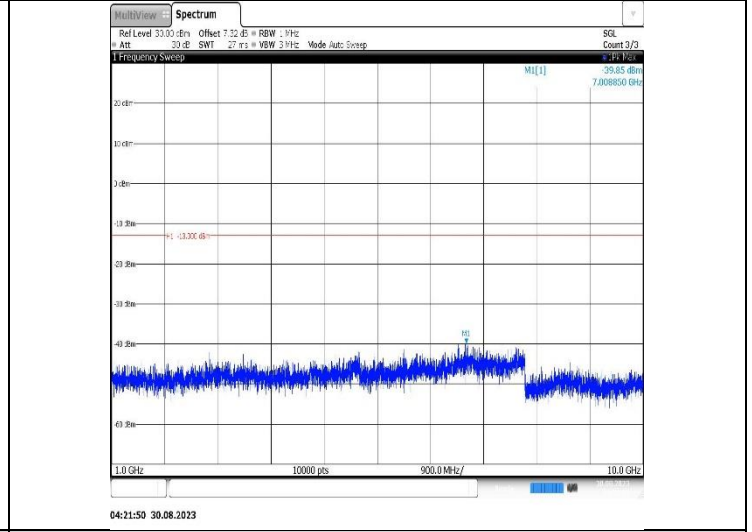
Band12-5MHz-16QAM-23155-1RB#0-Range2:1000~10000MHz
