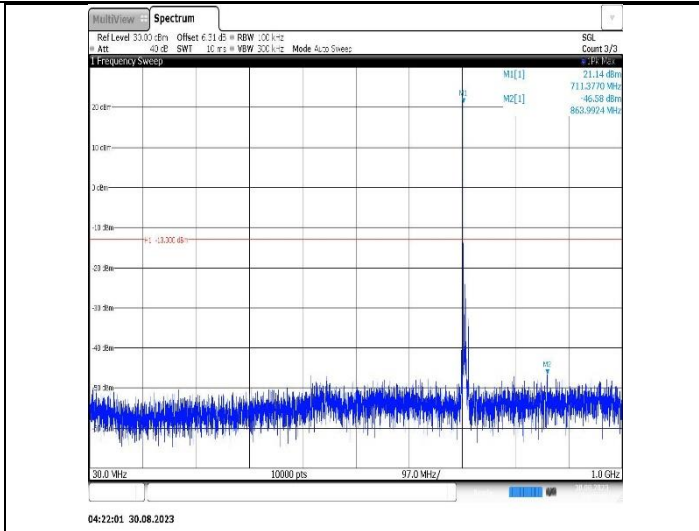
Band12-5MHz-16QAM-23035-1RB#0-Range1:30~1000MHz
