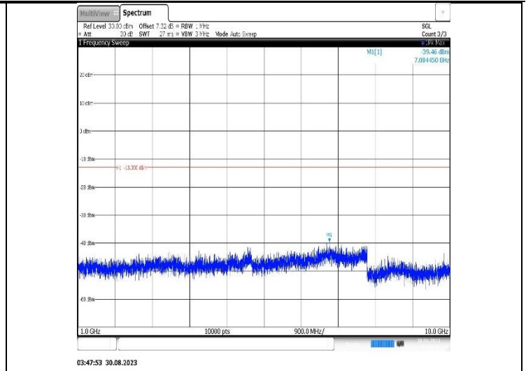
Band12-1.4MHz-16QAM-23017-1RB#0-Range2:1000~10000MHz
