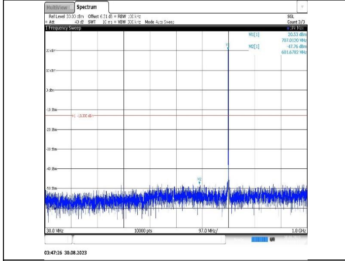
Band12-1.4MHz-16QAM-23173-1RB#0-Range1:30~1000MHz
