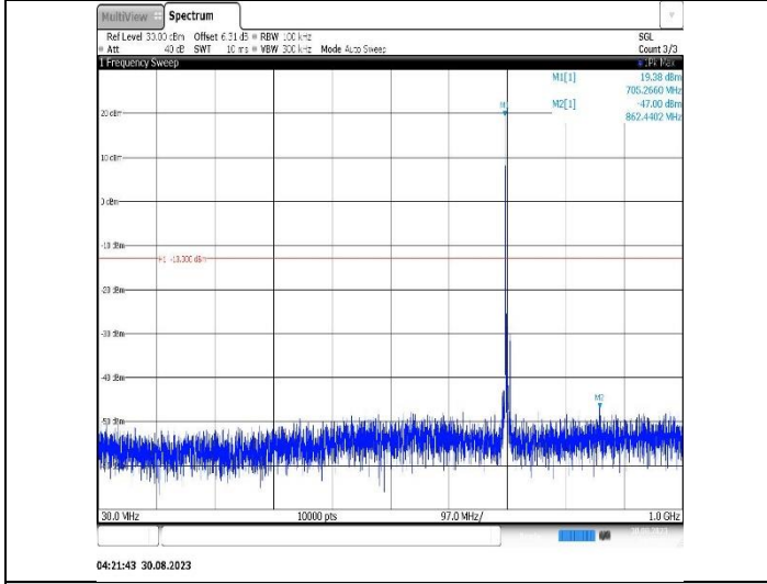
Band12-5MHz-16QAM-23155-1RB#0-Range1:30~1000MHz
