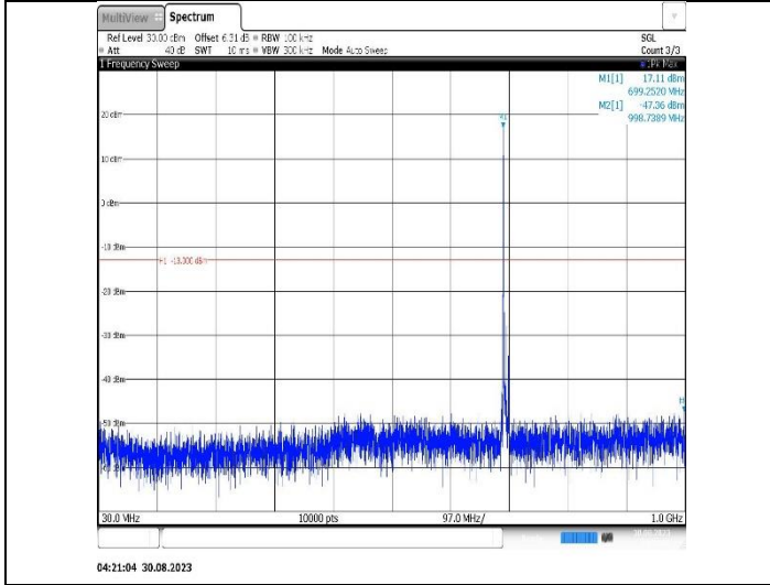
Band12-5MHz-16QAM-23095-1RB#0-Range1:30~1000MHz
