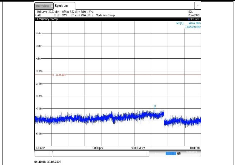
Band5-10MHz-QPSK-20450-1RB#0- Range2:1000~10000MHz
