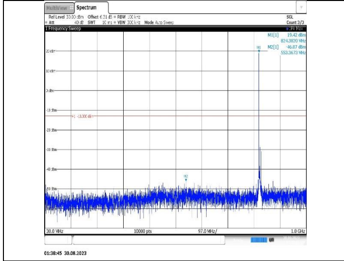
Band5-5MHz-16QAM-20525-1RB#0-Range1:30~1000MHz
