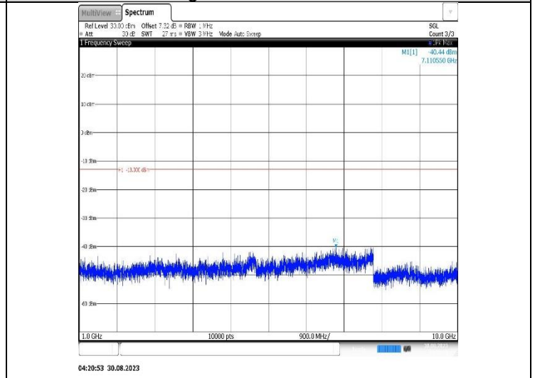
Band12-5MHz-QPSK-23095-1RB#0- Range2:1000~10000MHz
