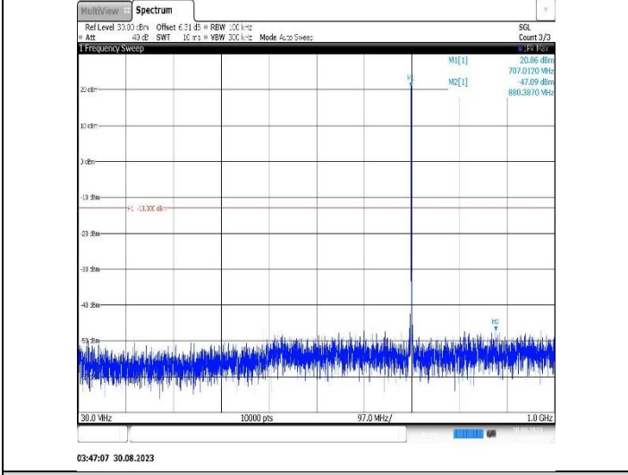
Band12-1.4MHz-QPSK-23173-1RB#0-Range1:30~1000MHz
