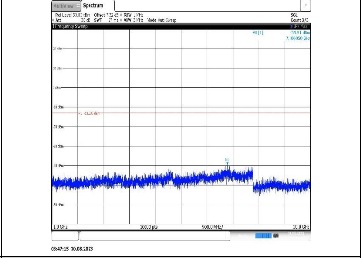
Band12-1.4MHz-QPSK-23173-1RB#0-Range2:1000~10000MHz
