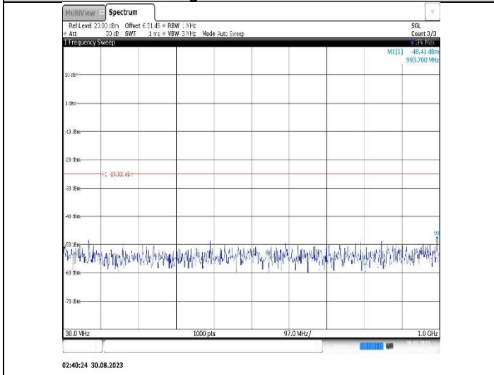
Band7-10MHz-16QAM-21100-1RB#0-Range1:30~1000MHz
