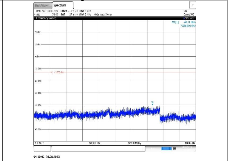
Band12-3MHz-QPSK-23095-1RB#0- Range2:1000~10000MHz
