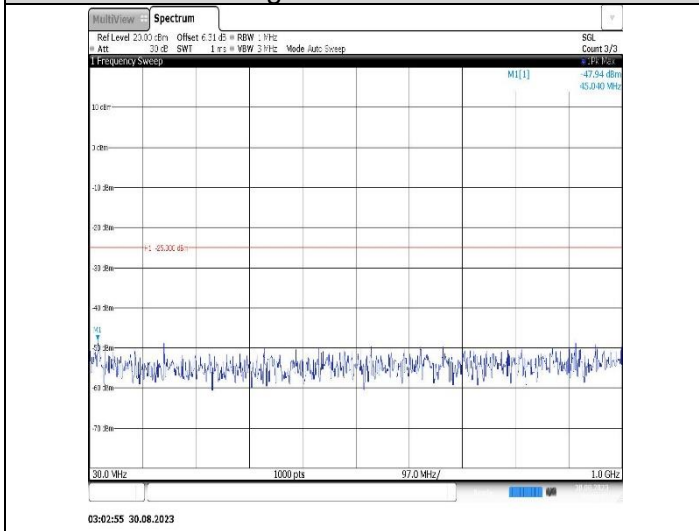
Band7-15MHz-16QAM-21375-1RB#0-Range1:30~1000MHz
