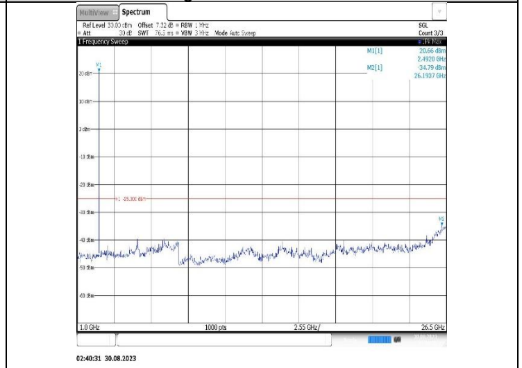
Band7-10MHz-16QAM-21100-1RB#0-Range2:1000~26500MHz
