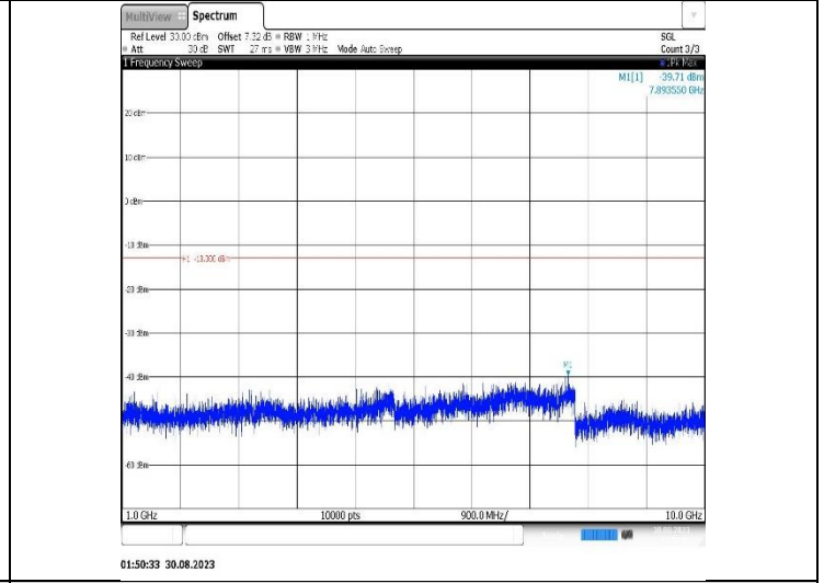
Band5-10MHz-16QAM-20600-1RB#0-Range2:1000~10000MHz
