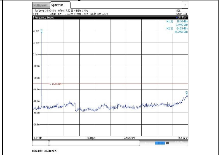
Band7-20MHz-16QAM-21100-1RB#0-Range2:1000~26500MHz
