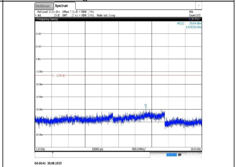
Band12-3MHz-QPSK-23165-1RB#0- Range2:1000~10000MHz
