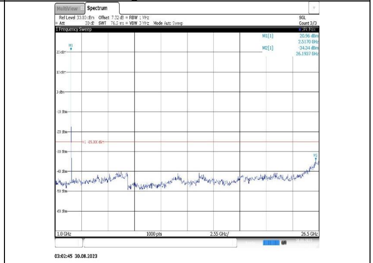
Band7-15MHz-QPSK-21375-1RB#0- Range2:1000~26500MHz
