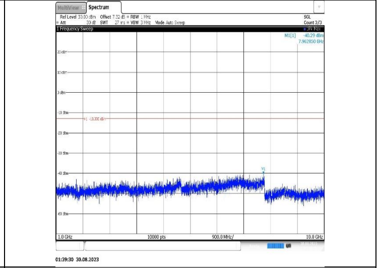
Band5-5MHz-16QAM-20625-1RB#0-Range2:1000~10000MHz
