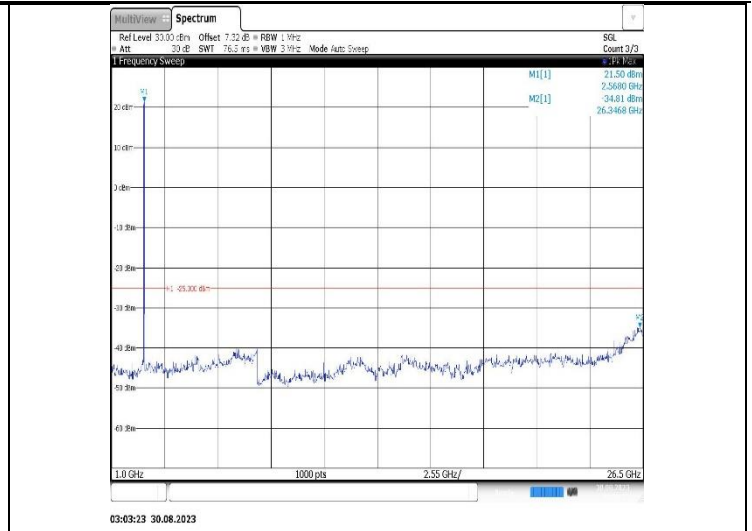
Band7-15MHz-16QAM-20825-1RB#0-Range2:1000~26500MHz
