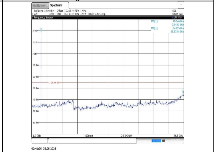
Band7-10MHz-16QAM-21400-1RB#0-Range2:1000~26500MHz
