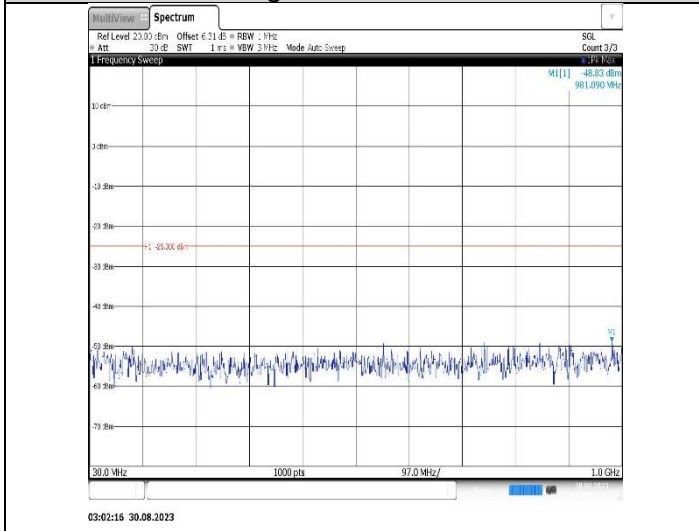
Band7-15MHz-16QAM-21100-1RB#0-Range1:30~1000MHz
