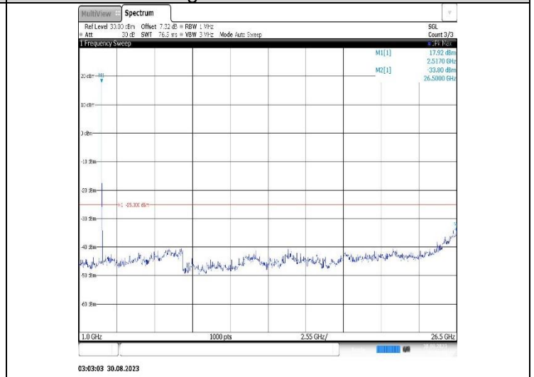
Band7-15MHz-16QAM-21375-1RB#0-Range2:1000~26500MHz
