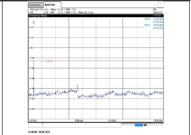
Band4-5MHz-16QAM-19975-1RB#0- Range2:1000~20000MHz
