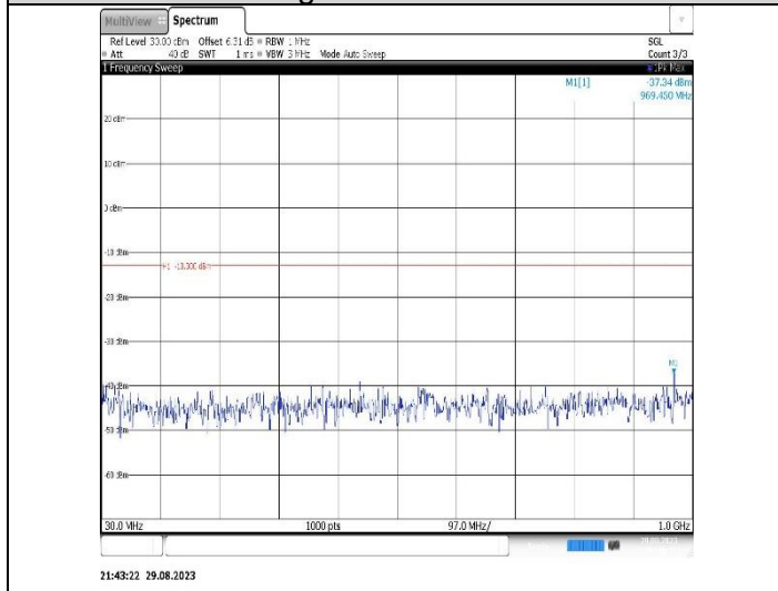
Band4-1.4MHz-16QAM-20393-1RB#0- Range1:30~1000MHz
