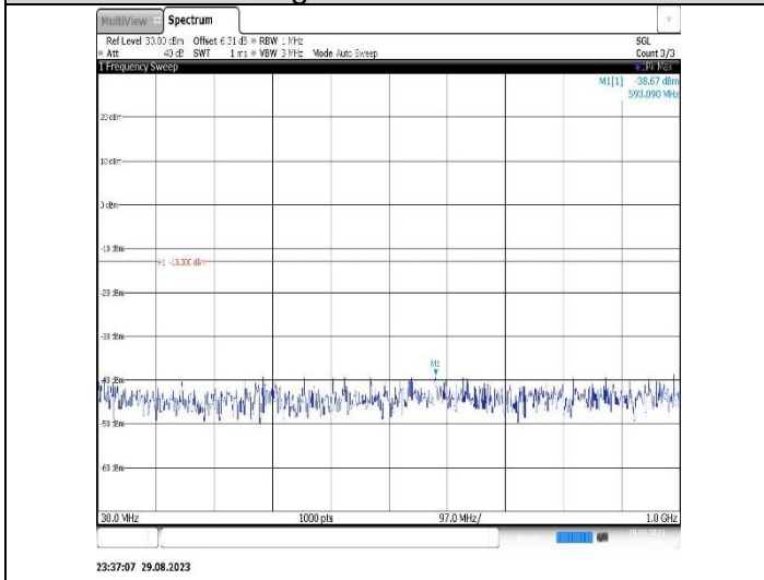
Band4-15MHz-QPSK-20325-1RB#0- Range1:30~1000MHz
