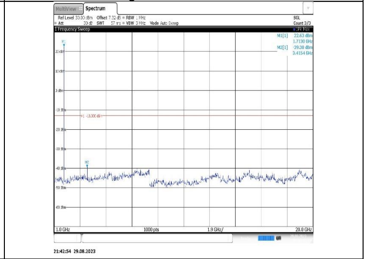
Band4-1.4MHz-16QAM-20175-1RB#0- Range2:1000~20000MHz
