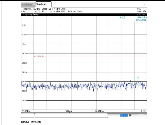
Band5-1.4MHz-QPSK-20407-1RB#0-Range1:30~1000MHz
