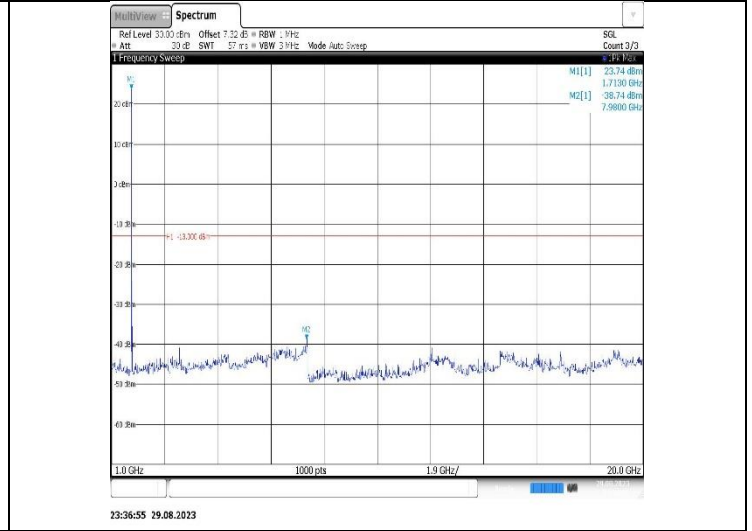
Band4-15MHz-16QAM-20175-1RB#0-Range2:1000~20000MHz
