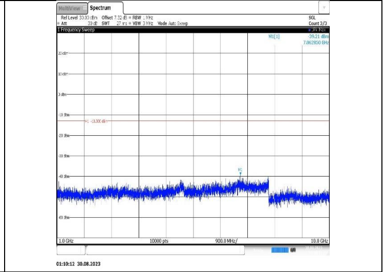
Band5-3MHz-16QAM-20525-1RB#0- Range2:1000~10000MHz
