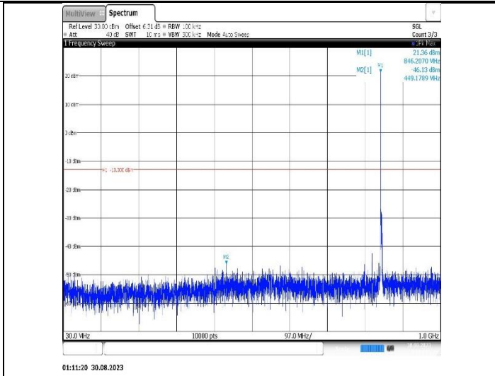
Band5-5MHz-QPSK-20425-1RB#0-Range1:30~1000MHz
