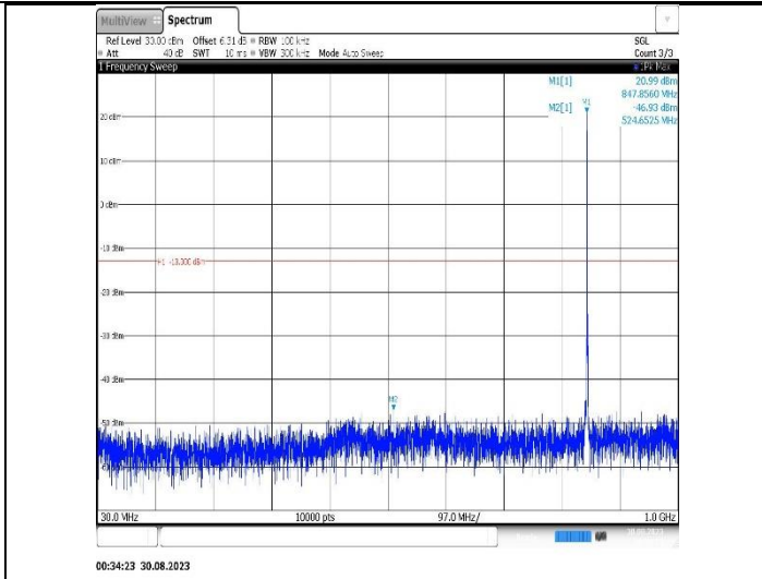
Band5-1.4MHz-16QAM-20407-1RB#0-Range1:30~1000MHz
