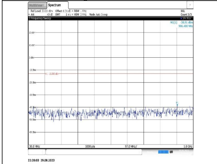
Band4-3MHz-16QAM-20385-1RB#0- Range1:30~1000MHz
