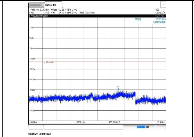
Band5-5MHz-QPSK-20425-1RB#0-Range2:1000~10000MHz
