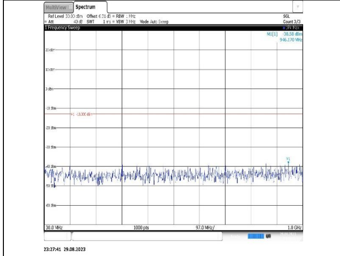
Band4-10MHz-16QAM-20350-1RB#0-Range1:30~1000MHz
