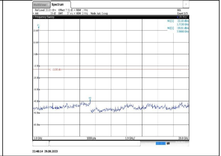
Band4-5MHz-16QAM-20175-1RB#0- Range2:1000~20000MHz
