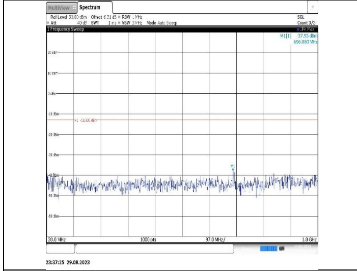
Band4-15MHz-16QAM-20325-1RB#0-Range1:30~1000MHz
