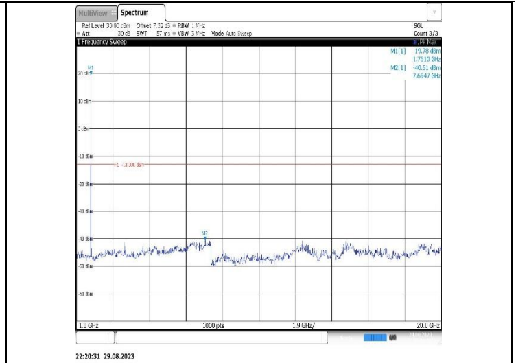
Band4-3MHz-16QAM-19965-1RB#0- Range2:1000~20000MHz
