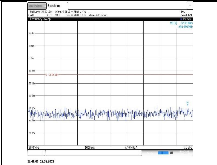
Band4-5MHz-16QAM-19975-1RB#0- Range1:30~1000MHz
