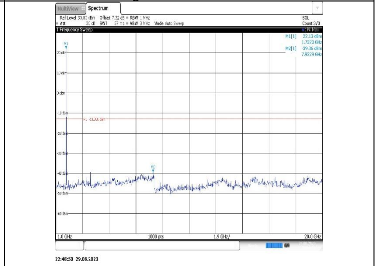
Band4-5MHz-16QAM-20375-1RB#0- Range2:1000~20000MHz
