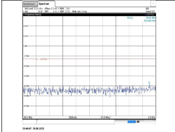
Band4-20MHz-16QAM-20175-1RB#0-Range1:30~1000MHz
