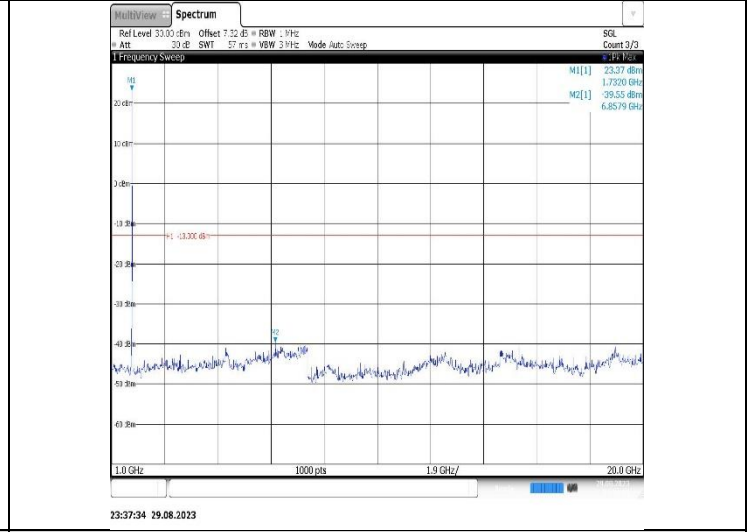
Band4-15MHz-16QAM-20325-1RB#0-Range2:1000~20000MHz
