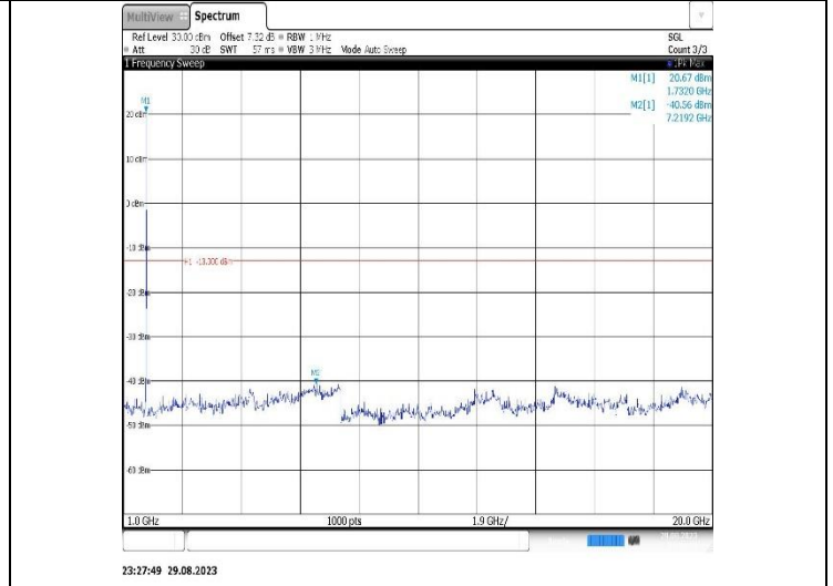
Band4-10MHz-16QAM-20350-1RB#0-Range2:1000~20000MHz
