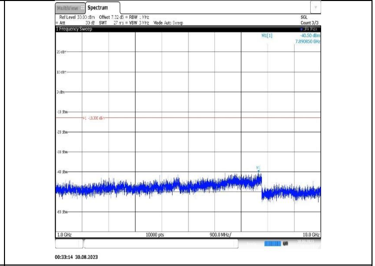
Band5-1.4MHz-QPSK-20525-1RB#0-Range2:1000~10000MHz
