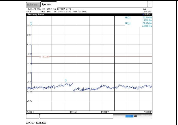
Band4-20MHz-16QAM-20050-1RB#0-Range2:1000~20000MHz
