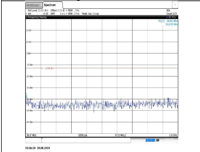
Band4-15MHz-QPSK-20175-1RB#0- Range1:30~1000MHz
