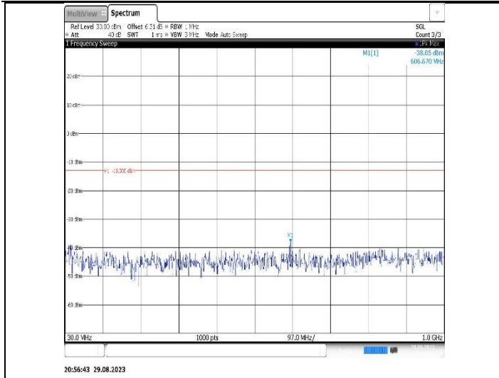
Band4-1.4MHz-QPSK-19957-1RB#0- Range1:30~1000MHz
