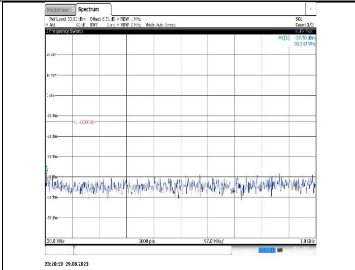
Band4-15MHz-QPSK-20025-1RB#0- Range1:30~1000MHz
