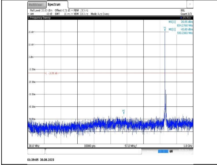
Band5-5MHz-QPSK-20625-1RB#0-Range1:30~1000MHz
