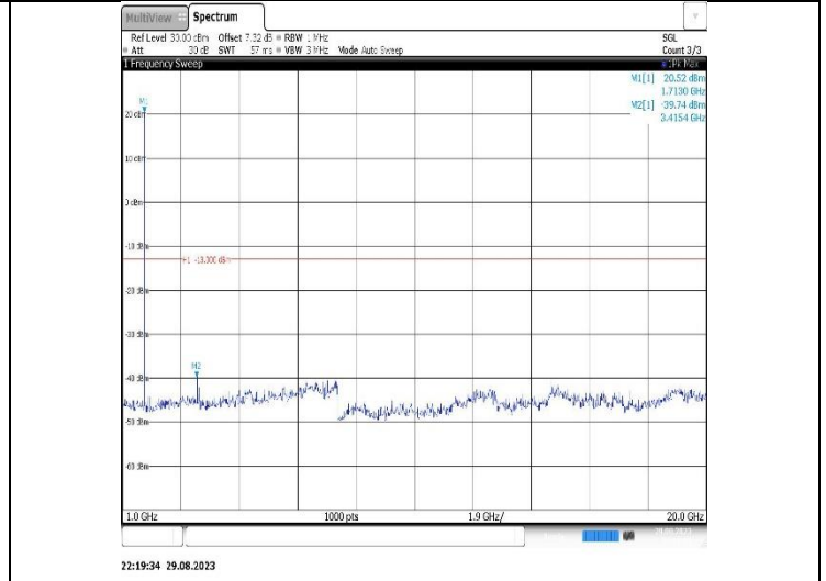
Band4-3MHz-16QAM-20175-1RB#0- Range2:1000~20000MHz
