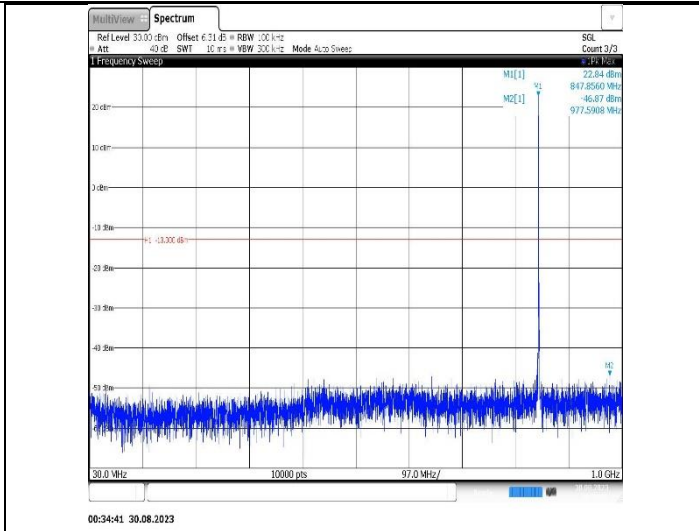
Band5-3MHz-QPSK-20415-1RB#0-Range1:30~1000MHz
