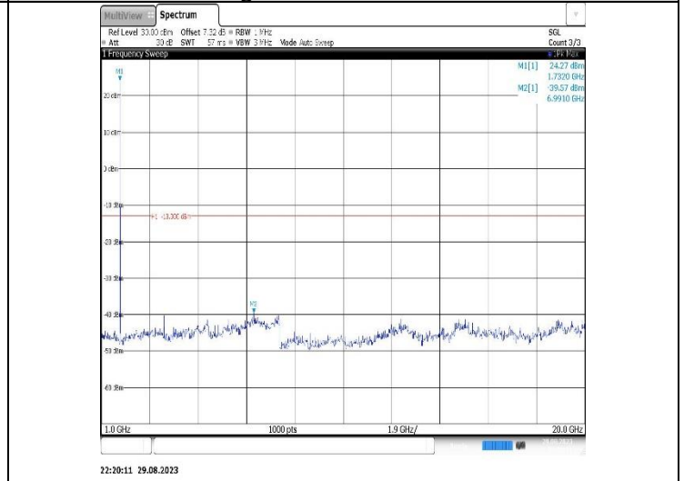
Band4-3MHz-16QAM-20385-1RB#0- Range2:1000~20000MHz
