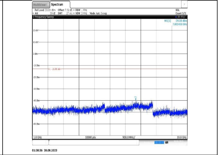
Band5-5MHz-QPSK-20525-1RB#0-Range2:1000~10000MHz
