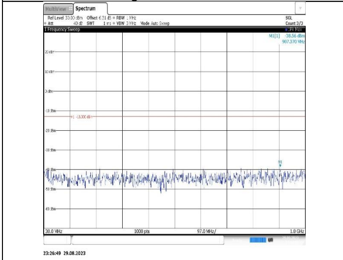
Band4-10MHz-QPSK-20175-1RB#0- Range1:30~1000MHz
