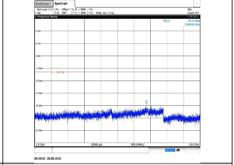
Band5-1.4MHz-QPSK-20643-1RB#0-Range2:1000~10000MHz
