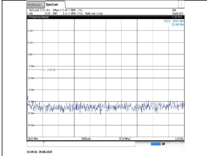
Band4-3MHz-16QAM-20175-1RB#0- Range1:30~1000MHz
