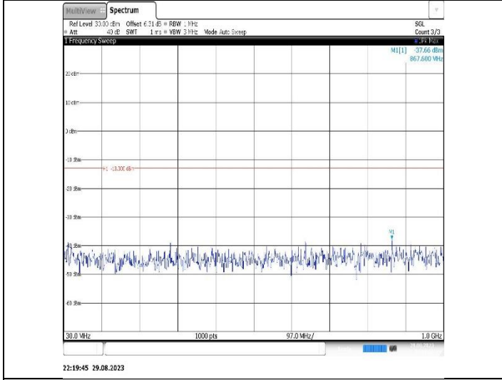
Band4-3MHz-QPSK-20385-1RB#0-Range1:30~1000MHz
