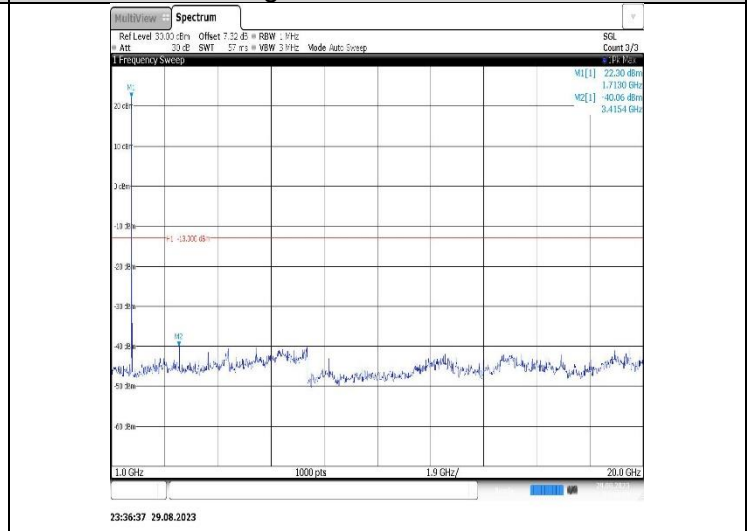
Band4-15MHz-QPSK-20175-1RB#0- Range2:1000~20000MHz
