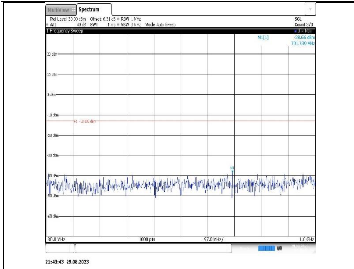
Band4-1.4MHz-16QAM-19957-1RB#0- Range1:30~1000MHz
