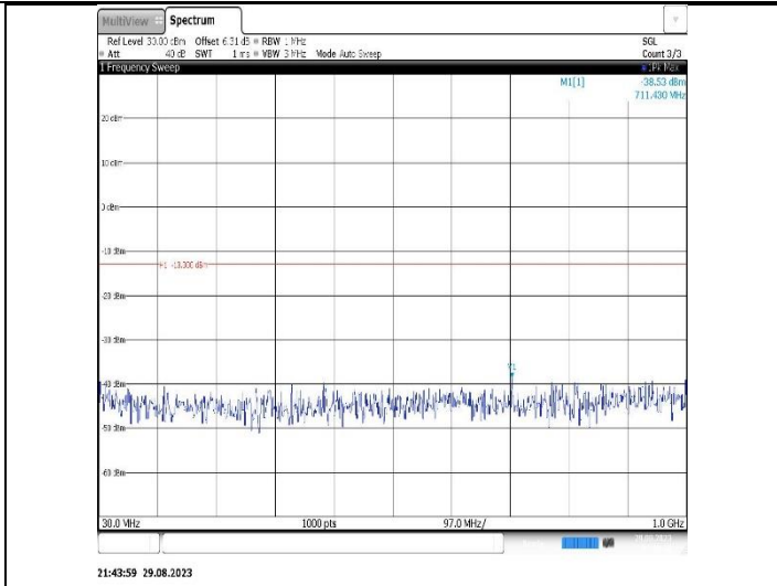
Band4-3MHz-QPSK-19965-1RB#0-Range1:30~1000MHz
