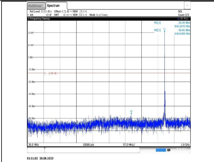
Band5-3MHz-16QAM-20415-1RB#0- Range1:30~1000MHz
