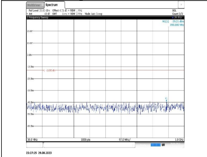
Band4-10MHz-QPSK-20350-1RB#0- Range1:30~1000MHz
