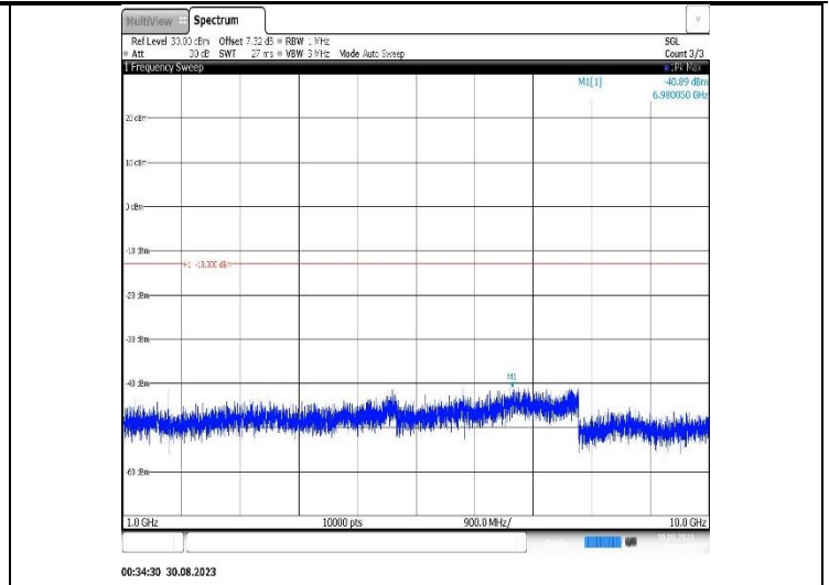
Band5-1.4MHz-16QAM-20407-1RB#0-Range2:1000~10000MHz
