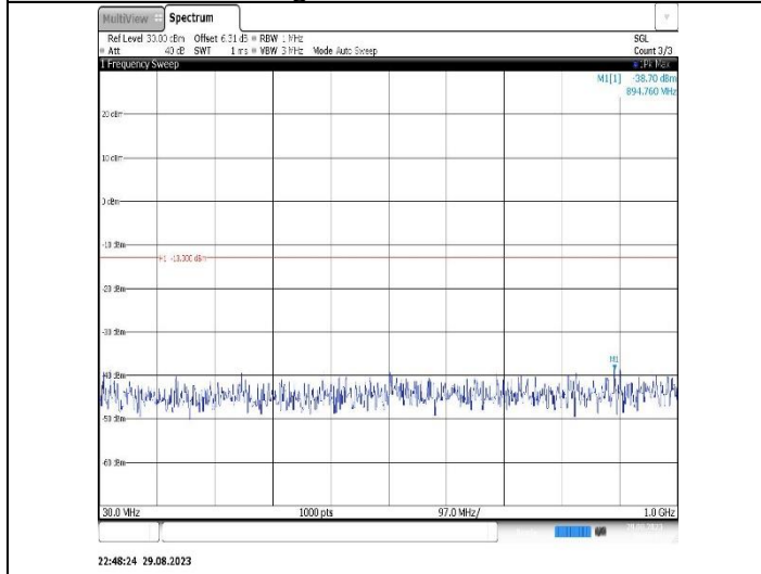
Band4-5MHz-QPSK-20375-1RB#0-Range1:30~1000MHz
