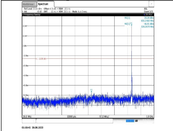
Band5-3MHz-16QAM-20635-1RB#0- Range1:30~1000MHz
