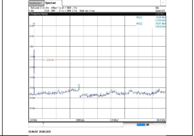
Band4-20MHz-16QAM-20300-1RB#0-Range2:1000~20000MHz
