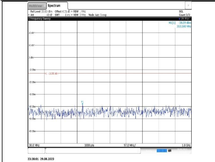
Band4-10MHz-16QAM-20000-1RB#0-Range1:30~1000MHz
