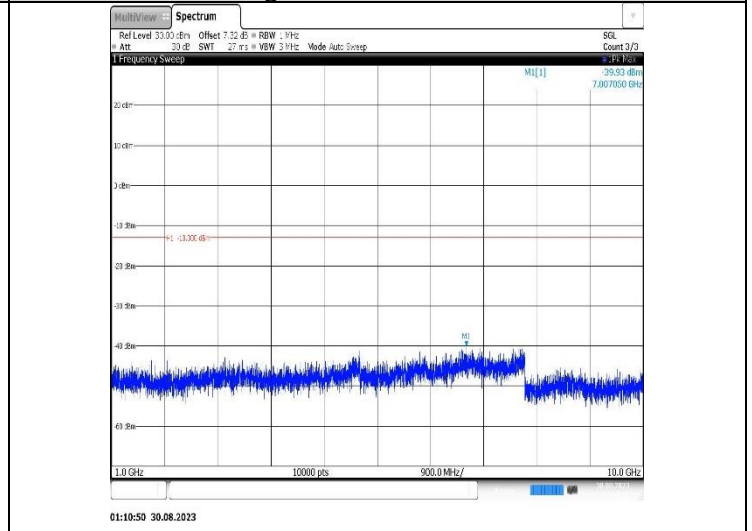
Band5-3MHz-16QAM-20635-1RB#0- Range2:1000~10000MHz
