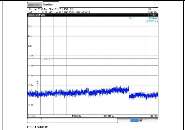
Band5-3MHz-16QAM-20415-1RB#0- Range2:1000~10000MHz
