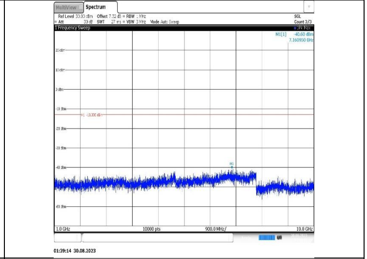
Band5-5MHz-QPSK-20625-1RB#0-Range2:1000~10000MHz
