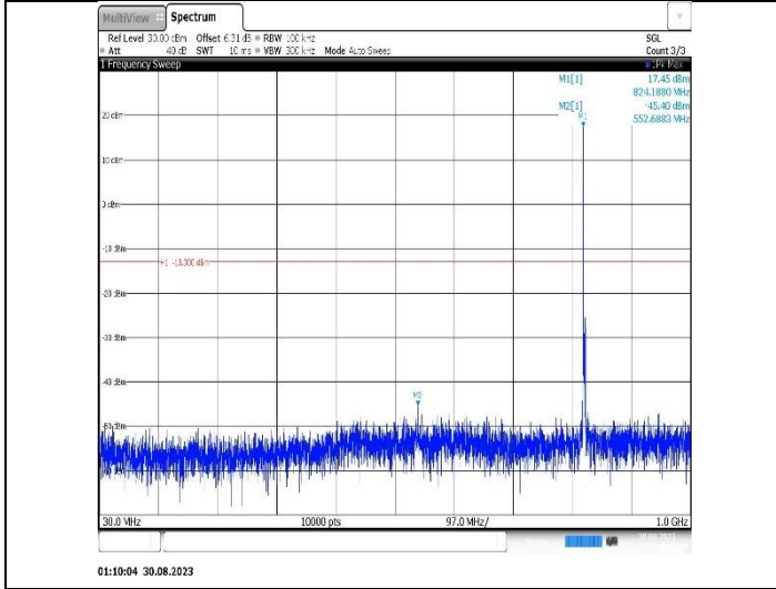
Band5-3MHz-16QAM-20525-1RB#0- Range1:30~1000MHz
