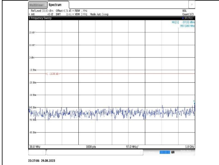
Band4-10MHz-16QAM-20175-1RB#0-Range1:30~1000MHz
