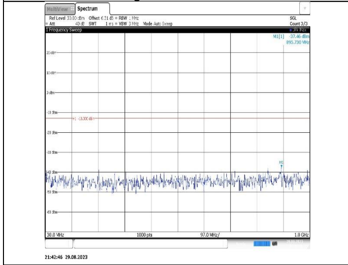
Band4-1.4MHz-16QAM-20175-1RB#0- Range1:30~1000MHz
