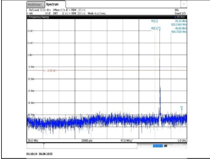
Band5-3MHz-QPSK-20635-1RB#0-Range1:30~1000MHz
