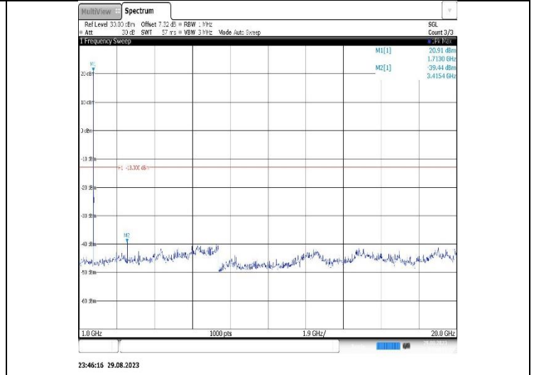
Band4-20MHz-16QAM-20175-1RB#0-Range2:1000~20000MHz
