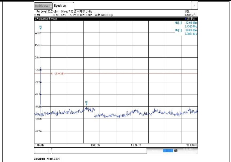
Band4-10MHz-16QAM-20000-1RB#0-Range2:1000~20000MHz
