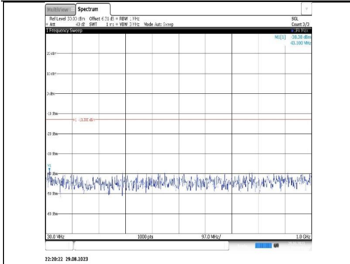
Band4-3MHz-16QAM-19965-1RB#0- Range1:30~1000MHz
