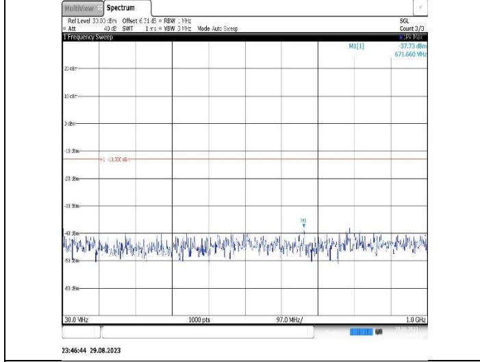
Band4-20MHz-16QAM-20300-1RB#0-Range1:30~1000MHz
