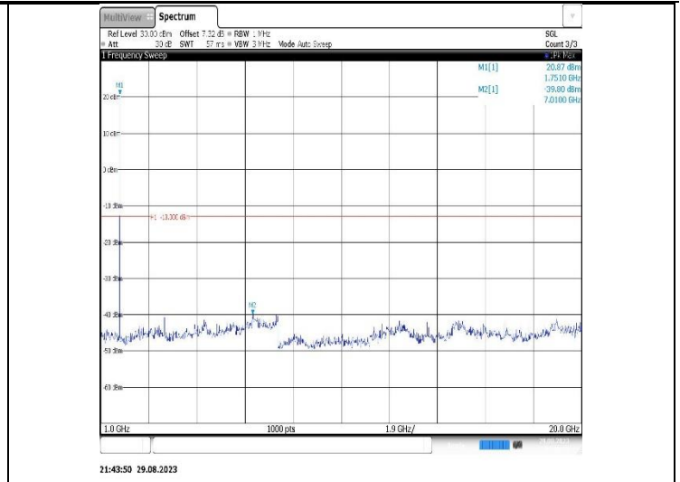
Band4-1.4MHz-16QAM-19957-1RB#0- Range2:1000~20000MHz
