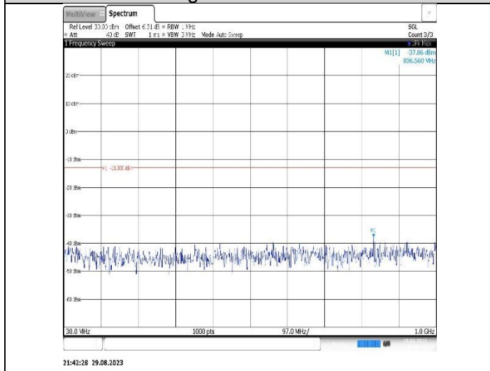
Band4-1.4MHz-QPSK-20175-1RB#0- Range1:30~1000MHz
