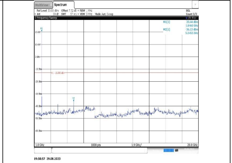
Band2-3MHz-16QAM-18900-1RB#0-Range2:1000~20000MHz
