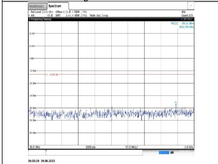
Band2-20MHz-16QAM-18900-1RB#0-Range1:30~1000MHz
