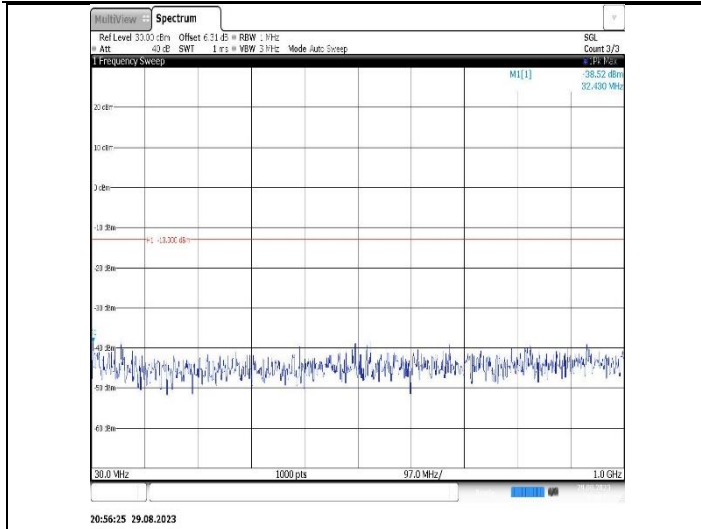
Band2-20MHz-16QAM-18700-1RB#0-Range1:30~1000MHz
