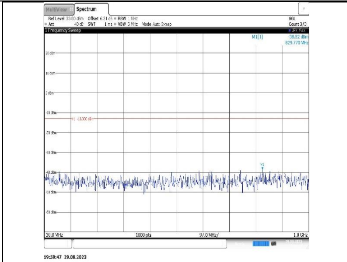
Band2-3MHz-16QAM-18615-1RB#0-Range1:30~1000MHz
