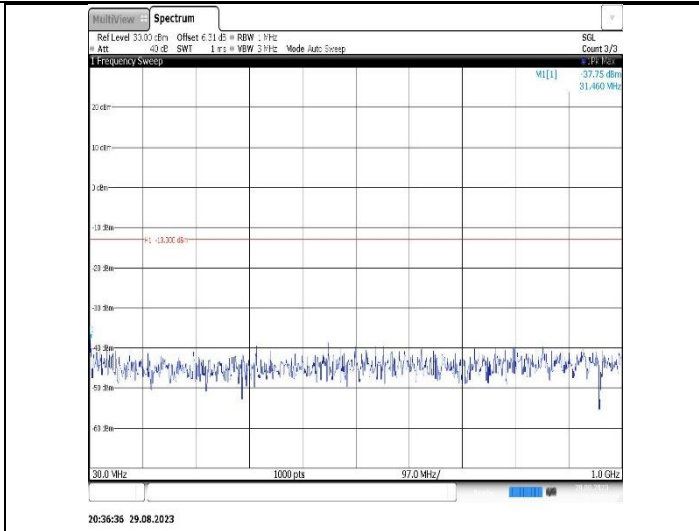
Band2-15MHz-QPSK-18675-1RB#0- Range1:30~1000MHz
