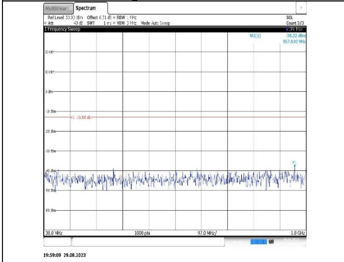
Band2-3MHz-QPSK-19185-1RB#0-Range1:30~1000MHz
