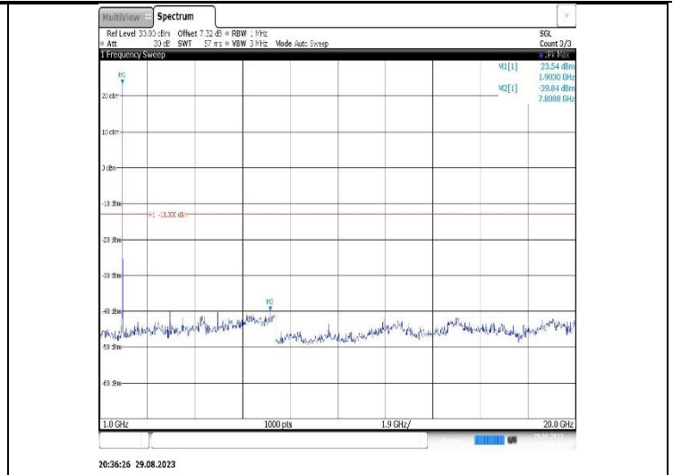
Band2-10MHz-16QAM-18650-1RB#0-Range2:1000~20000MHz
