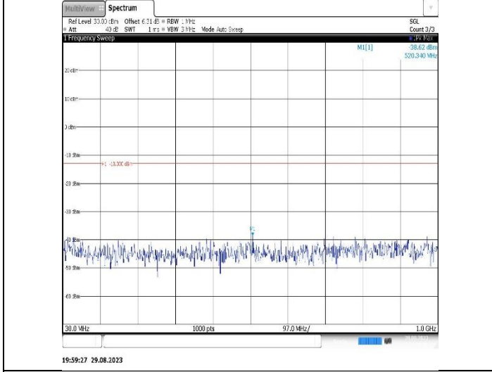
Band2-3MHz-16QAM-19185-1RB#0-Range1:30~1000MHz
