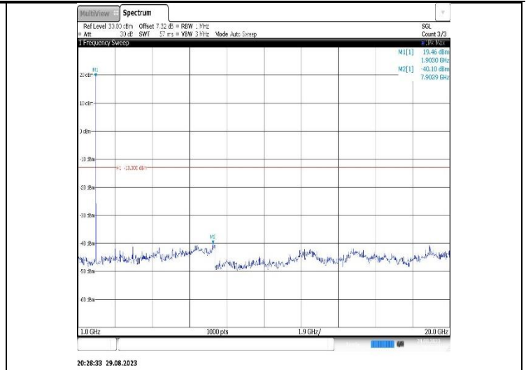
Band2-5MHz-16QAM-18625-1RB#0- Range2:1000~20000MHz
