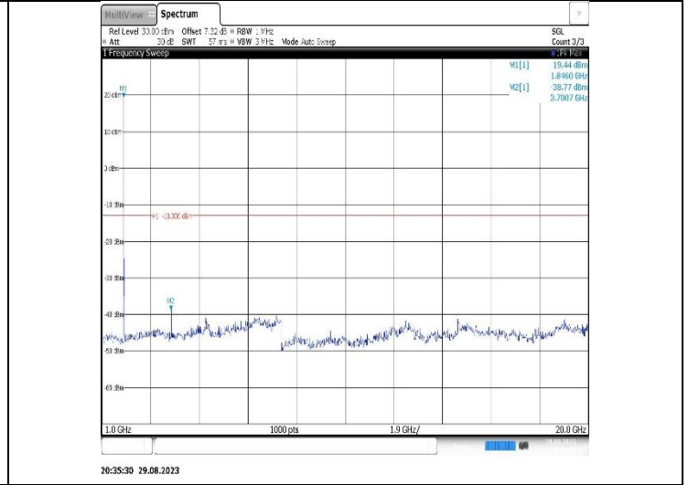
Band2-10MHz-16QAM-18900-1RB#0-Range2:1000~20000MHz
