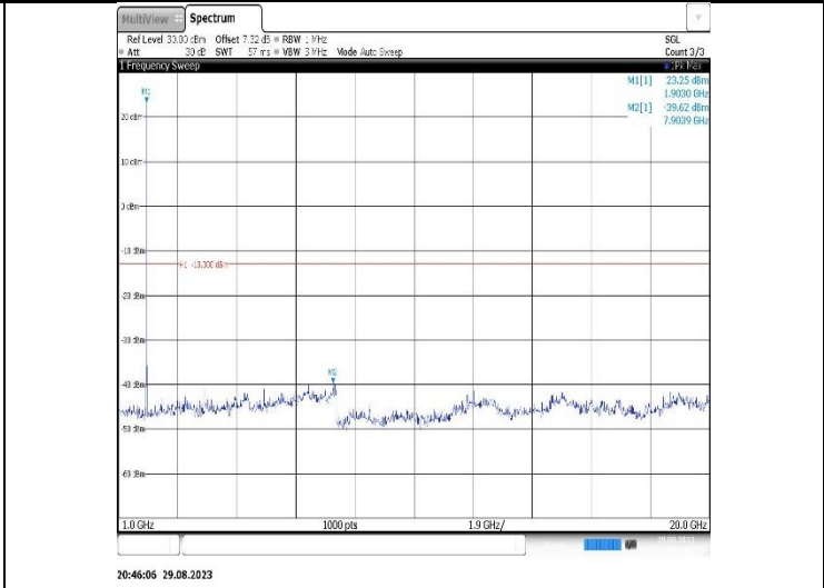
Band2-15MHz-16QAM-18675-1RB#0-Range2:1000~20000MHz
