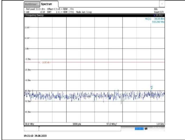
Band2-1.4MHz-16QAM-18900-1RB#0- Range1:30~1000MHz
