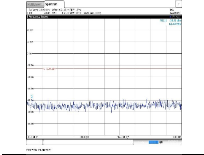
Band2-5MHz-QPSK-19175-1RB#0-Range1:30~1000MHz
