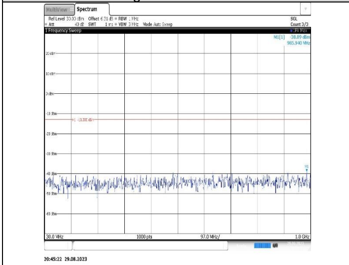
Band2-15MHz-QPSK-19125-1RB#0- Range1:30~1000MHz
