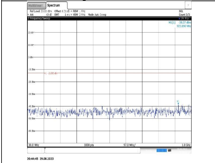
Band2-15MHz-QPSK-18900-1RB#0- Range1:30~1000MHz
