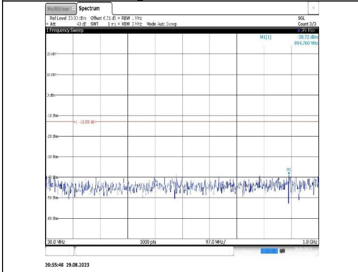
Band2-20MHz-QPSK-19100-1RB#0- Range1:30~1000MHz
