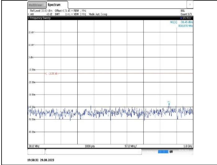
Band2-3MHz-QPSK-18900-1RB#0-Range1:30~1000MHz
