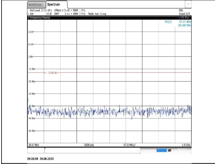
Band2-10MHz-16QAM-19150-1RB#0-Range1:30~1000MHz
