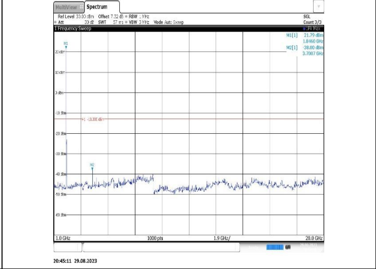
Band2-15MHz-16QAM-18900-1RB#0-Range2:1000~20000MHz
