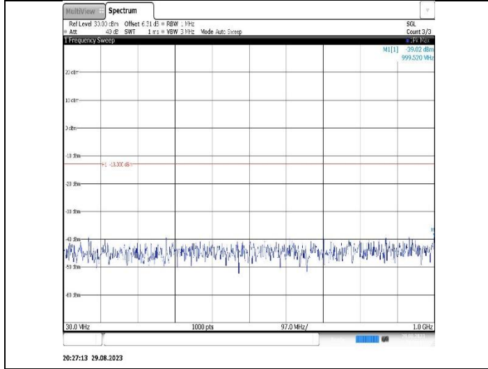
Band2-5MHz-QPSK-18900-1RB#0-Range1:30~1000MHz
