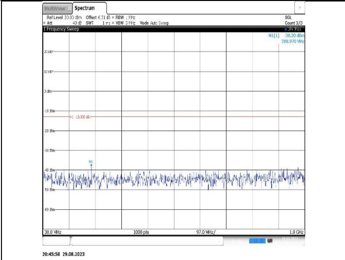
Band2-15MHz-16QAM-18675-1RB#0-Range1:30~1000MHz
