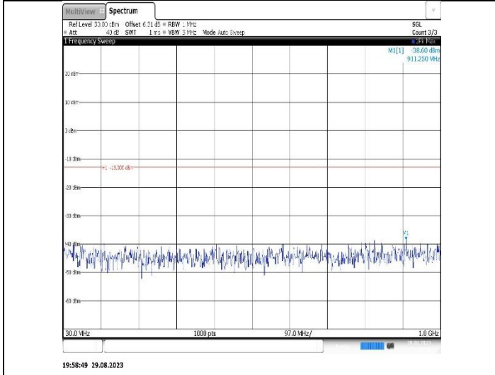
Band2-3MHz-16QAM-18900-1RB#0-Range1:30~1000MHz
