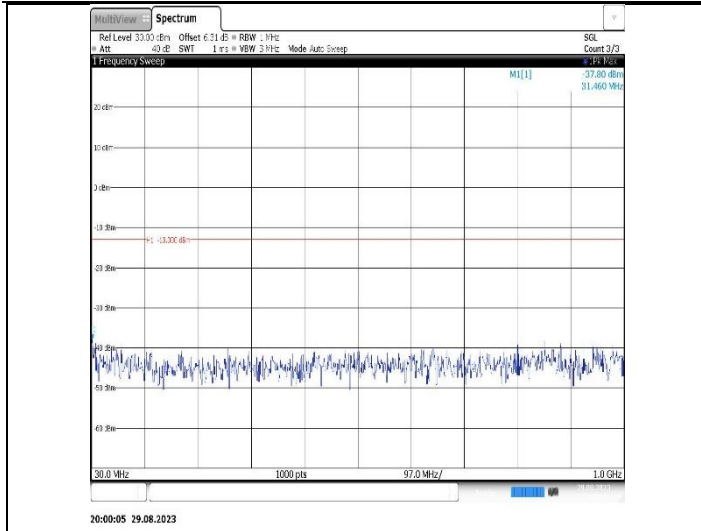
Band2-5MHz-QPSK-18625-1RB#0-Range1:30~1000MHz
