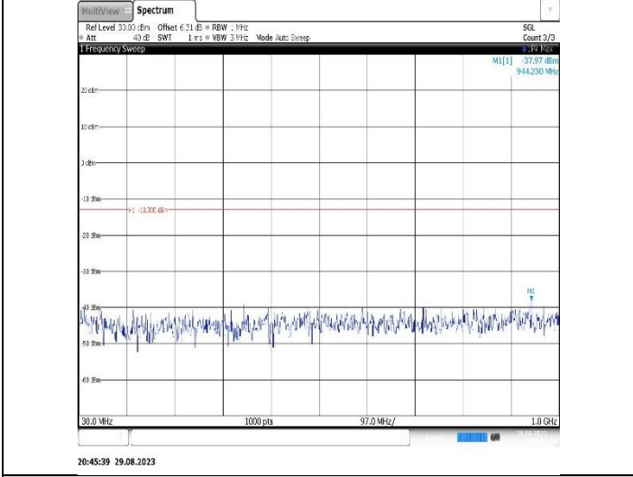
Band2-15MHz-16QAM-19125-1RB#0-Range1:30~1000MHz
