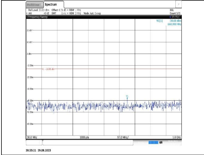
Band2-10MHz-16QAM-18900-1RB#0-Range1:30~1000MHz
