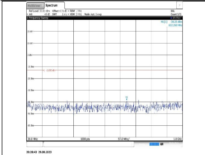
Band2-10MHz-QPSK-18650-1RB#0-Range1:30~1000MHz
