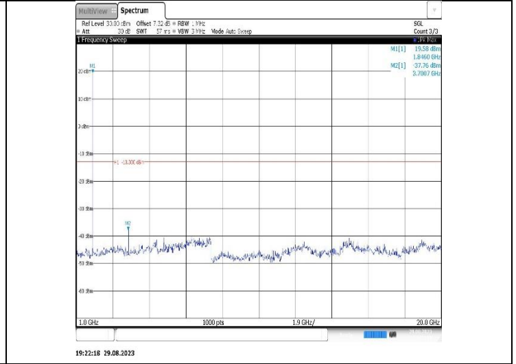
Band2-1.4MHz-16QAM-18900-1RB#0- Range2:1000~20000MHz
