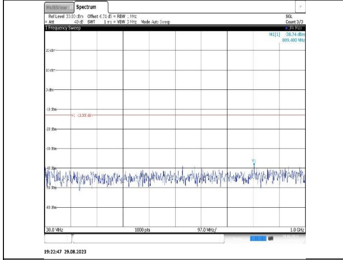
Band2-1.4MHz-16QAM-19193-1RB#0- Range1:30~1000MHz
