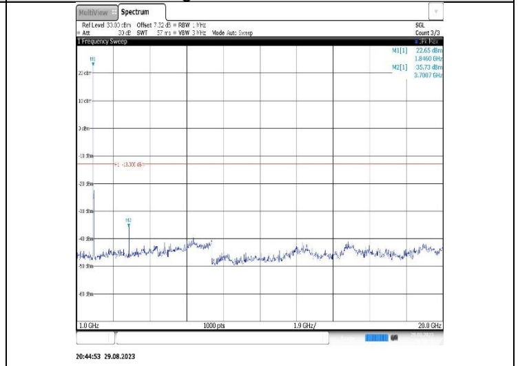
Band2-15MHz-QPSK-18900-1RB#0- Range2:1000~20000MHz
