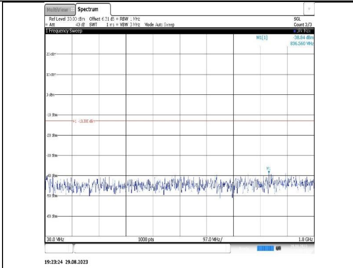
Band2-3MHz-QPSK-18615-1RB#0-Range1:30~1000MHz
