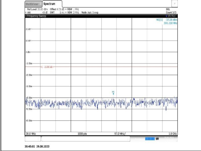
Band2-15MHz-16QAM-18900-1RB#0-Range1:30~1000MHz
