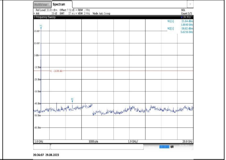
Band2-10MHz-16QAM-19150-1RB#0-Range2:1000~20000MHz
