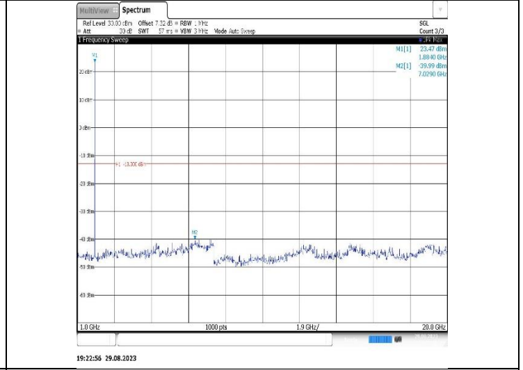
Band2-1.4MHz-16QAM-19193-1RB#0- Range2:1000~20000MHz
