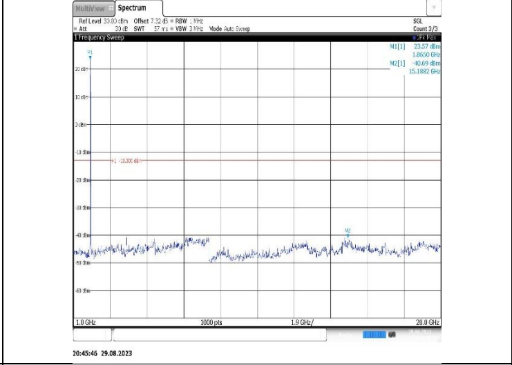
Band2-15MHz-16QAM-19125-1RB#0-Range2:1000~20000MHz
