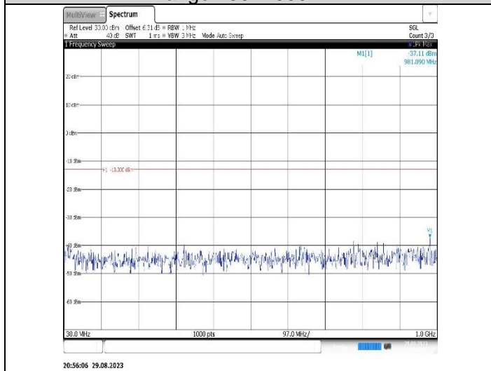
Band2-20MHz-16QAM-19100-1RB#0-Range1:30~1000MHz
