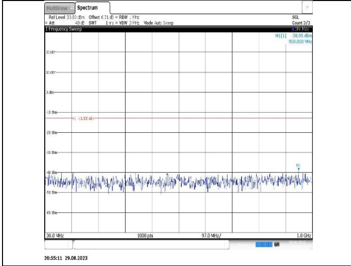
Band2-20MHz-QPSK-18900-1RB#0- Range1:30~1000MHz
