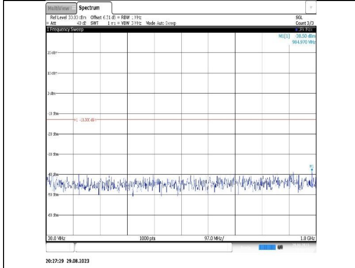
Band2-5MHz-16QAM-18900-1RB#0- Range1:30~1000MHz
