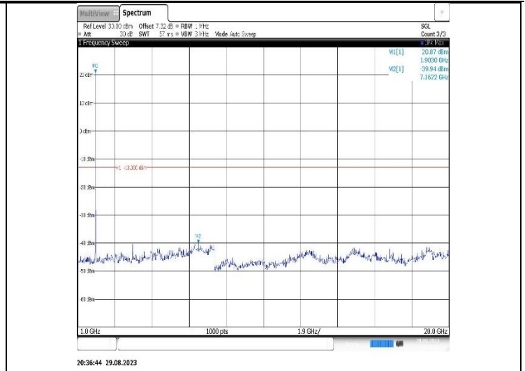
Band2-15MHz-QPSK-18675-1RB#0- Range2:1000~20000MHz
