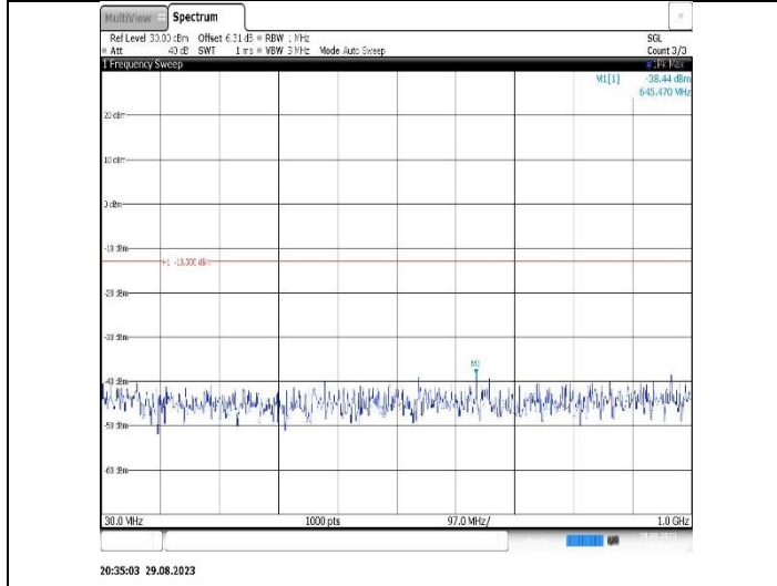
Band2-10MHz-QPSK-18900-1RB#0-Range1:30~1000MHz
