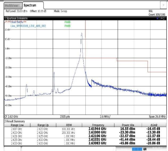
Band38-10MHz-QPSK-38200-1RB#49
