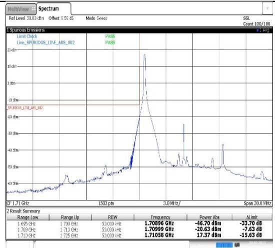
Band66-10MHz-QPSK-132022-1RB#0
