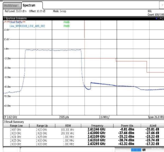
Band38-10MHz-QPSK-38200-50RB#0
