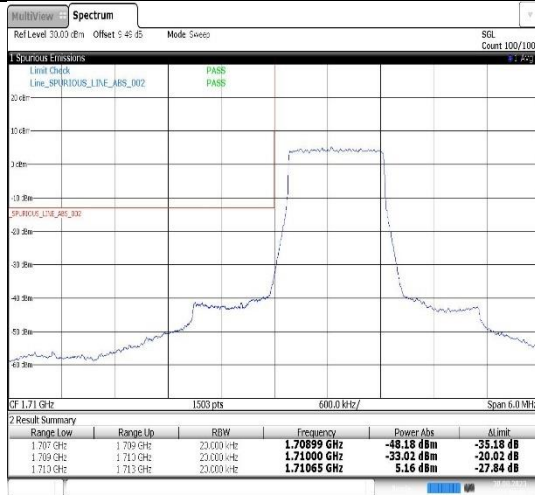
Band66-1.4MHz-QPSK-131979-6RB#0
