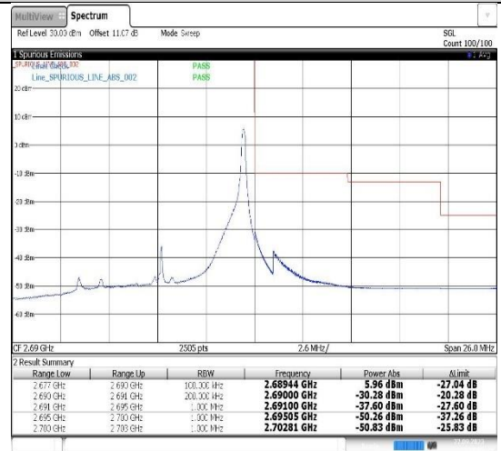
Band41-10MHz-16QAM-41540-1RB#49
