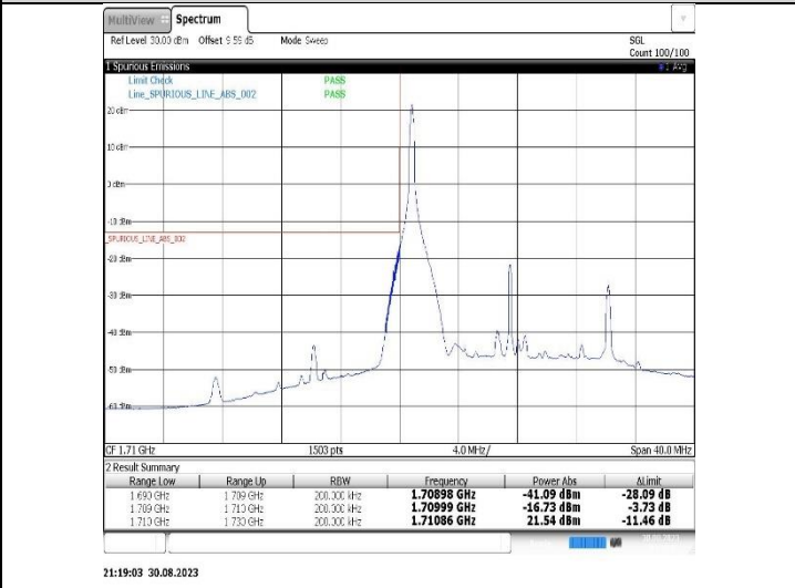
Band66-15MHz-16QAM-132047-1RB#74
