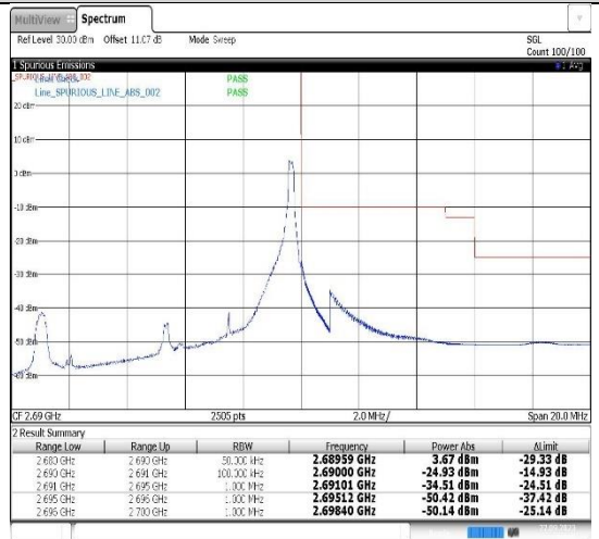
Band41-5MHz-QPSK-41565-1RB#24
