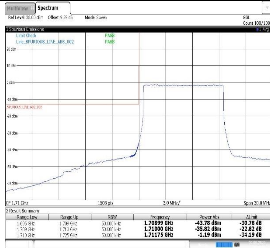
Band66-10MHz-16QAM-132022-50RB#0
