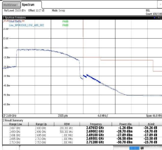
Band41-20MHz-16QAM-41490-100RB#0
