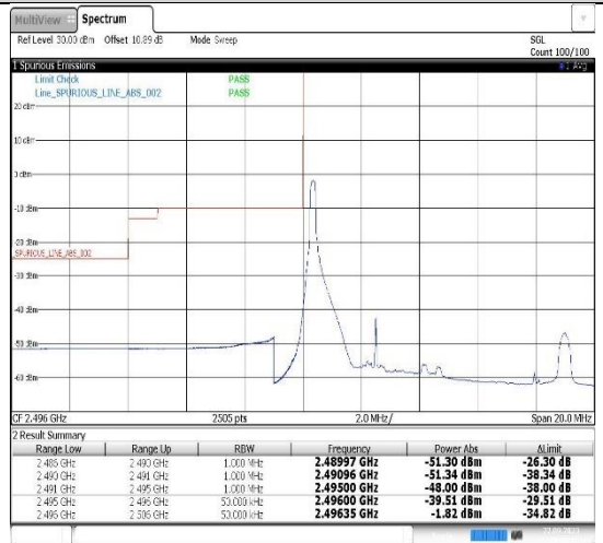
Band41-5MHz-16QAM-39675-1RB#0
