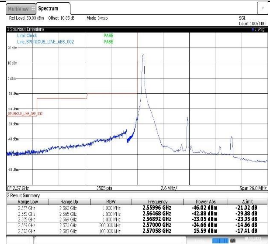
Band38-10MHz-16QAM-37800-1RB#0
