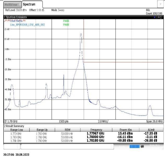
Band66-10MHz-QPSK-132022-1RB#0
