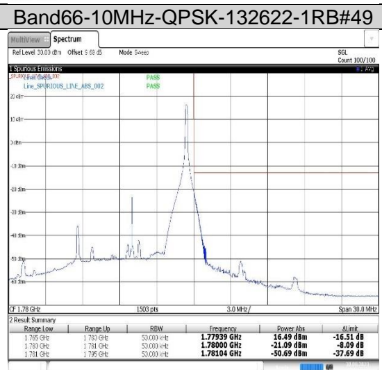
Band66-10MHz-QPSK-132622-1RB#49
