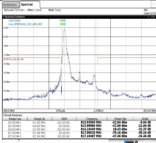
Band26(814-824)-3MHz-16QAM-26705-1RB#0
