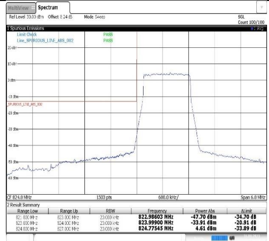
Band26(824-849)-1.4MHz-QPSK-26797-6RB#0
