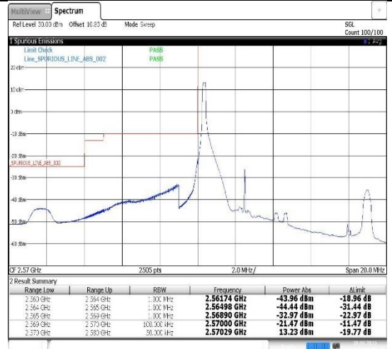
Band38-5MHz-QPSK-37775-1RB#0
