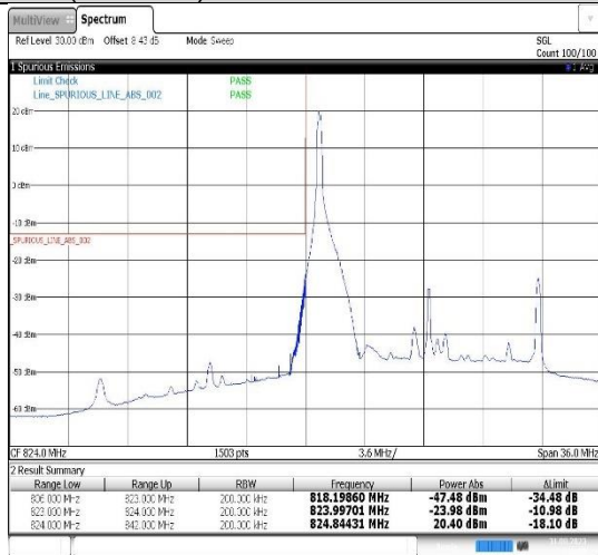
Band26(824-849)-15MHz-16QAM-26865-1RB#0
