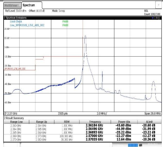
Band38-5MHz-16QAM-37775-1RB#0
