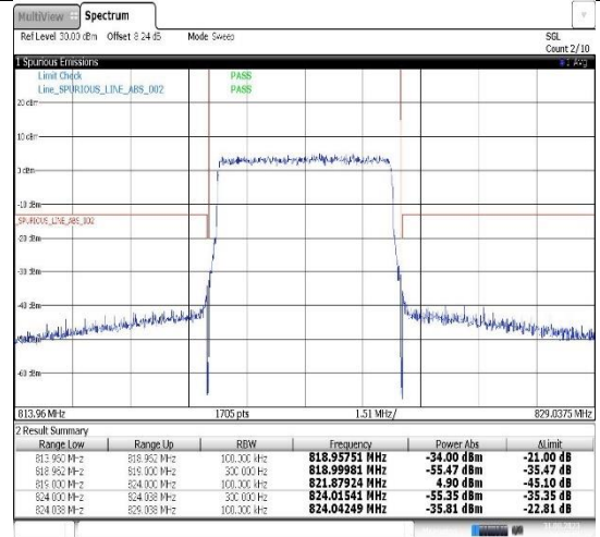
Band26(814-824)-10MHz-QPSK-26740-1RB#49
