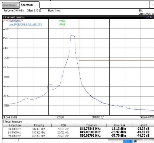
Band26(824-849)-1.4MHz-16QAM-27033-1RB#5
