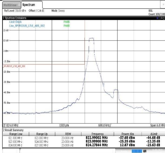
Band26(824-849)-1.4MHz-QPSK-26797-1RB#0
