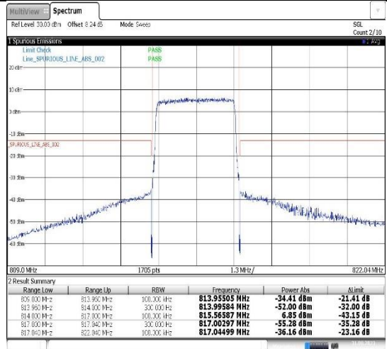
Band26(814-824)-3MHz-16QAM-26705-15RB#0
