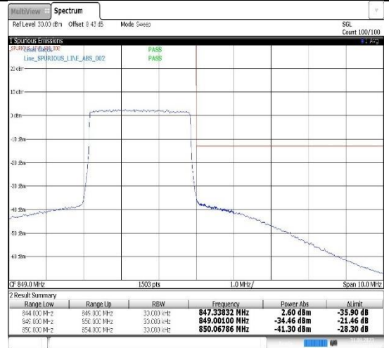
Band26(824-849)-3MHz-16QAM-27025-15RB#0
