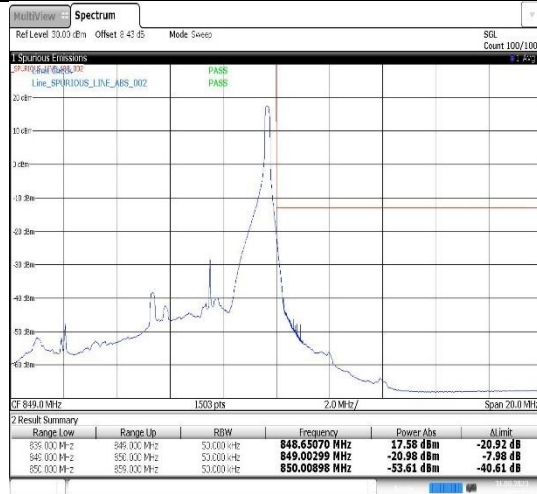
13:08:12 31.08.2023 Band26(824-849)-5MHz-16QAM-26815-1RB#0
