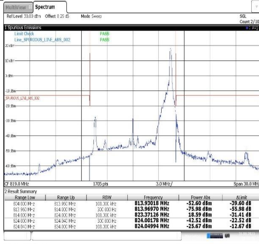
Band26(824-849)-1.4MHz-QPSK-26797-1RB#0
