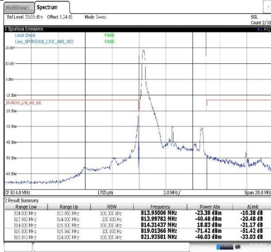
Band26(814-824)-5MHz-QPSK-26765-1RB#24
