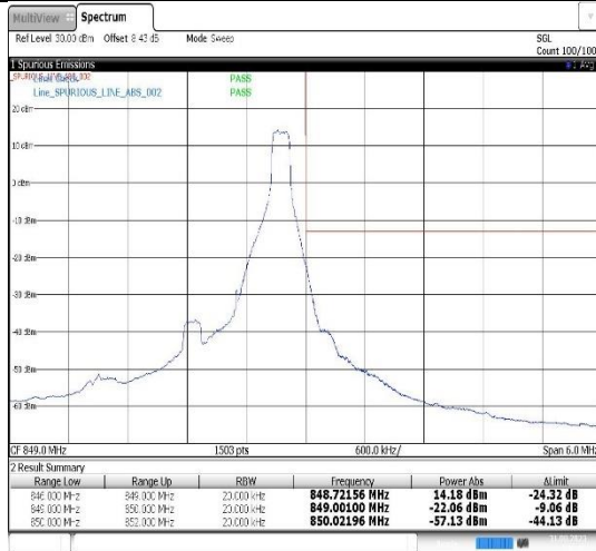
Band26(824-849)-1.4MHz-QPSK-27033-1RB#5
