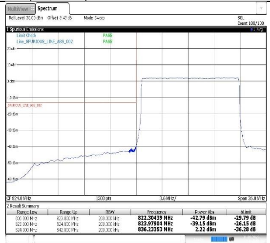
Band26(824-849)-15MHz-16QAM-26865-75RB#0
