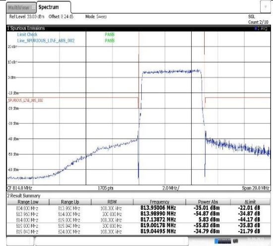
Band26(814-824)-5MHz-QPSK-26765-25RB#0
