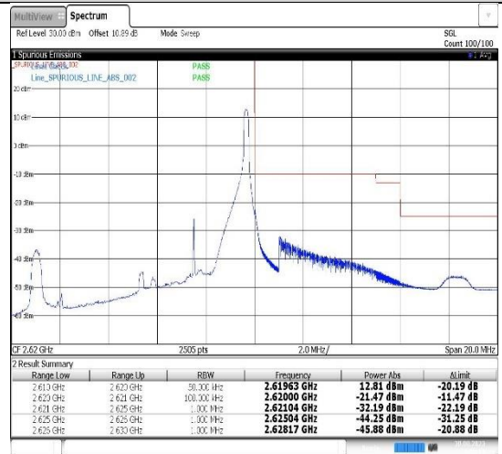
Band38-5MHz-16QAM-38225-1RB#24
