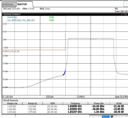
Band25-20MHz-16QAM-26140-100RB#0
