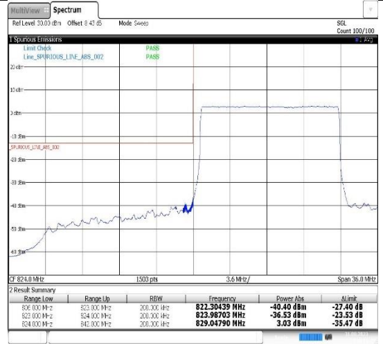
Band26(824-849)-15MHz-16QAM-26865-75RB#0
