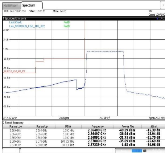
Band38-5MHz-16QAM-37775-25RB#0
