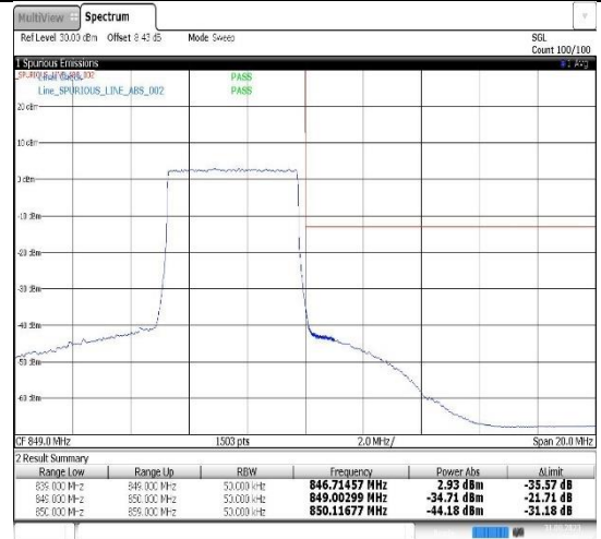
13:13:42 31.08.2023 Band26(824-849)-5MHz-16QAM-26815-25RB#0
