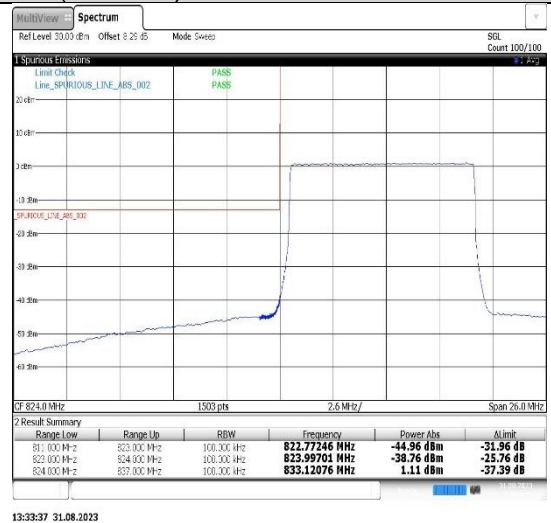
Band26(824-849)-15MHz-QPSK-26865-75RB#0
