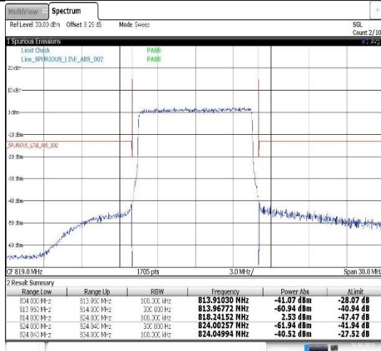
Band26(814-824)-10MHz-QPSK-26740-50RB#0
