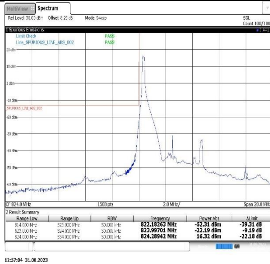
12:57:04 31.08.2023 Band26(824-849)-5MHz-QPSK-27015-1RB#24
