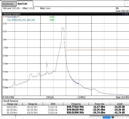
Band26(824-849)-3MHz-16QAM-27025-1RB#14
