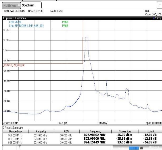
Band26(824-849)-3MHz-16QAM-26805-1RB#0
