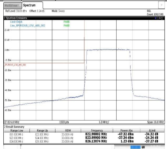
Band26(824-849)-3MHz-16QAM-26805-15RB#0
