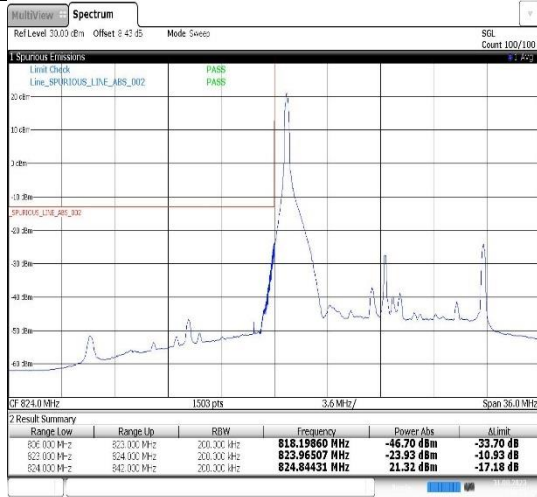
Band26(824-849)-15MHz-16QAM-26865-1RB#0
