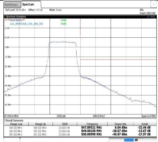
Band26(824-849)-1.4MHz-QPSK-27033-6RB#0
