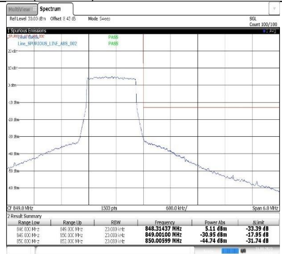
Band26(824-849)-1.4MHz-16QAM-27033-6RB#0
