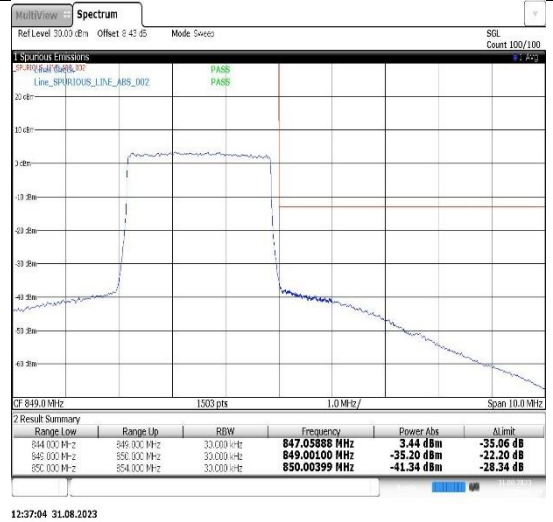
Band26(824-849)-3MHz-16QAM-26805-15RB#0
