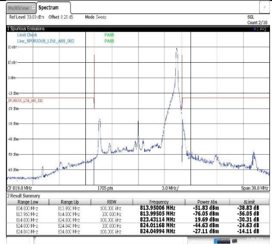
Band26(814-824)-10MHz-QPSK-26740-1RB#49
