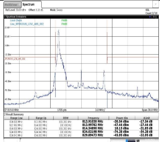
Band26(814-824)-10MHz-16QAM-26740-1RB#0
