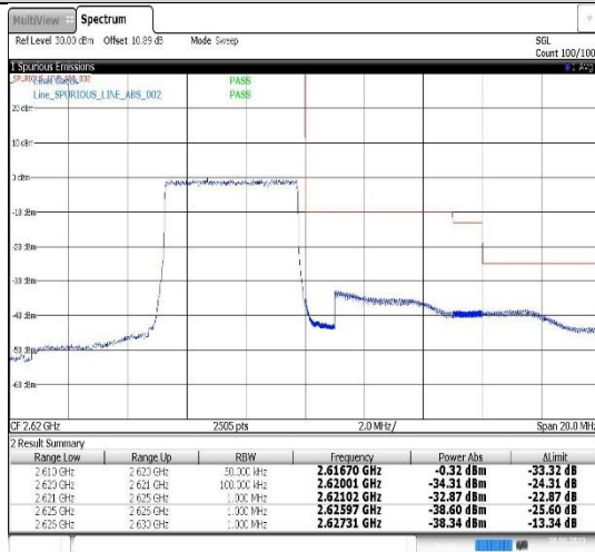
Band38-5MHz-QPSK-38225-25RB#0
