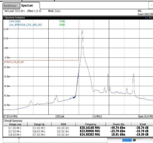
Band26(824-849)-10MHz-QPSK-26840-1RB#0
