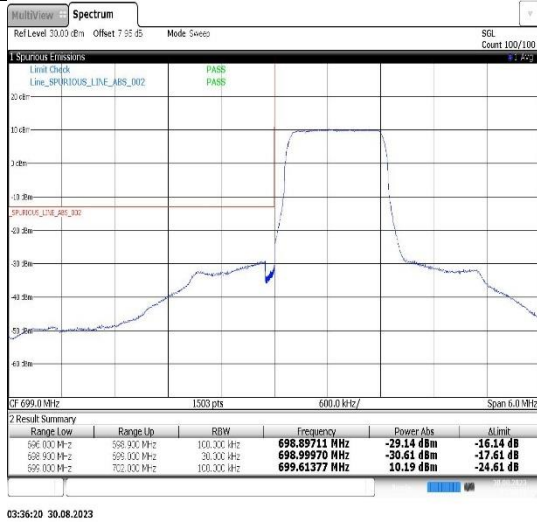
Band12-1.4MHz-QPSK-23173-6RB#0
