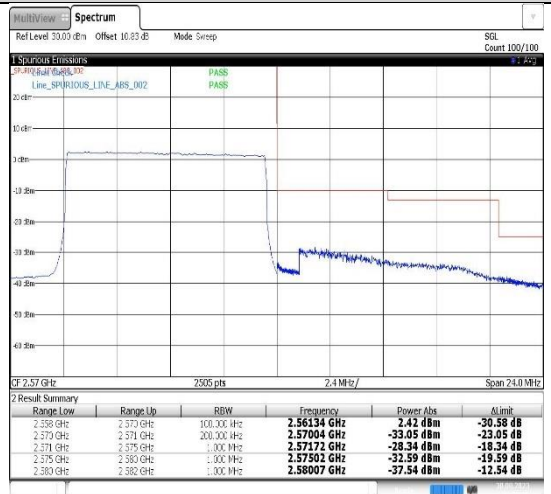
Band7-10MHz-QPSK-21400-50RB#0
