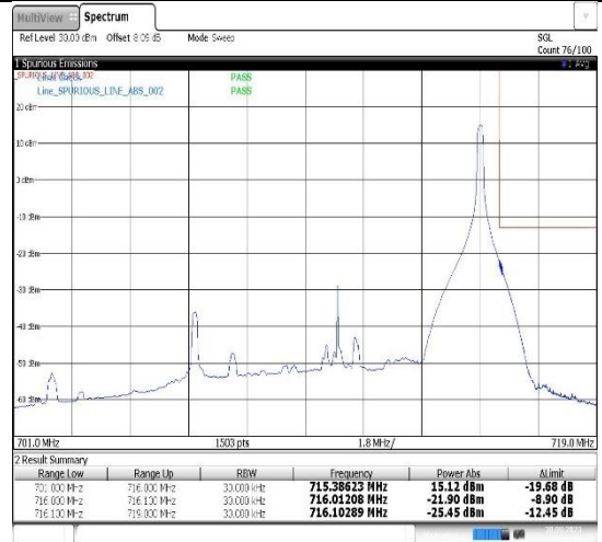
Band17-10MHz-QPSK-23800-1RB#49
