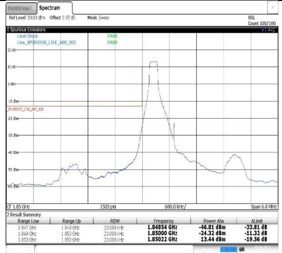
Band25-1.4MHz-QPSK-26047-1RB#0
