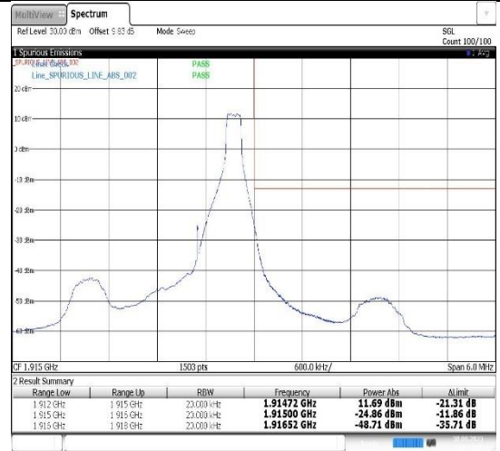
Band25-1.4MHz-16QAM-26683-1RB#5
