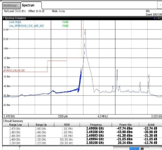
Band7-20MHz-16QAM-20850-1RB#0
