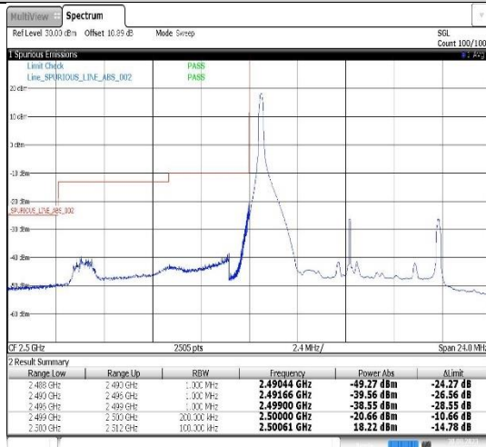
Band7-10MHz-16QAM-20800-1RB#0
