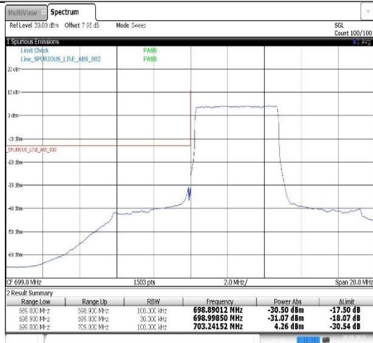
Band12-5MHz-QPSK-23035-25RB#0
