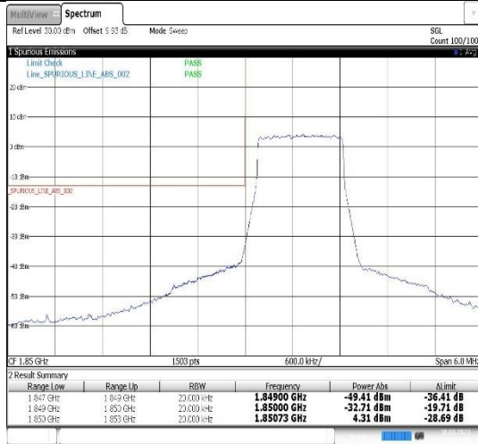
Band25-1.4MHz-16QAM-26047-6RB#0
