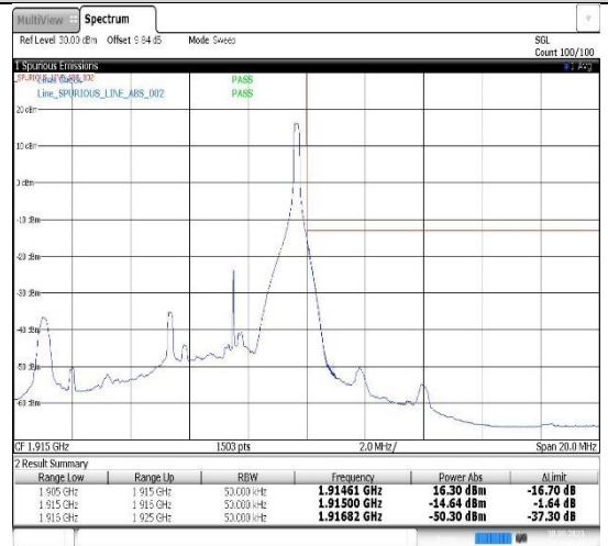
Band25-5MHz-QPSK-26665-1RB#24
