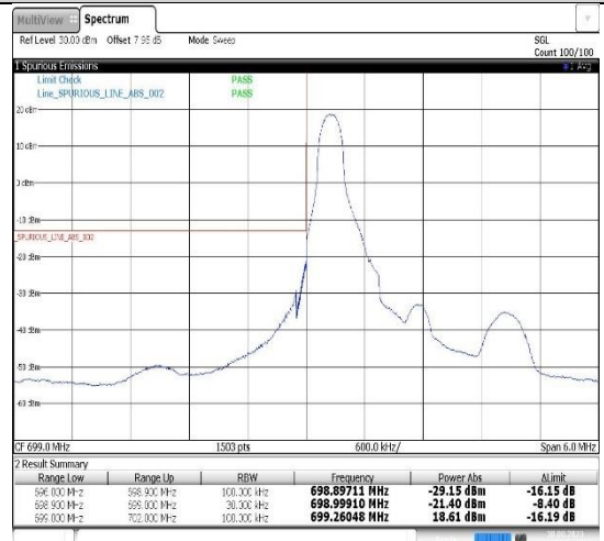
Band12-1.4MHz-QPSK-23017-1RB#0
