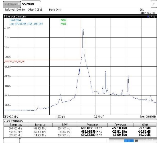
Band12-10MHz-16QAM-23060-1RB#0
