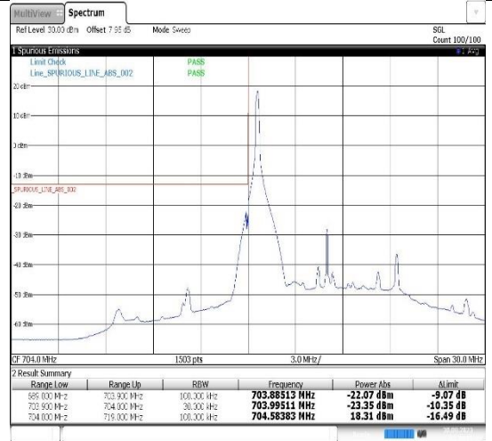
Band17-10MHz-16QAM-23800-1RB#49
