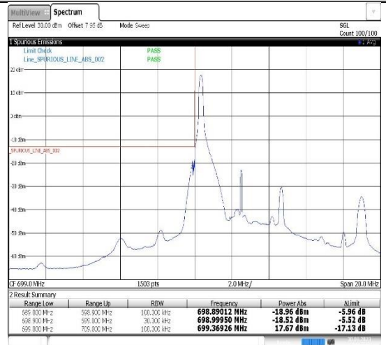
Band12-5MHz-16QAM-23035-1RB#0
