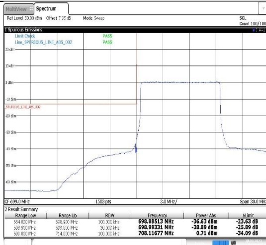
Band12-10MHz-16QAM-23060-50RB#0
