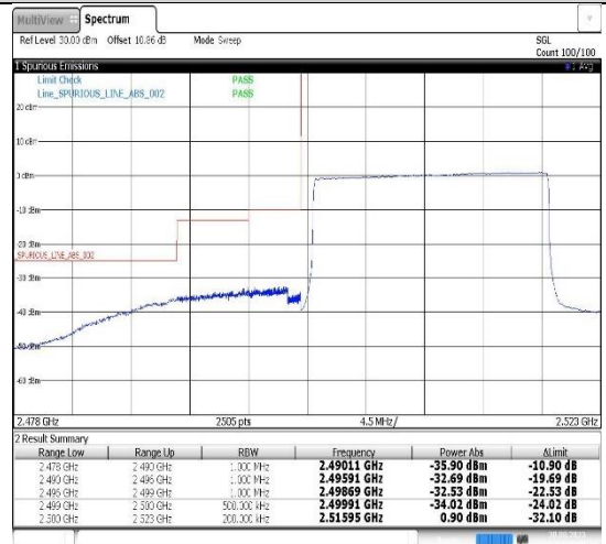
Band7-20MHz-16QAM-20850-100RB#0
