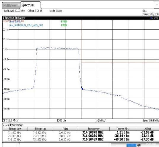
Band12-3MHz-16QAM-23165-15RB#0
