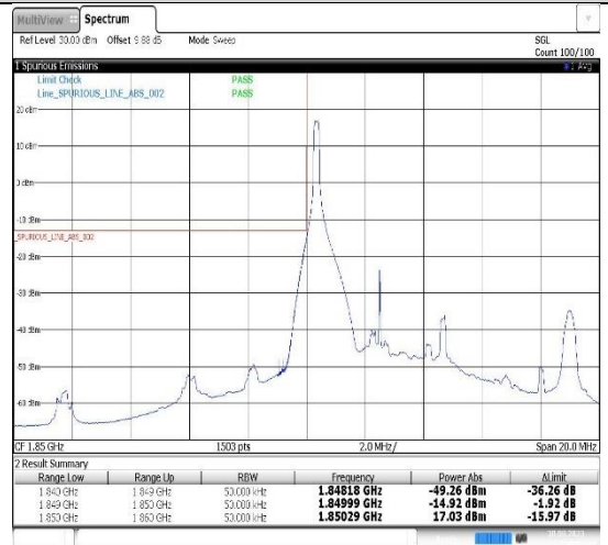
Band25-5MHz-QPSK-26065-1RB#0
