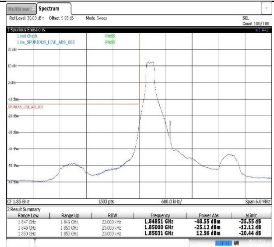
Band25-1.4MHz-16QAM-26047-1RB#0
