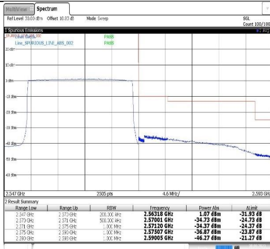
Band7-20MHz-16QAM-21350-100RB#0
