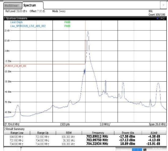
Band17-5MHz-QPSK-23755-1RB#0
