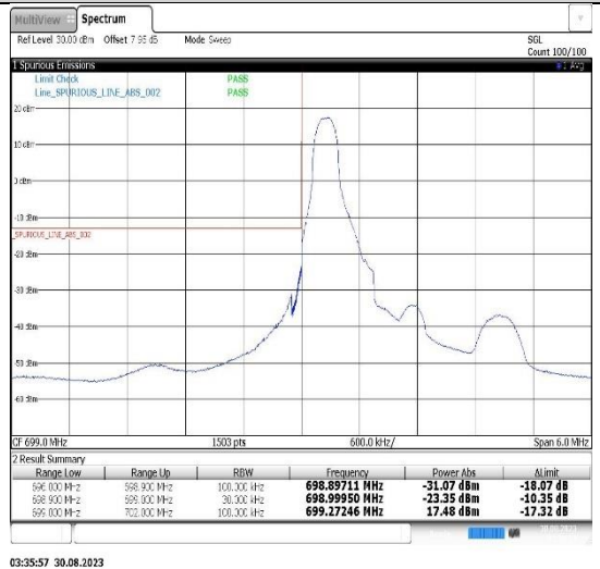
Band12-1.4MHz-16QAM-23017-1RB#5
