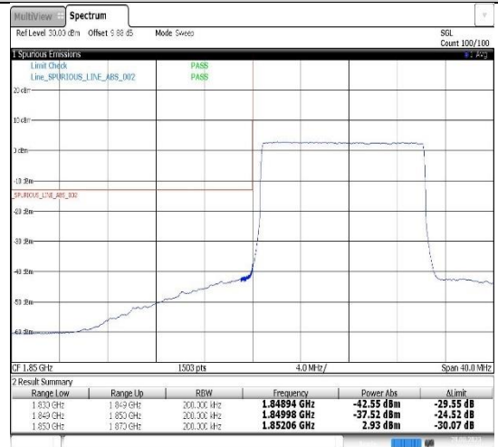
Band2-15MHz-16QAM-18675-75RB#0
