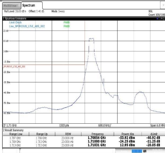
Band4-1.4MHz-16QAM-19957-1RB#0
