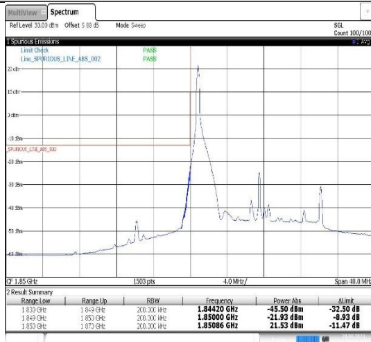
Band2-15MHz-16QAM-18675-1RB#0
