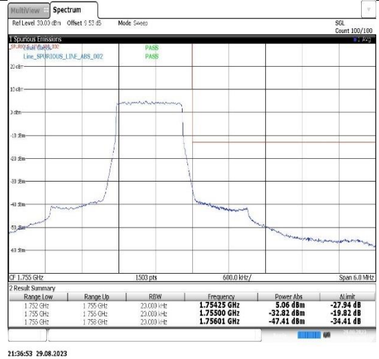
Band4-1.4MHz-16QAM-19957-6RB#0
