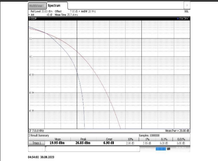
Band17-10MHz-16QAM-23790-50RB#0
