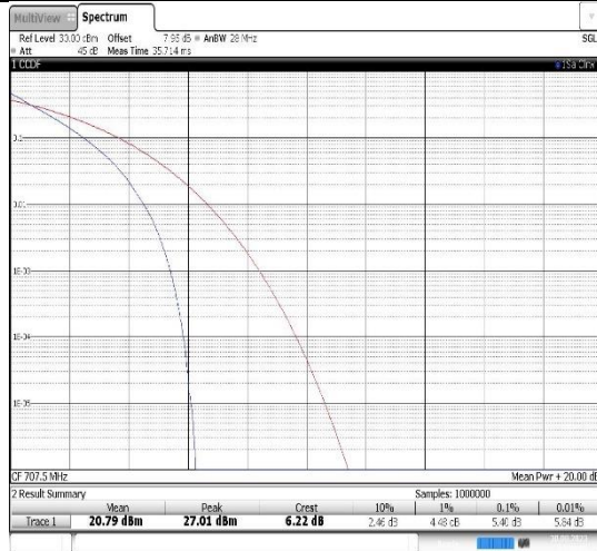
Band12-10MHz-QPSK-23095-50RB#0
