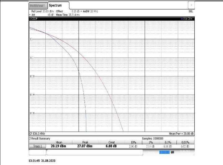
Band26(824-849)-10MHz-16QAM-26915-50RB#0
