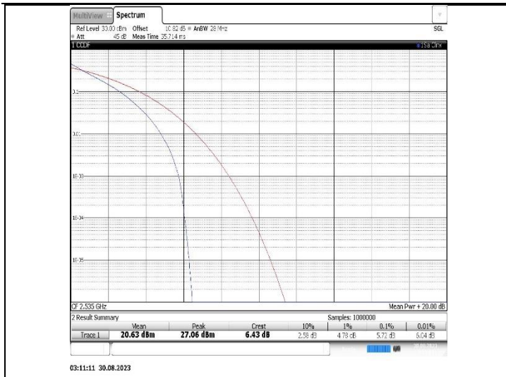
Band7-20MHz-QPSK-21100-100RB#0
