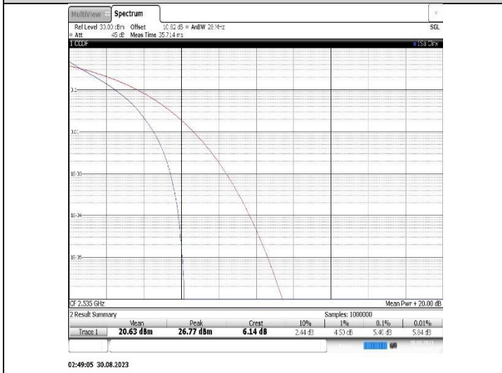
Band7-15MHz-QPSK-21100-75RB#0
