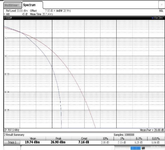
Band12-5MHz-16QAM-23095-25RB#0
