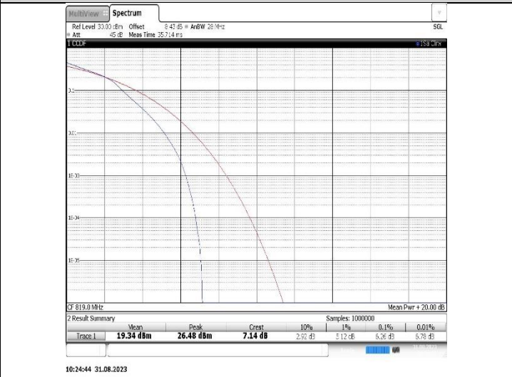
Band26(814-824)-10MHz-16QAM-26740-50RB#0
