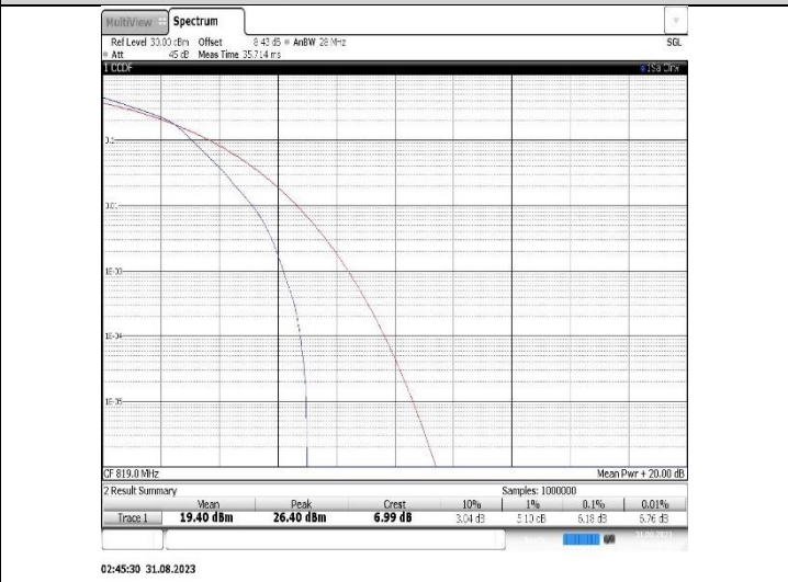
Band26(814-824)-3MHz-16QAM-26740-15RB#0
