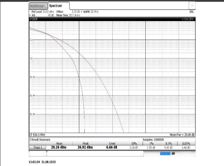
Band26(824-849)-3MHz-16QAM-26915-15RB#0
