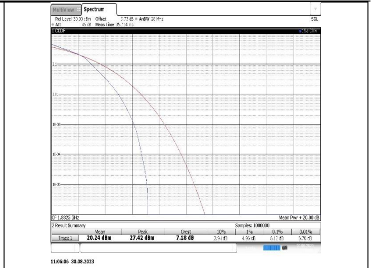
Band25-5MHz-16QAM-26365-25RB#0
