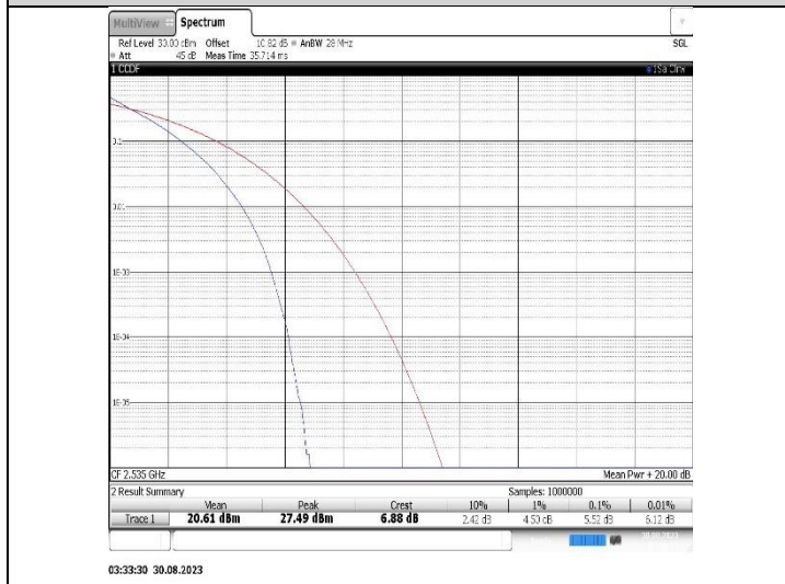
Band7-20MHz-QPSK-21100-100RB#0
