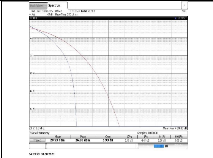
Band17-10MHz-QPSK-23790-50RB#0
