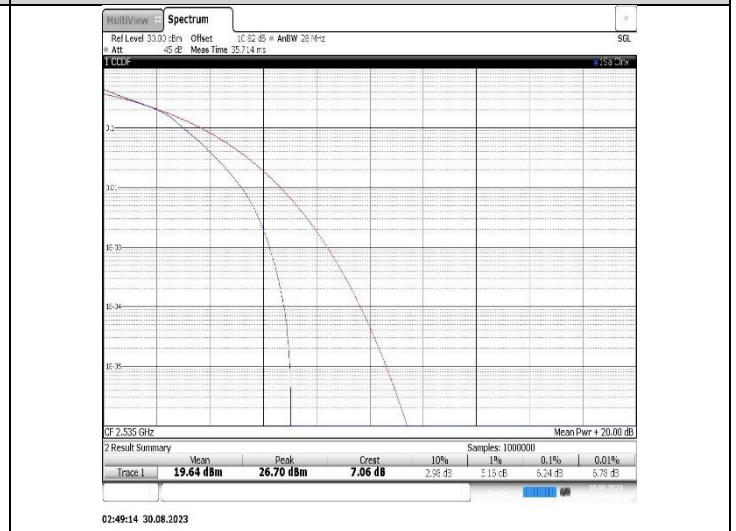
Band7-15MHz-16QAM-21100-75RB#0
