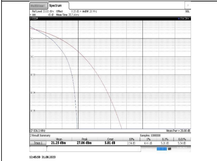
Band26(824-849)-5MHz-QPSK-26915-25RB#0
