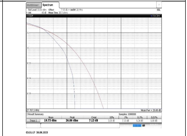
Band12-1.4MHz-16QAM-23095-6RB#0
