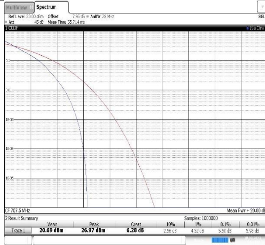
Band12-5MHz-QPSK-23095-25RB#0
