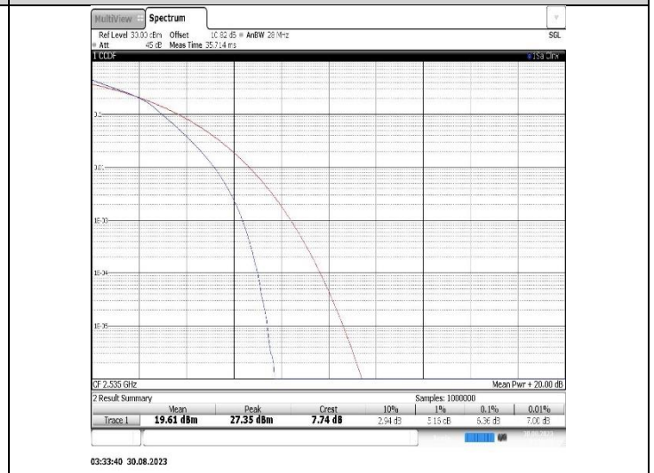
Band7-20MHz-16QAM-21100-100RB#0
