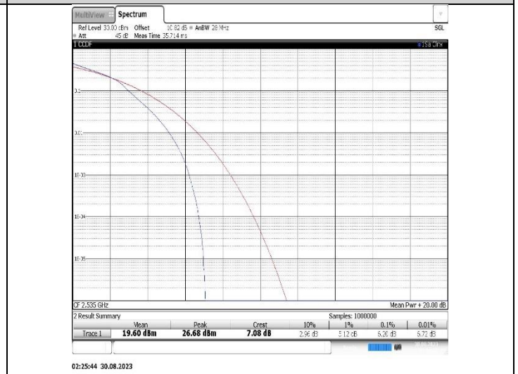
Band7-10MHz-16QAM-21100-50RB#0
