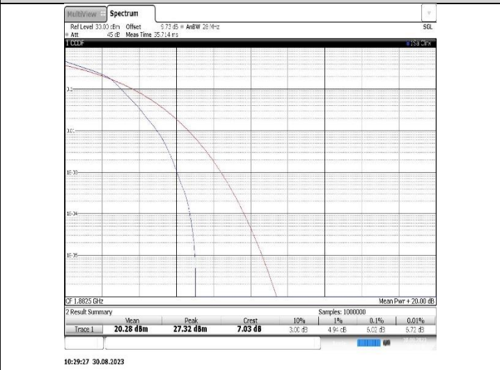
Band25-3MHz-16QAM-26365-15RB#0
