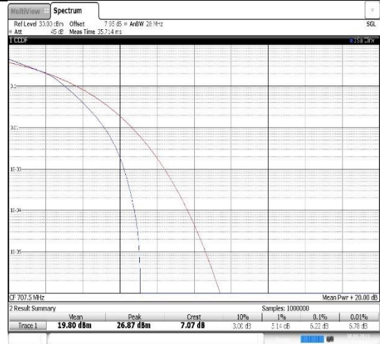
Band12-10MHz-16QAM-23095-50RB#0
