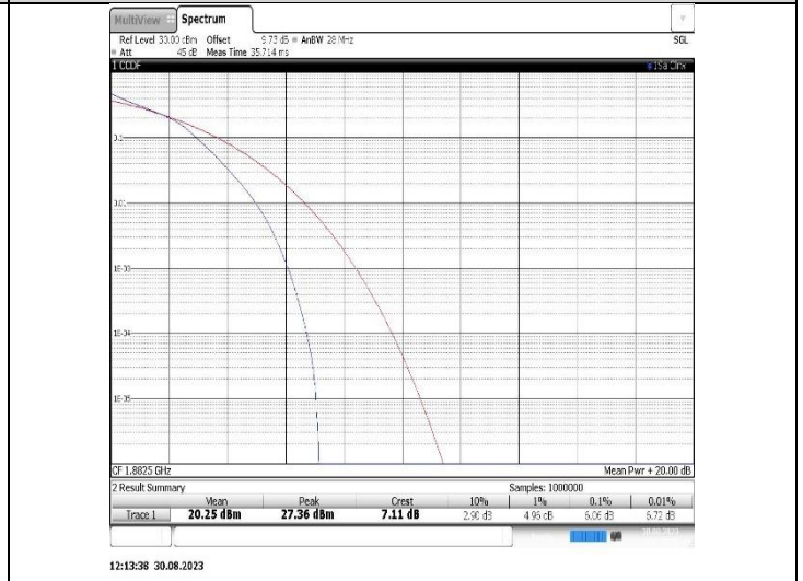
Band25-15MHz-16QAM-26365-75RB#0
