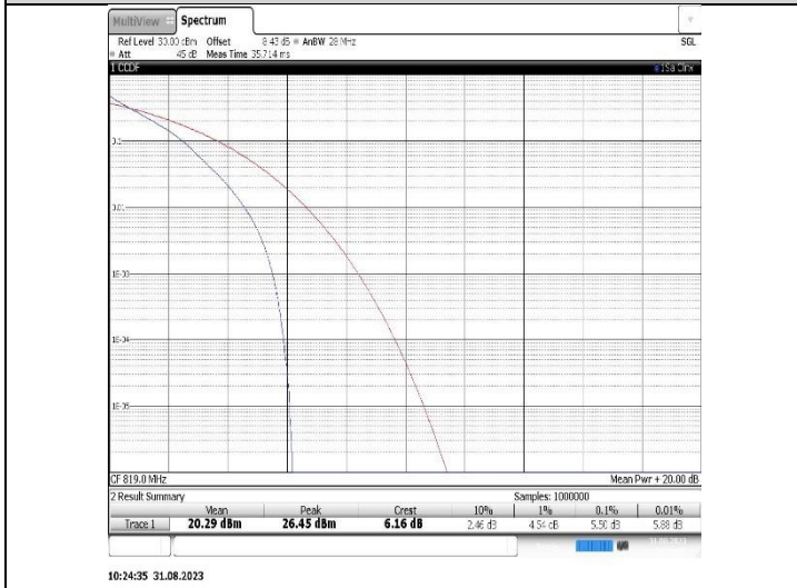
Band26(814-824)-10MHz-QPSK-26740-50RB#0
