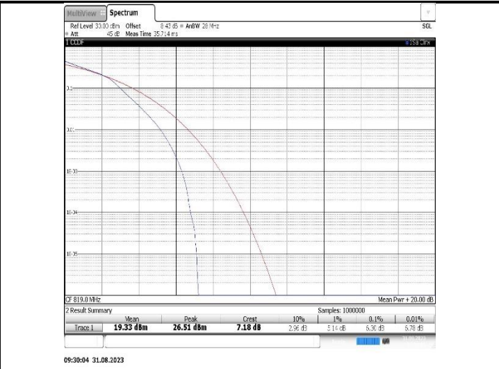
Band26(814-824)-5MHz-16QAM-26740-25RB#0
