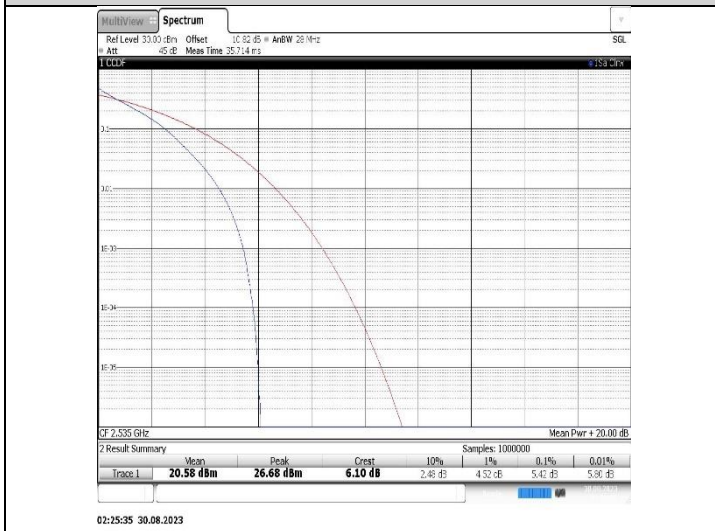
Band7-10MHz-QPSK-21100-50RB#0
