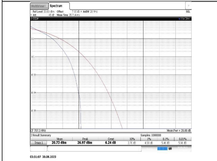
Band12-1.4MHz-QPSK-23095-6RB#0
