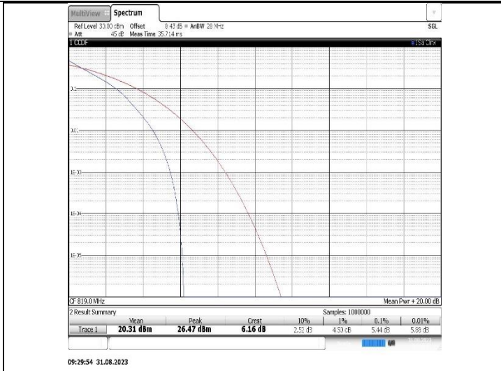
Band26(814-824)-5MHz-QPSK-26740-25RB#0
