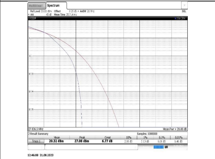
Band26(824-849)-5MHz-16QAM-26915-25RB#0
