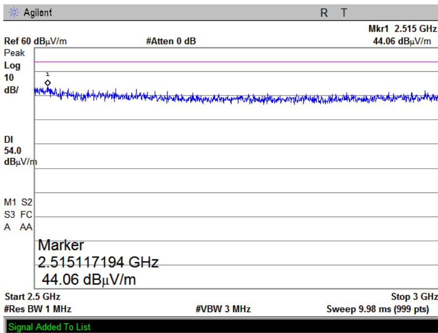
Plot 3.5.16 Emissions in restricted frequency bands test results, 2.5 – 3.0 GHz range, Horizontal, Fc = 2440 MHz (w/o notch filter)
