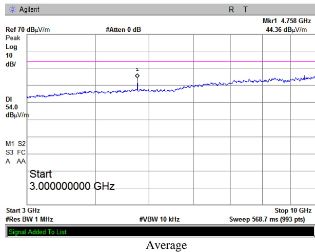
Plot 3.5.8 Emissions in restricted frequency bands test results, 3 – 10 GHz range, Horizontal, Fc = 2405 MHz (with notch filter)
