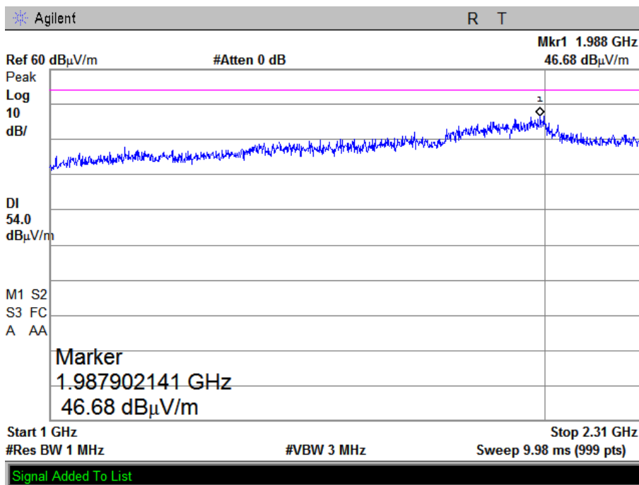
Plot 3.5.14 Emissions in restricted frequency bands test results, 1.0 – 2.31 GHz range, Horizontal, Fc = 2440 MHz (w/o notch filter)
