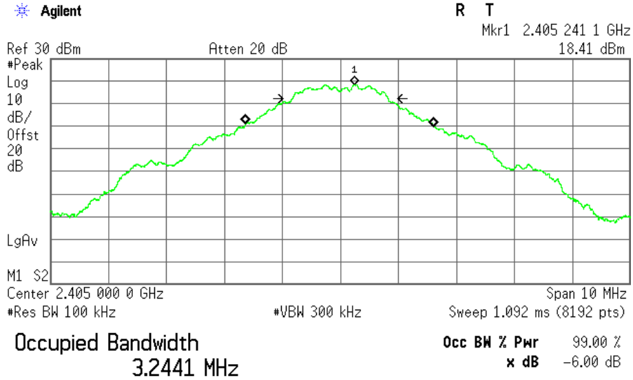
Plot 3.1.1: 6 dB DTS Bandwidth, Fc = 2405MHz
