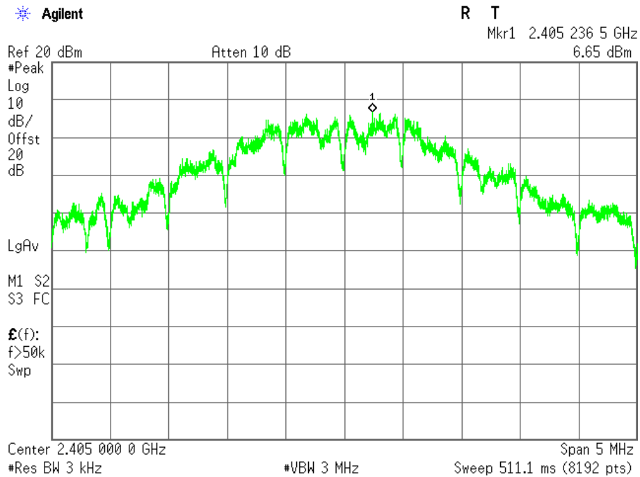
Plot 3.3.1 Maximum Power Spectral Density test results, Fc = 2405MHz
