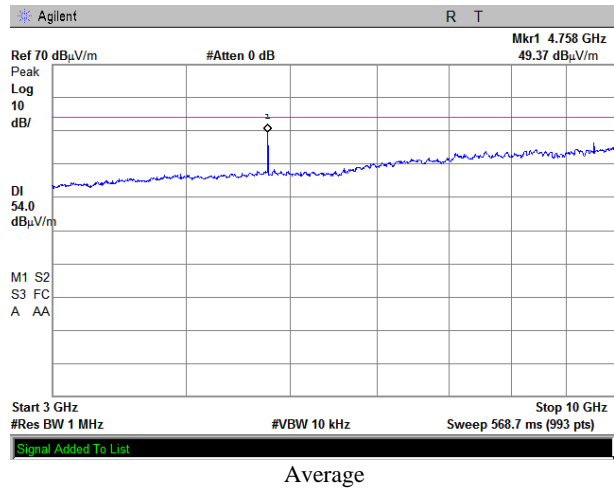
Plot 3.5.8 Emissions in restricted frequency bands test results, 3 – 10 GHz range, Horizontal, Fc = 2405 MHz (with notch filter)
