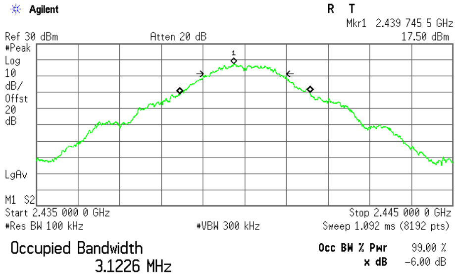
Plot 3.1.2: 6 dB DTS Bandwidth, Fc = 2440MHz
