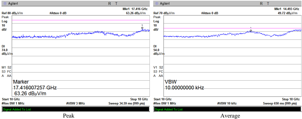
Plot 3.5.10 Emissions in restricted frequency bands test results, 10 – 18 GHz range, Horizontal, Fc = 2405 MHz (with notch filter)
