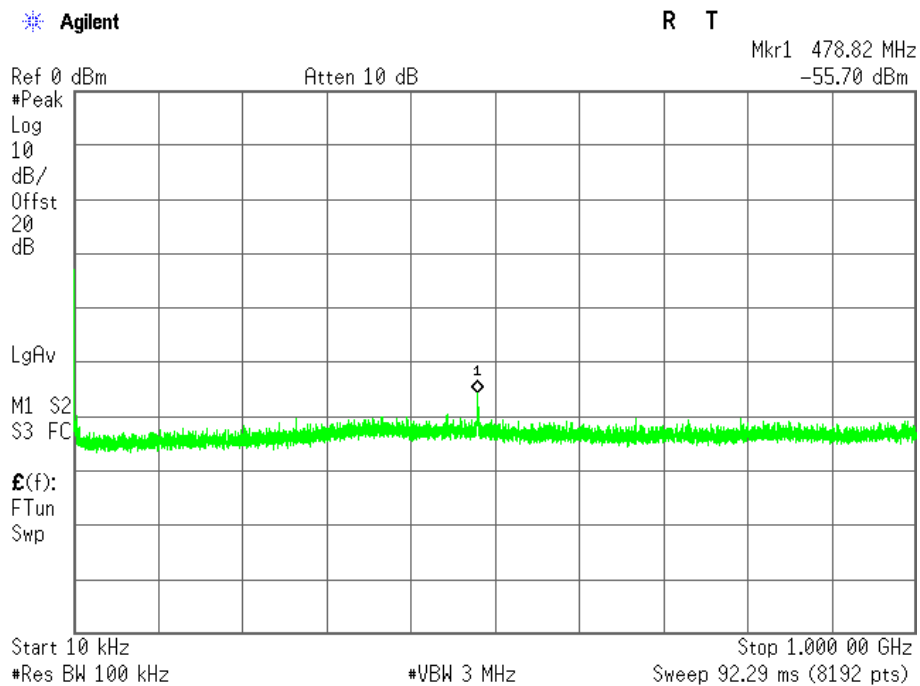
Plot 3.4.5 Unwanted Conducted Emissions into Non-Restricted Frequency Bands test results in 9 kHz – 1 GHz frequency range, F_c = 2440 MHz
