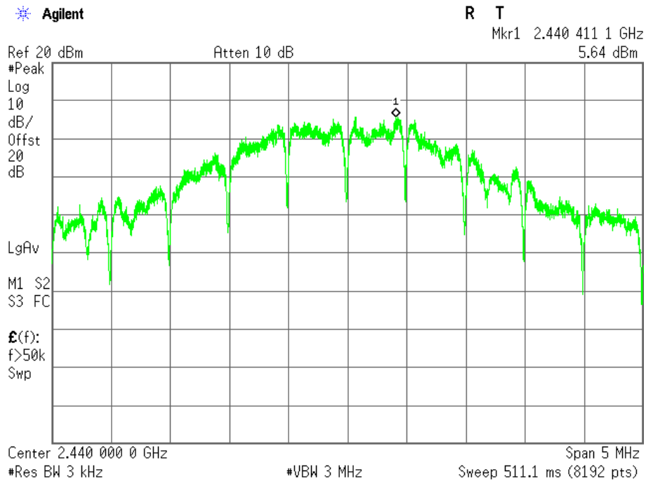
Plot 3.3.2 Maximum Power Spectral Density test results, Fc = 2440MHz
