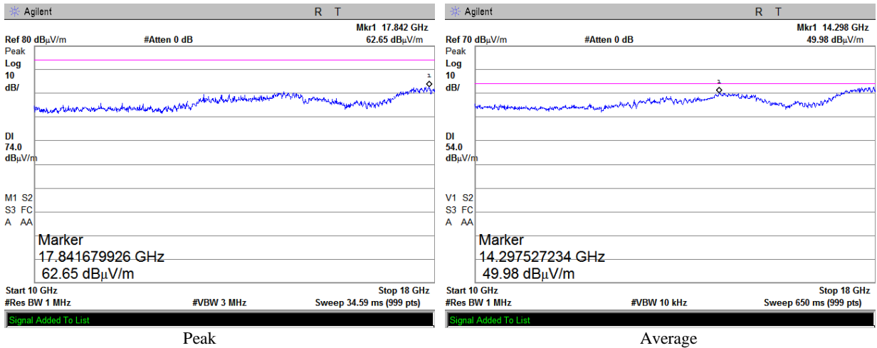
Plot 3.5.10 Emissions in restricted frequency bands test results, 10 – 18 GHz range, Horizontal, Fc = 2405 MHz (with notch filter)
