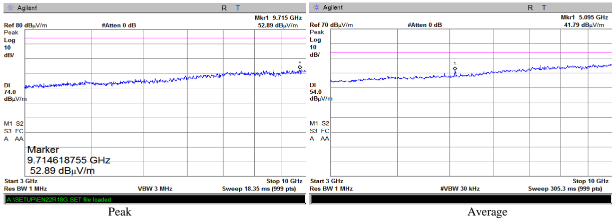
Plot 3.5.28 Emissions in restricted frequency bands test results, 3 – 10 GHz range, Horizontal, Fc = 2480 MHz (with notch filter)
