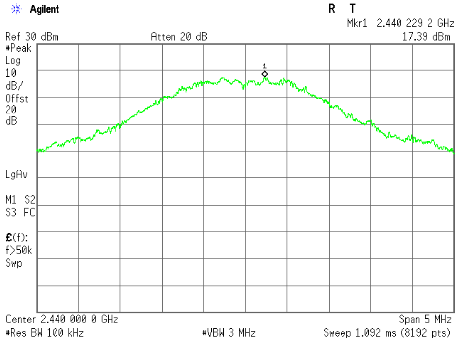
Plot 3.4.4 Unwanted Conducted Emissions into Non-Restricted Frequency Bands test results, Fundamental Emission Reference Level, F_c = 2440 MHz
