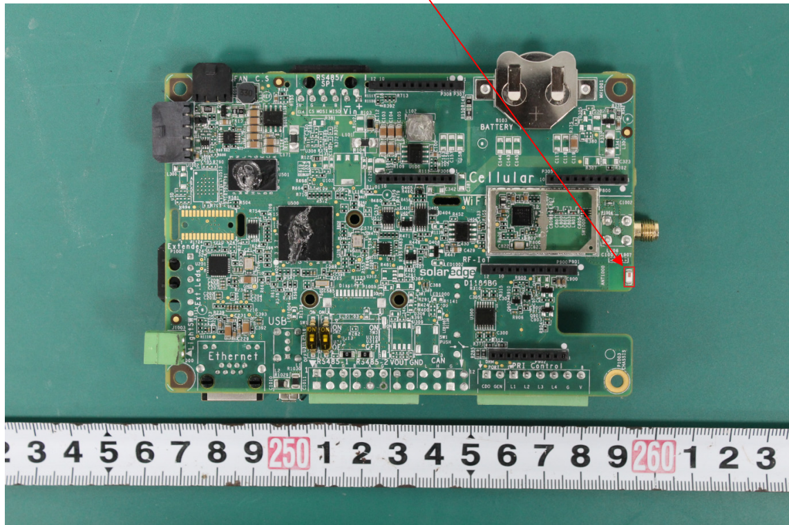
Chip Antenna
