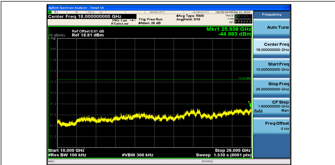
RF Conducted Spurious Emissions_BLE_2442
