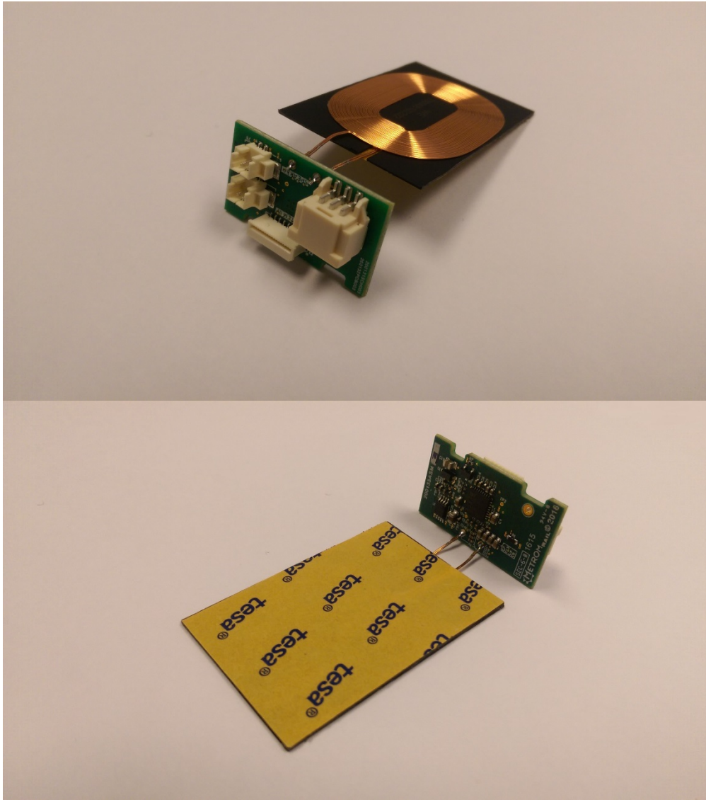
Personnel module charging coil and assembly
