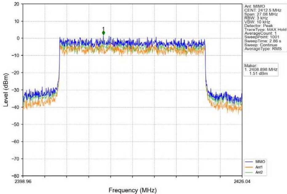
16QAM 20MHz_LCH_2412.5MHz_MIMO_NTNV
