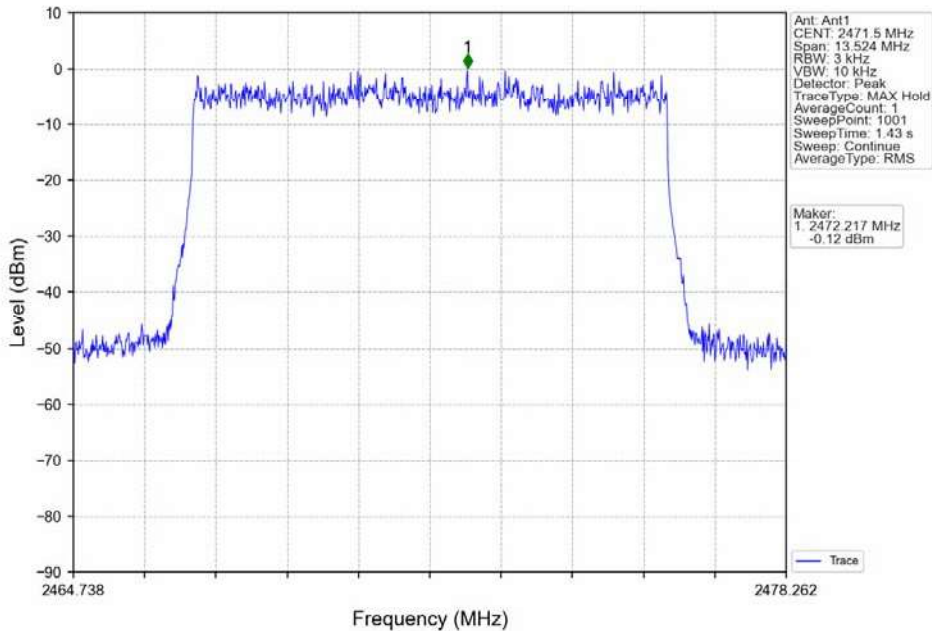
16QAM 10MHz_HCH_2471.5MHz_Ant1_NTNV
