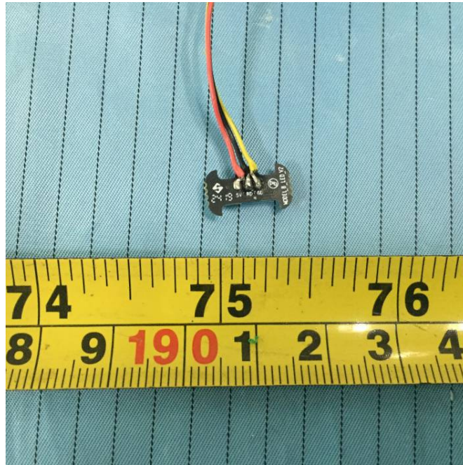
EUT – LED Board 2 Bottom View
