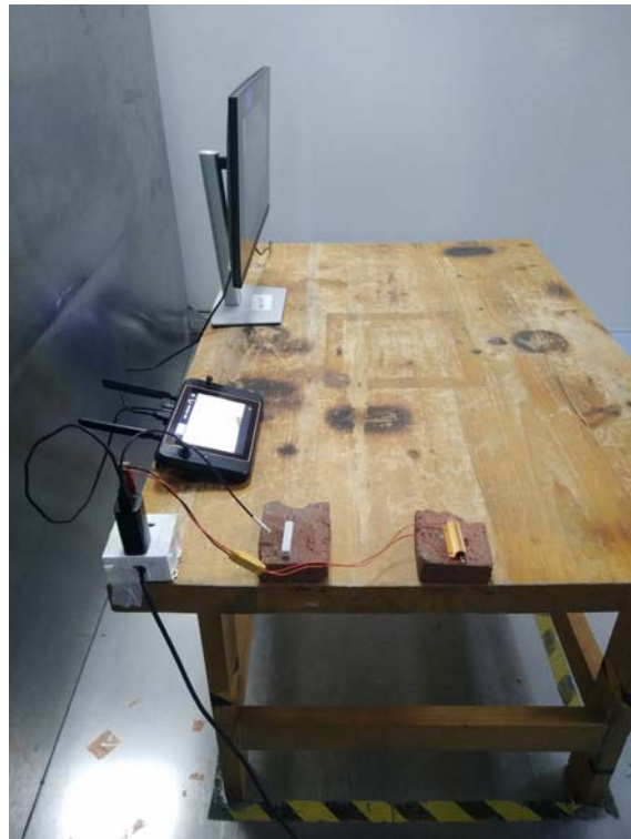
Conducted Emission Rear View
