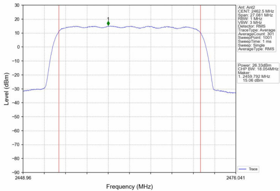
16QAM_HCH_2462.5MHz_Ant2_NTNV
