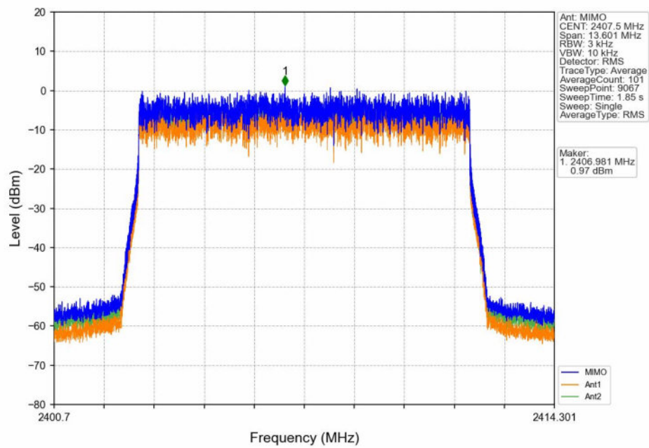
16QAM_LCH_2407.5MHz_MIMO_NTNV
