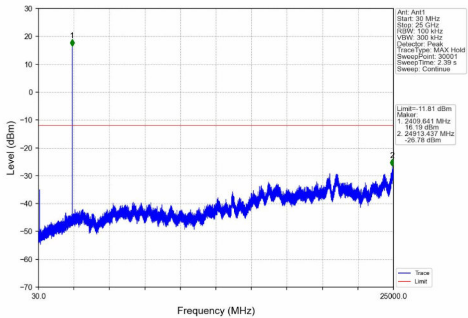
16QAM_LCH_2407.5MHz_Ant1_NTNV
