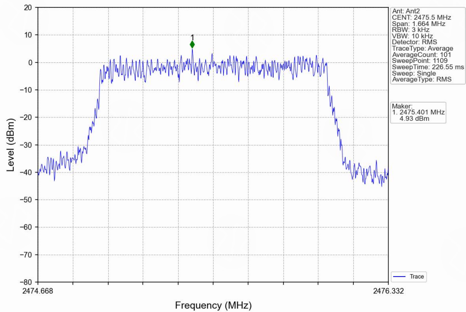
16QAM_HCH_2475.5MHz_MIMO_NTNV
