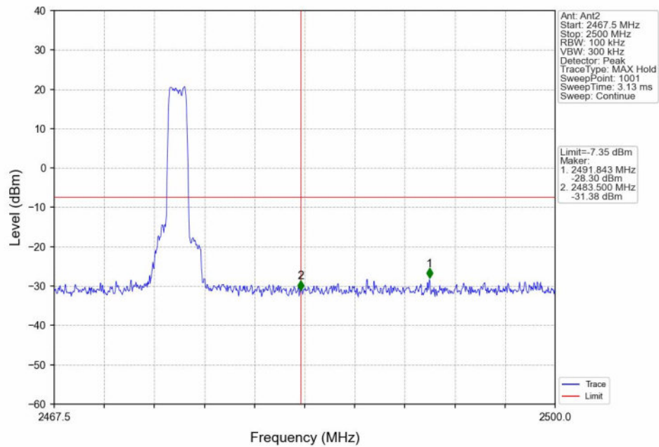
QPSK_HCH_2475.5MHz_Ant2_NTNV
