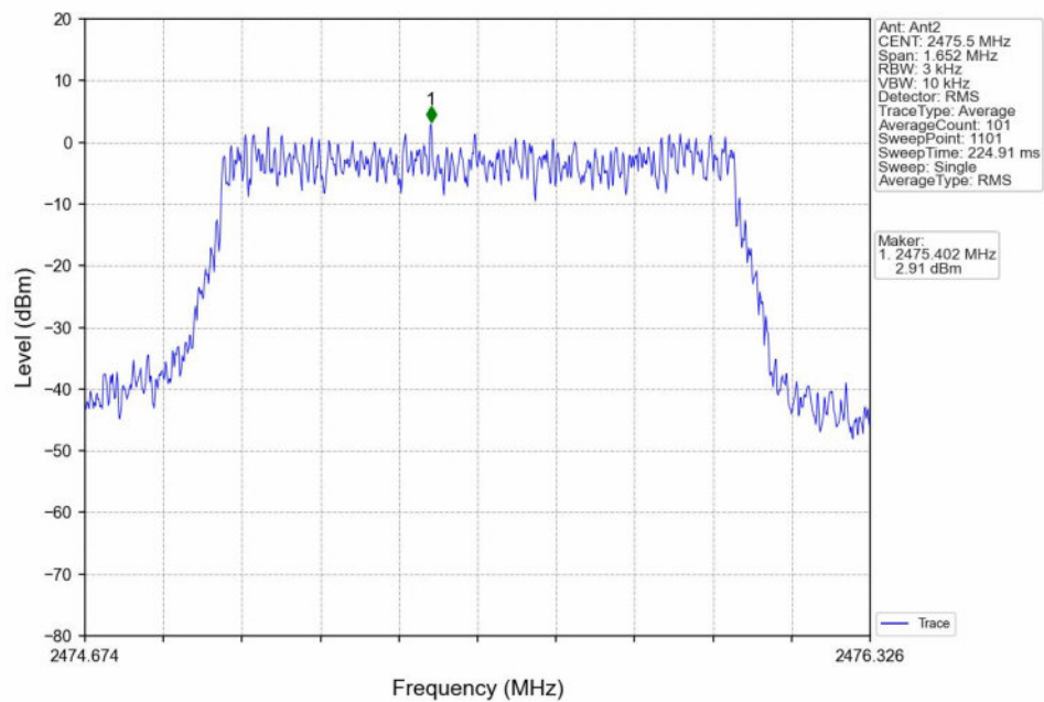
QPSK_HCH_2475.5MHz_Ant2_NTNV
