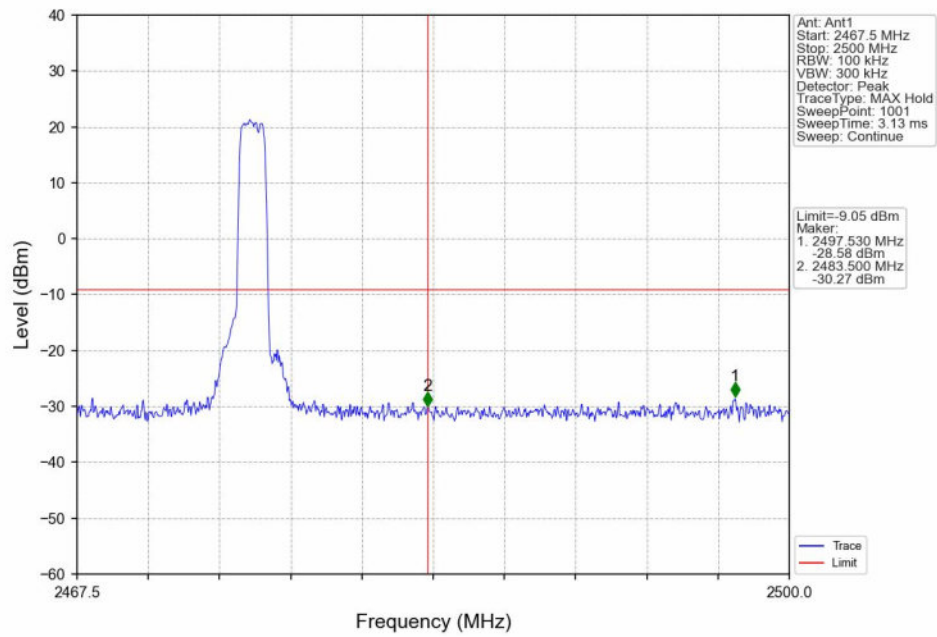
QPSK_HCH_2475.5MHz_Ant1_NTNV
