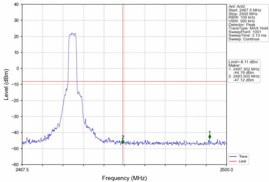
16QAM_HCH_2475.5MHz_Ant2_NTNV
