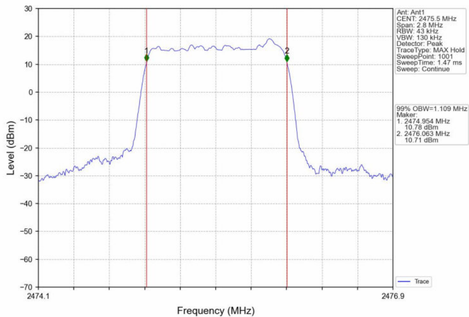
16QAM_HCH_2475.5MHz_MIMO_NTNV
