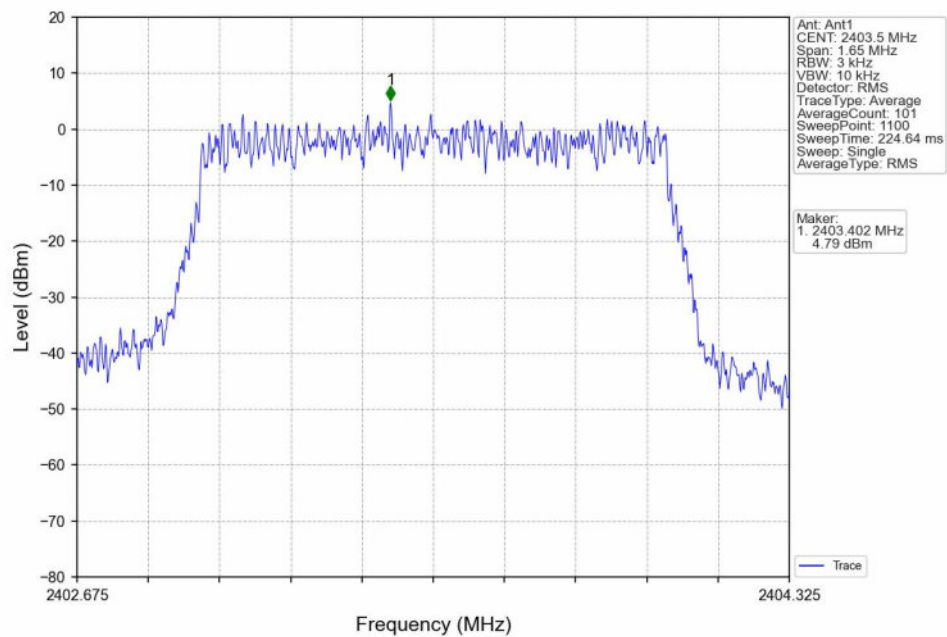
16QAM_LCH_2403.5MHz_Ant1_NTNV
