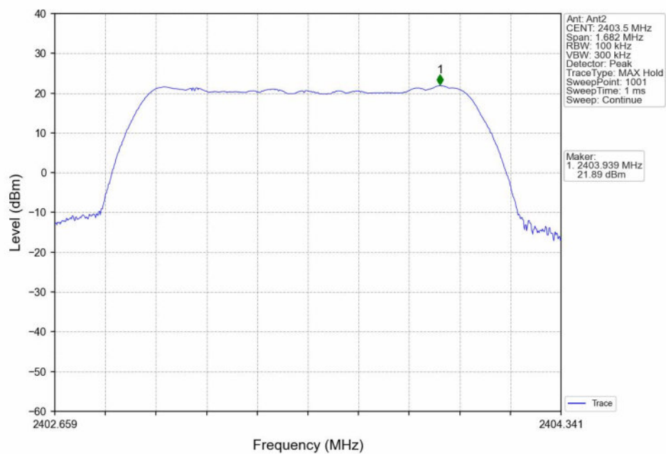
16QAM_LCH_2403.5MHz_Ant2_NTNV
