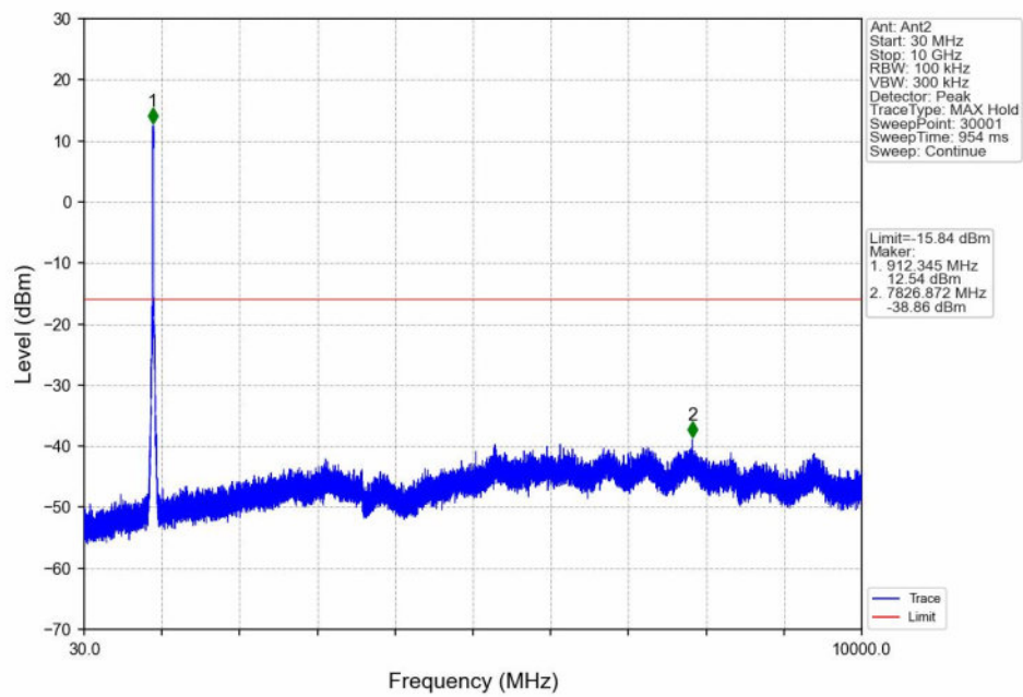
16QAM_LCH_914MHz_Ant2_NTNV
