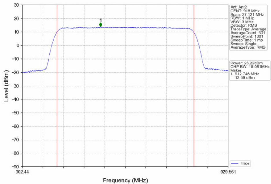
QPSK_HCH_916MHz_Ant2_NTNV
