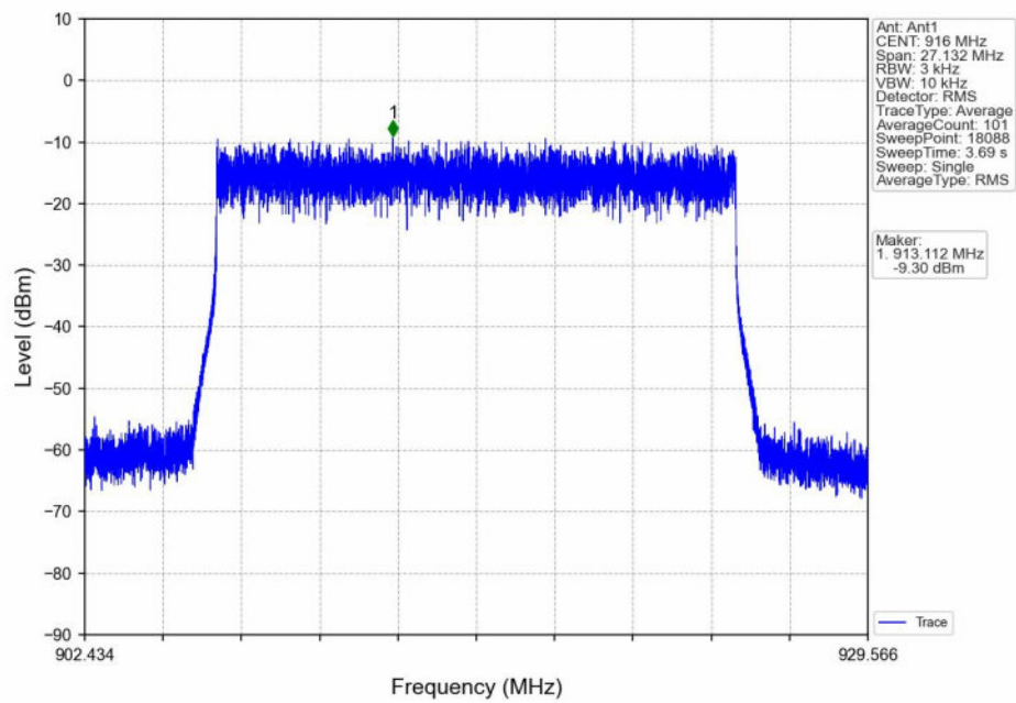
16QAM_HCH_916MHz_Ant1_NTNV
