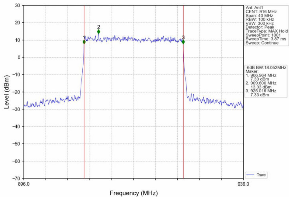
16QAM_HCH_916MHz_Ant1_NTNV
