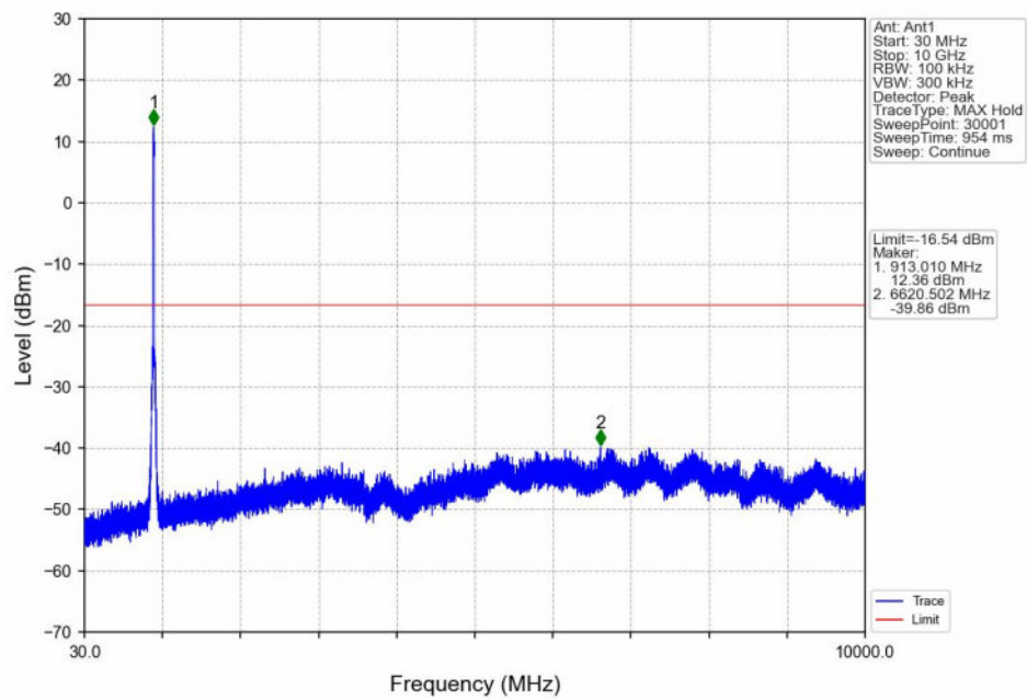
16QAM_LCH_914MHz_Ant1_NTNV
