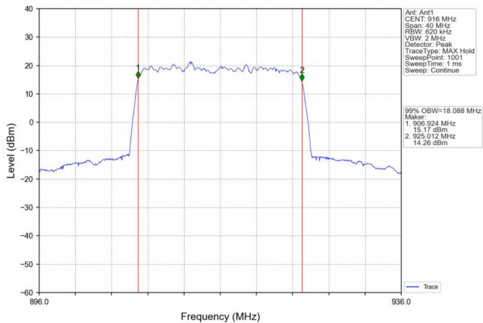
16QAM_HCH_916MHz_Ant1_NTNV
