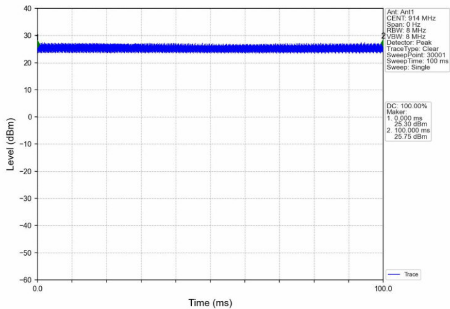
16QAM_LCH_914MHz_Ant1_NTNV
