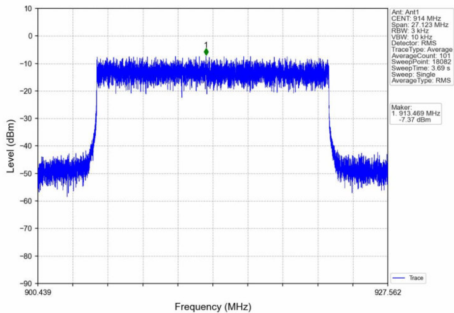
16QAM_LCH_914MHz_Ant1_NTNV
