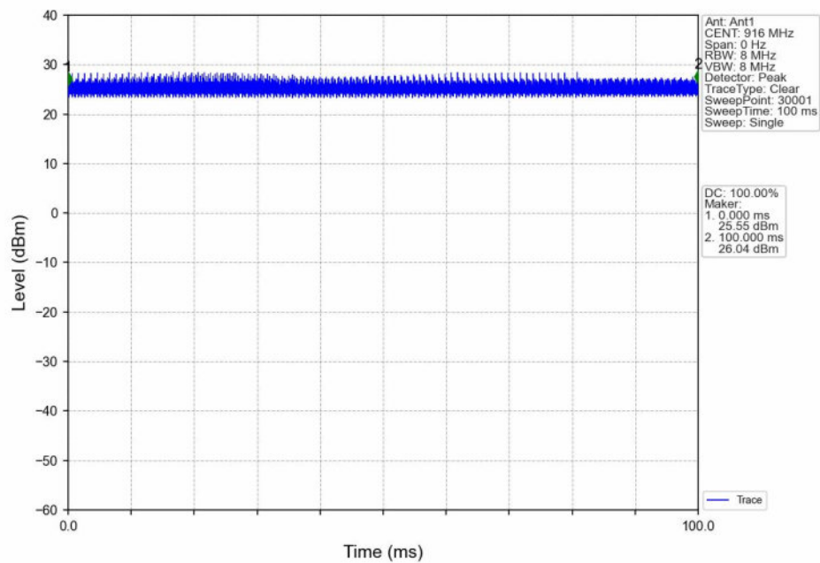
16QAM_HCH_916MHz_Ant1_NTNV
