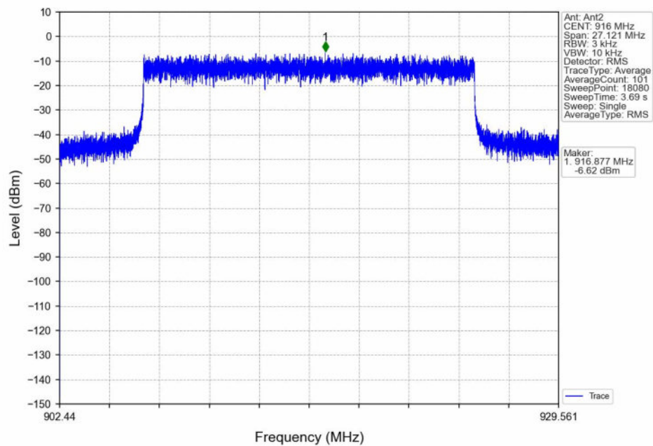
QPSK_HCH_916MHz_Ant2_NTNV
