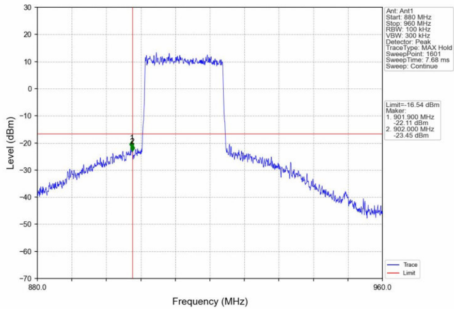
16QAM_LCH_914MHz_Ant1_NTNV
