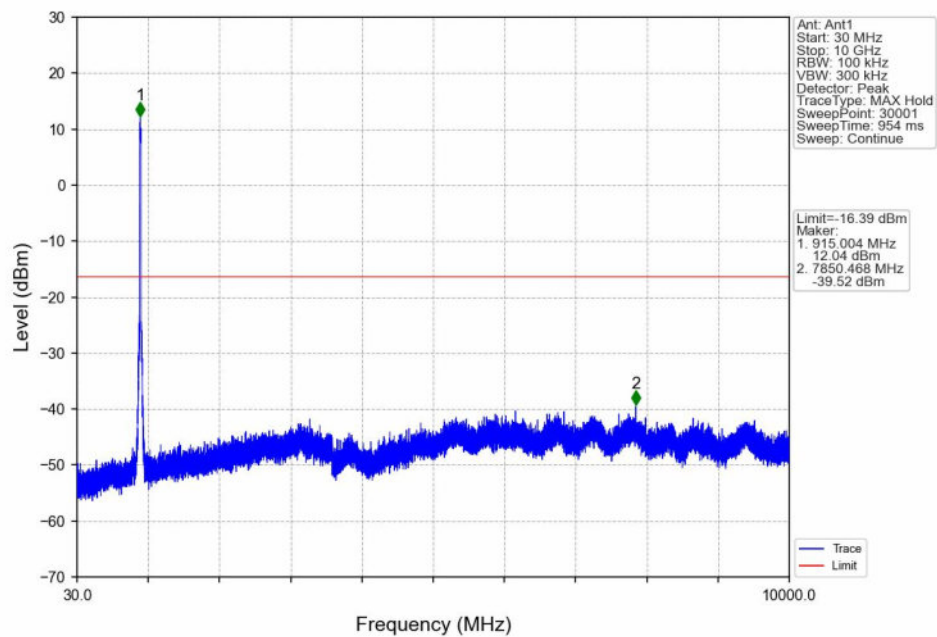
QPSK_HCH_916MHz_Ant1_NTNV
