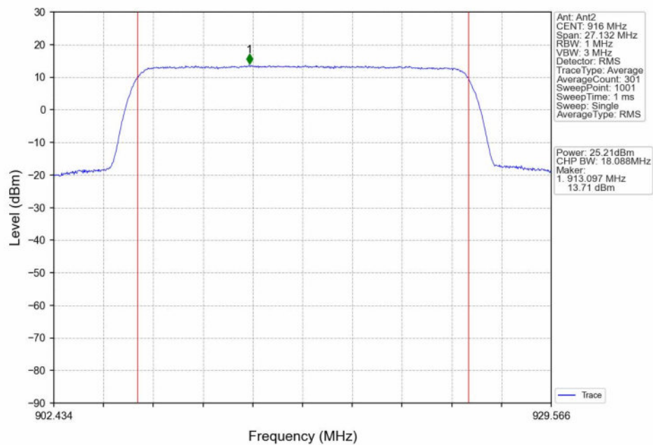
16QAM_HCH_916MHz_Ant2_NTNV
