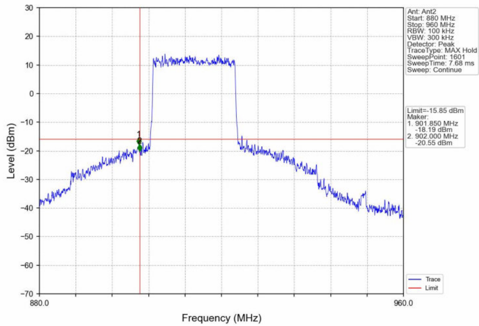
QPSK_LCH_914MHz_Ant2_NTNV
