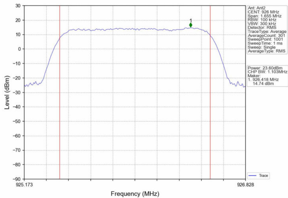
QPSK_HCH_926MHz_Ant2_NTNV
