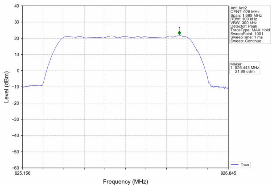
QPSK_HCH_926MHz_Ant2_NTNV
