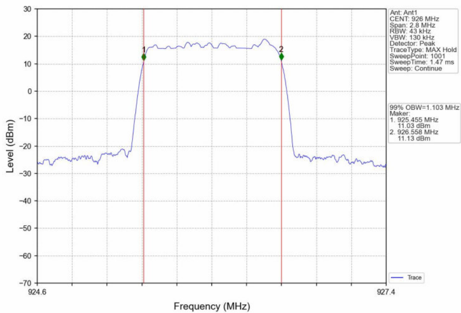
16QAM_HCH_926MHz_Ant1_NTNV
