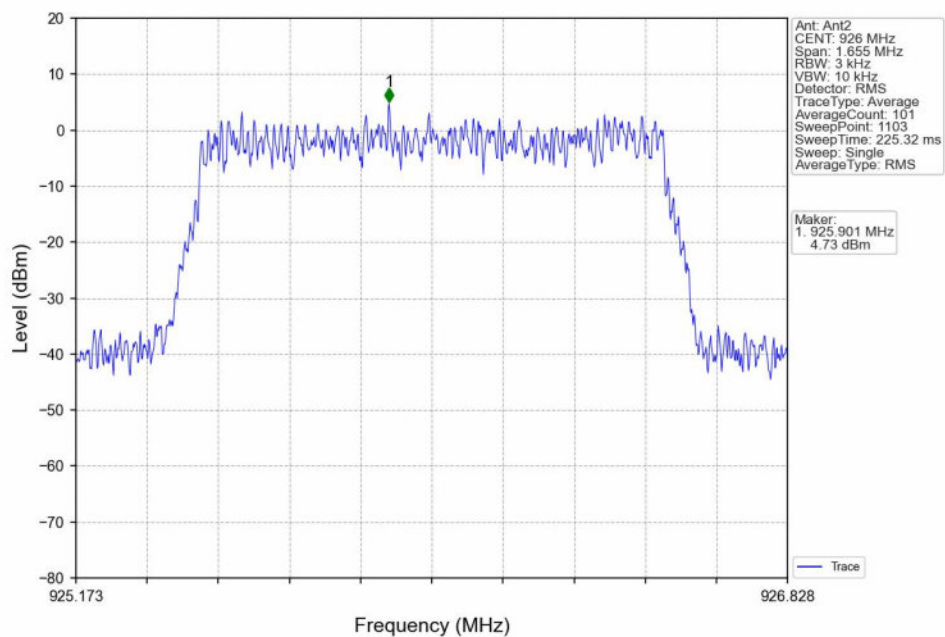
QPSK_HCH_926MHz_Ant2_NTNV
