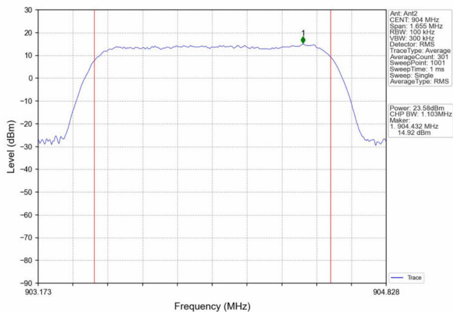
16QAM_LCH_904MHz_Ant2_NTNV
