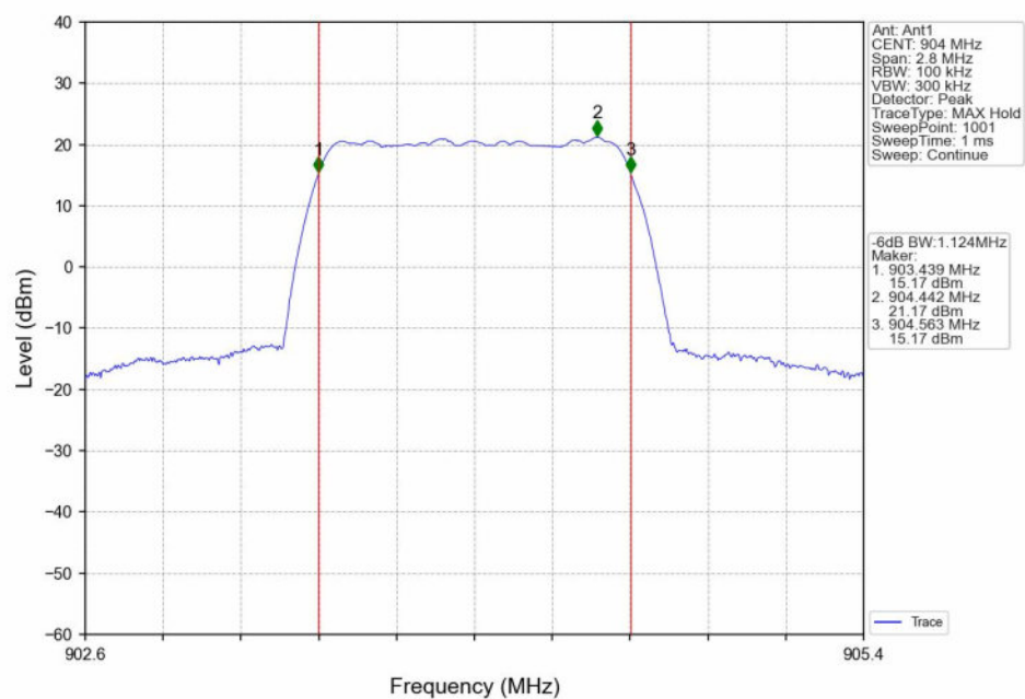
16QAM_LCH_904MHz_Ant1_NTNV
