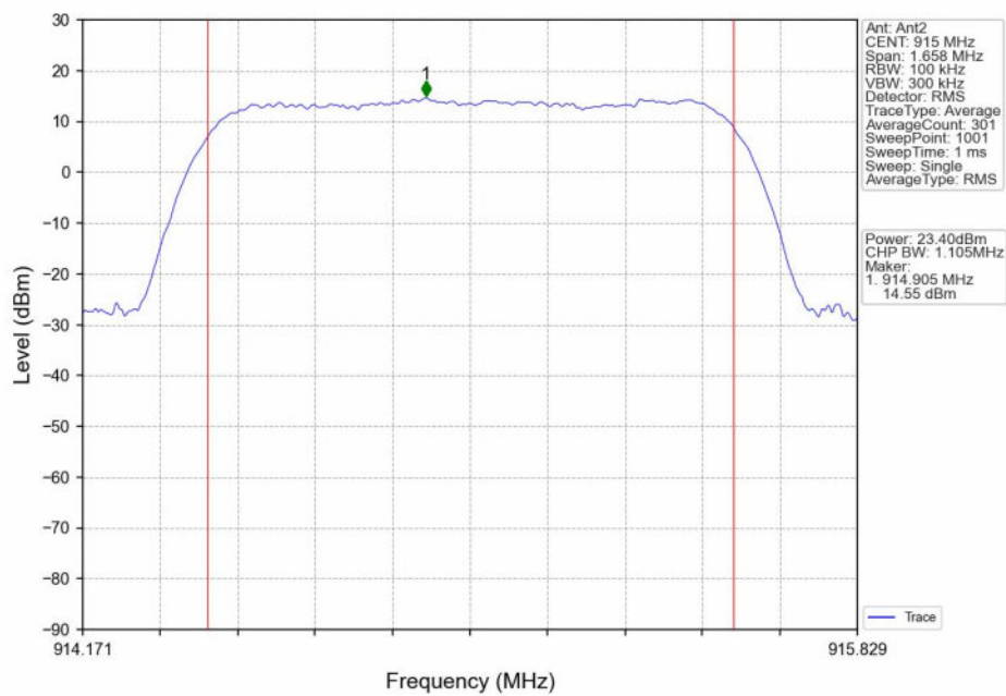
QPSK_MCH_915MHz_Ant2_NTNV
