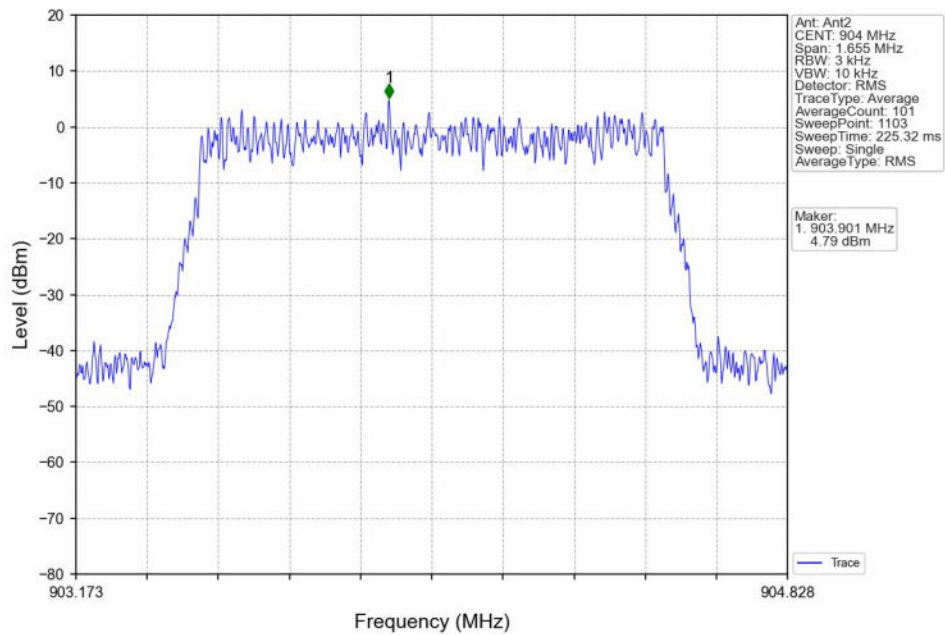
16QAM_LCH_904MHz_MIMO_NTNV
