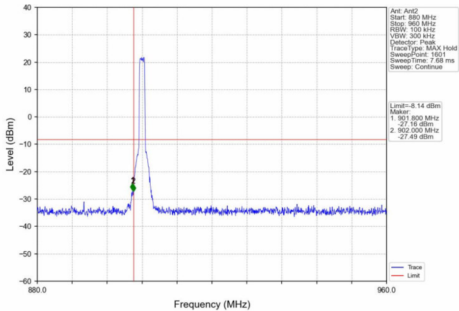
16QAM_LCH_904MHz_Ant2_NTNV
