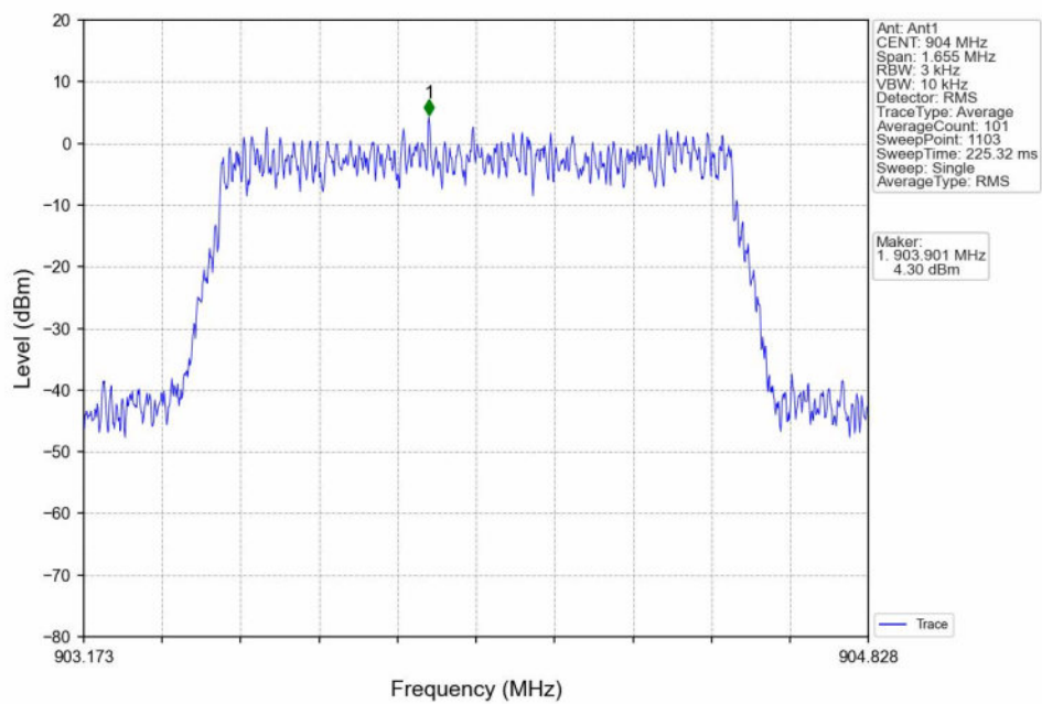
16QAM_LCH_904MHz_Ant1_NTNV
