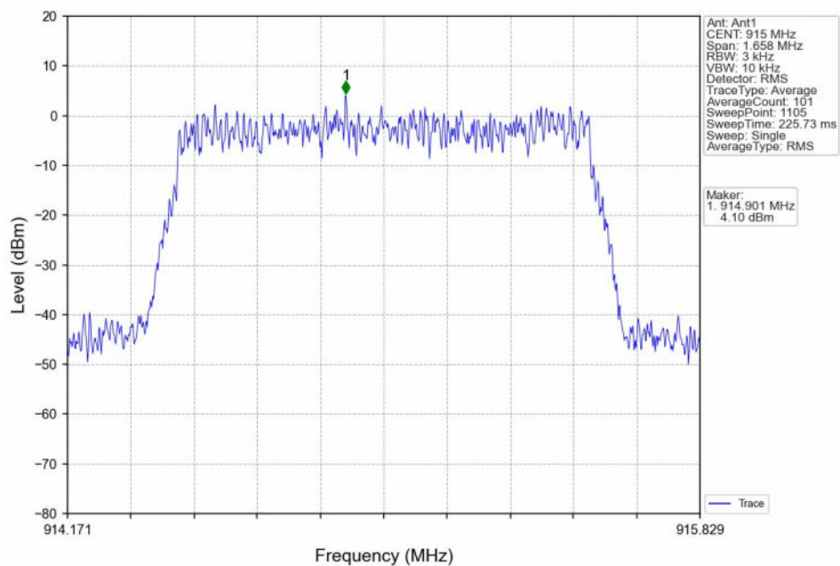
QPSK_MCH_915MHz_Ant1_NTNV
