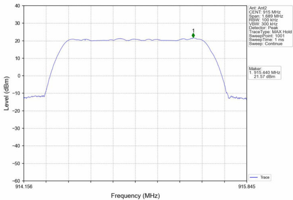
QPSK_MCH_915MHz_Ant2_NTNV
