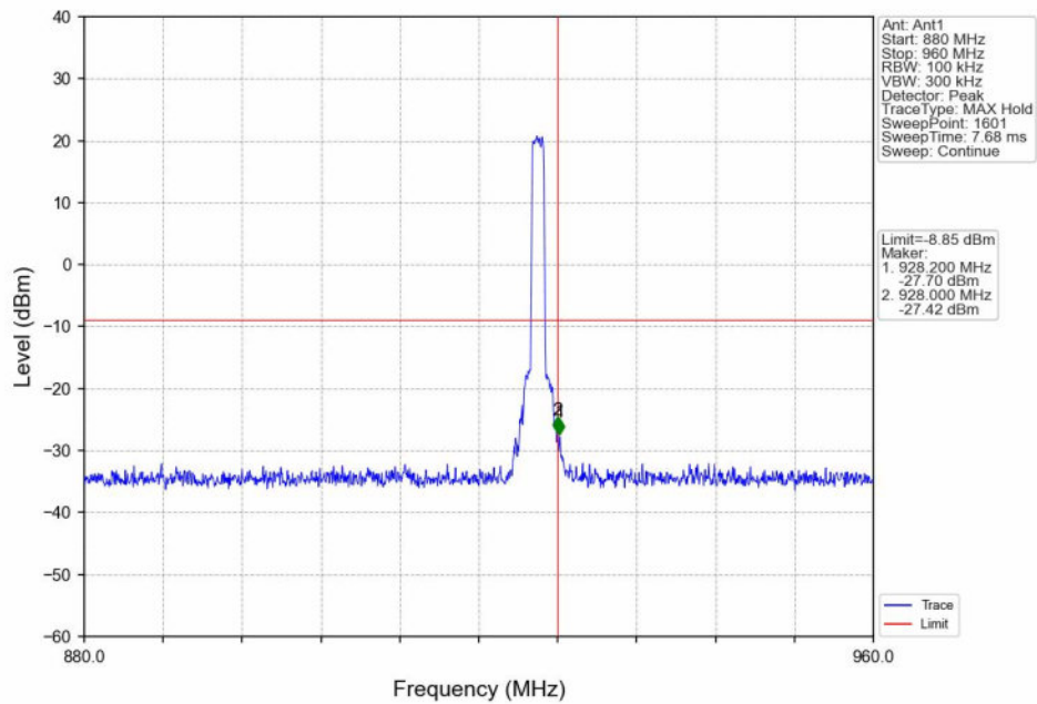
16QAM_HCH_926MHz_Ant1_NTNV
