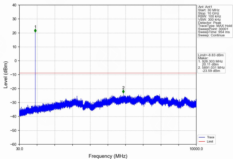
QPSK_HCH_926MHz_Ant1_NTNV
