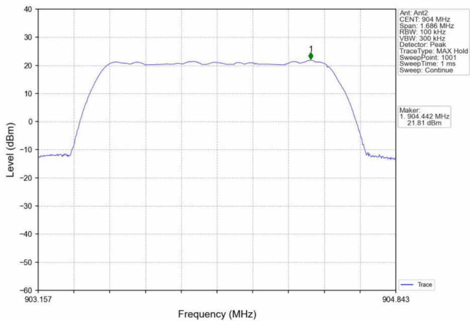
16QAM_LCH_904MHz_Ant2_NTNV
