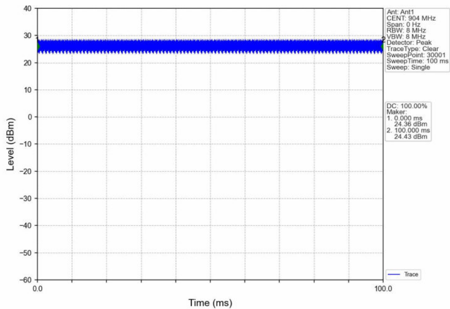
16QAM_LCH_904MHz_Ant1_NTNV
