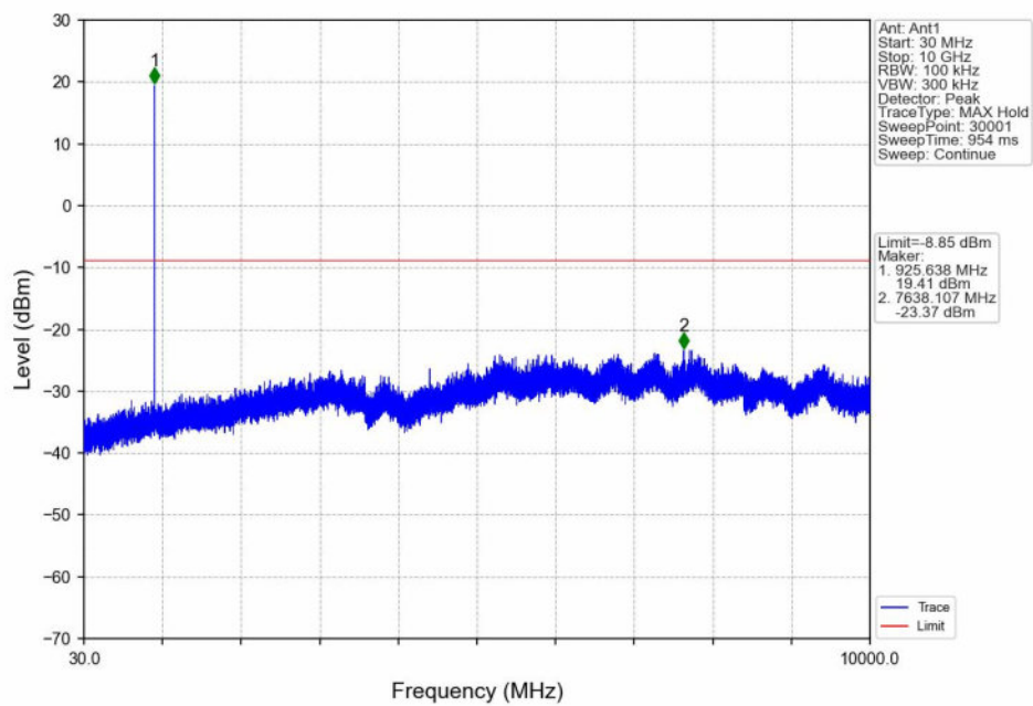
16QAM_HCH_926MHz_Ant1_NTNV
