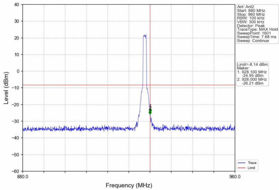
QPSK_HCH_926MHz_Ant2_NTNV
