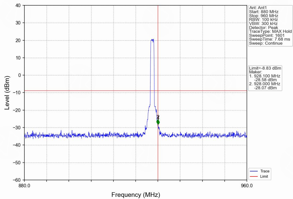
QPSK_HCH_926MHz_Ant1_NTNV
