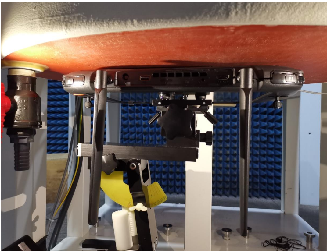
Vertical mode (1g/10g SAR for ANT 5 and ANT 6)(0mm)
