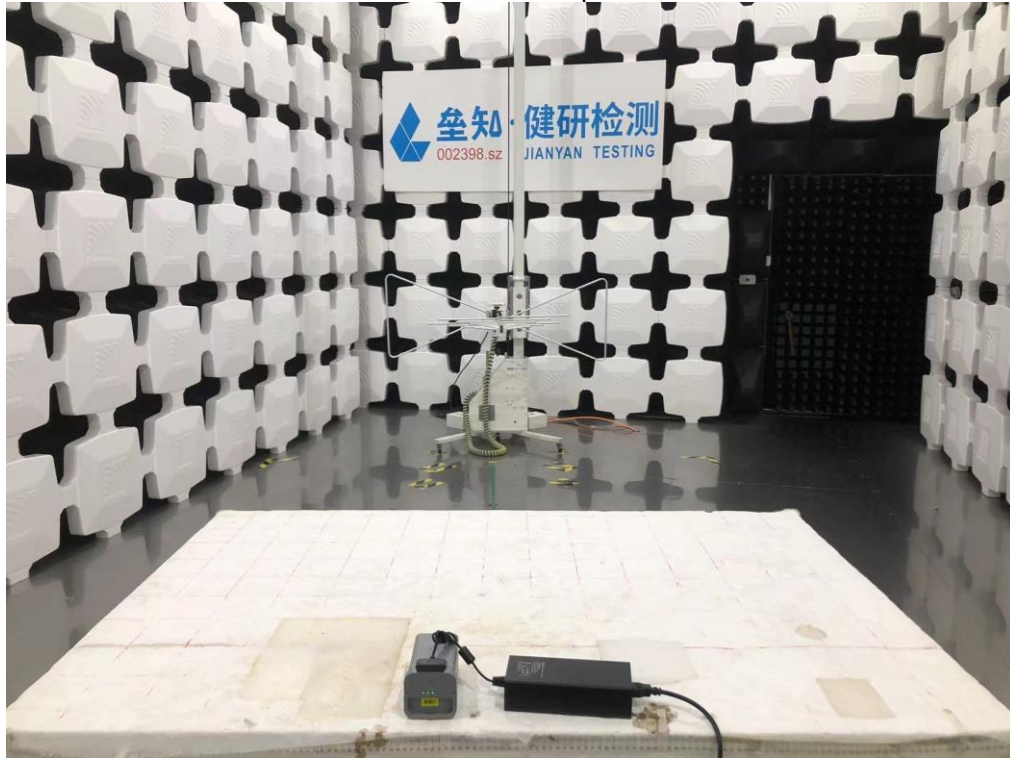
Radiated Spurious Emission Below 1GHz Adapter 1
