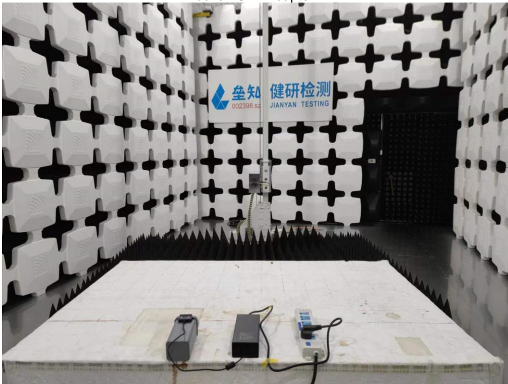
Above 1GHz Adapter 1
