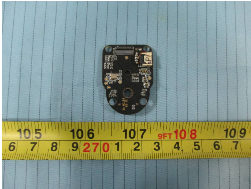
EUT – Vidicon Main Board 4 Bottom View
