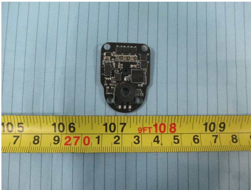
EUT – Vidicon Main Board 4 Top View
