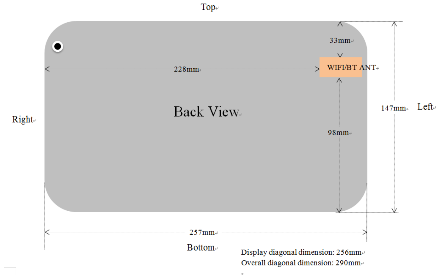
Fig.14.1 EUT Antenna Locations
