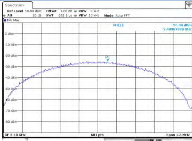
GFSK(BLE) HIGH CHANNEL
