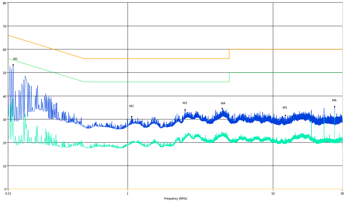
CE Test case_FCC_CE_FCC PART 15_Class B
