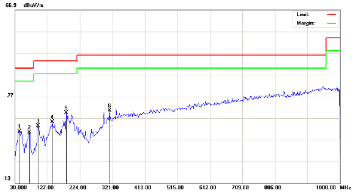
Radiated Emission Test –Horizontal -3m
