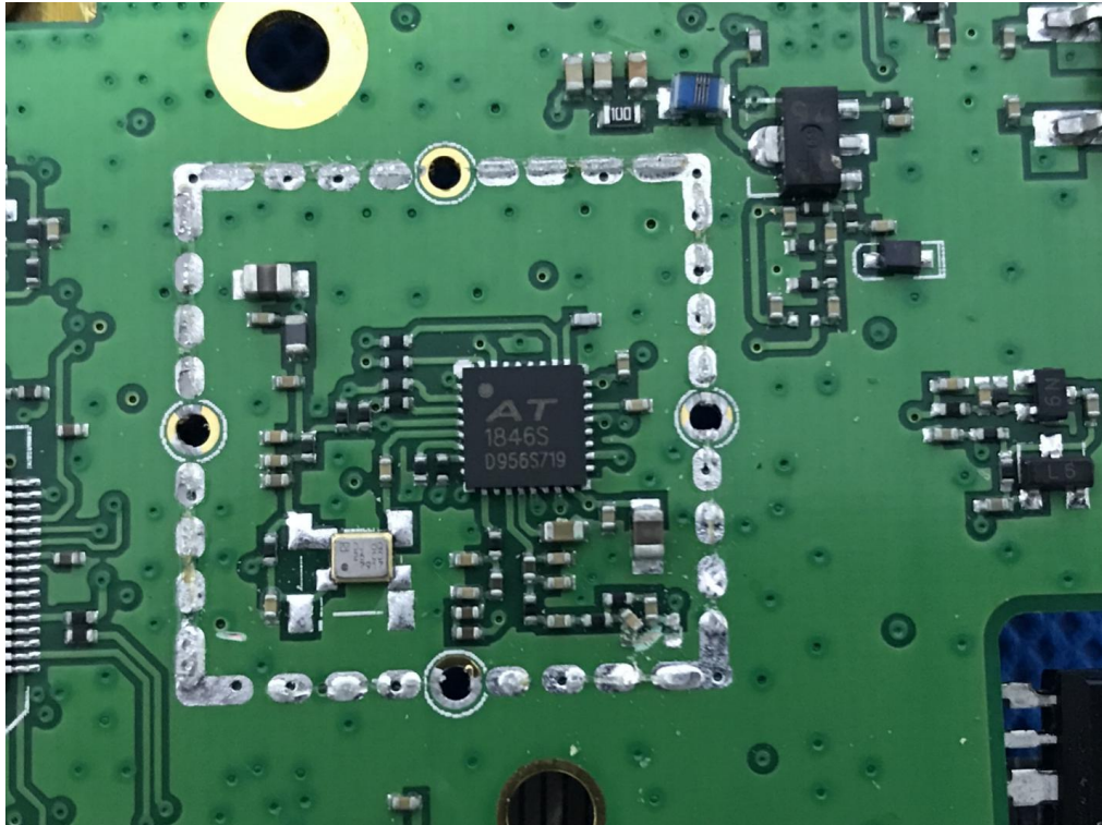
INTERNAL VIEW-3 OF EUT-1
