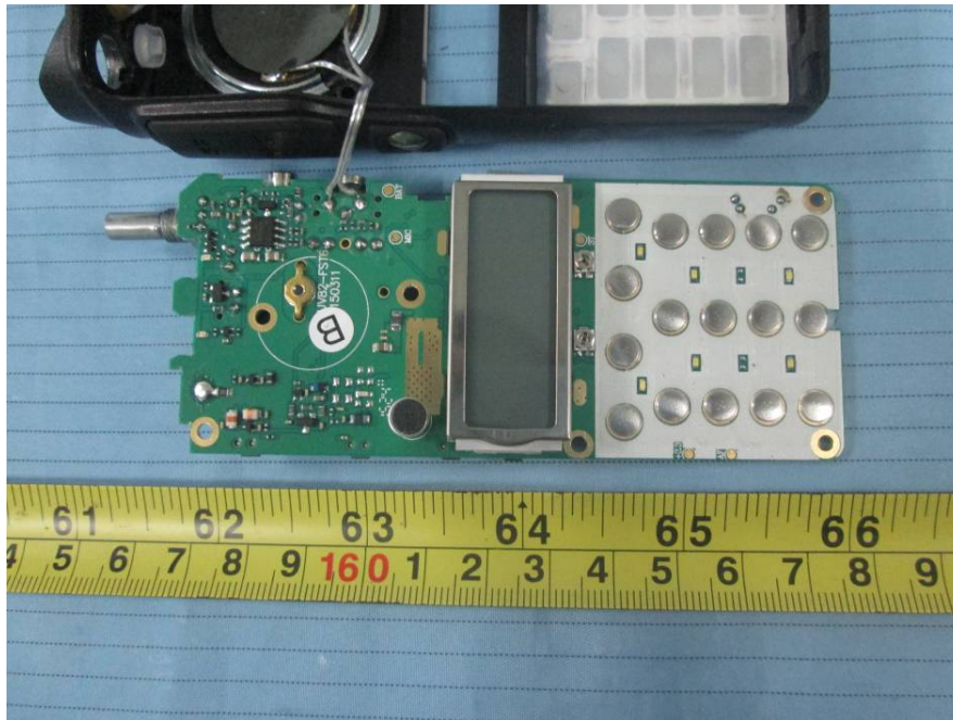
EUT- Main Board Top View (Screen)
