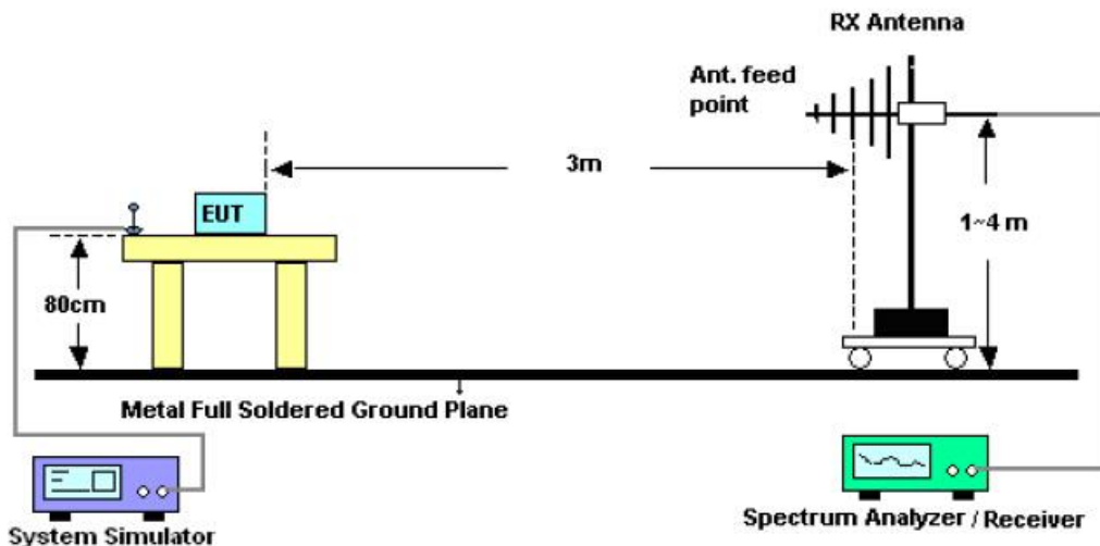
RADIATED EMISSION TEST SETUP 30MHz-1000MHz
