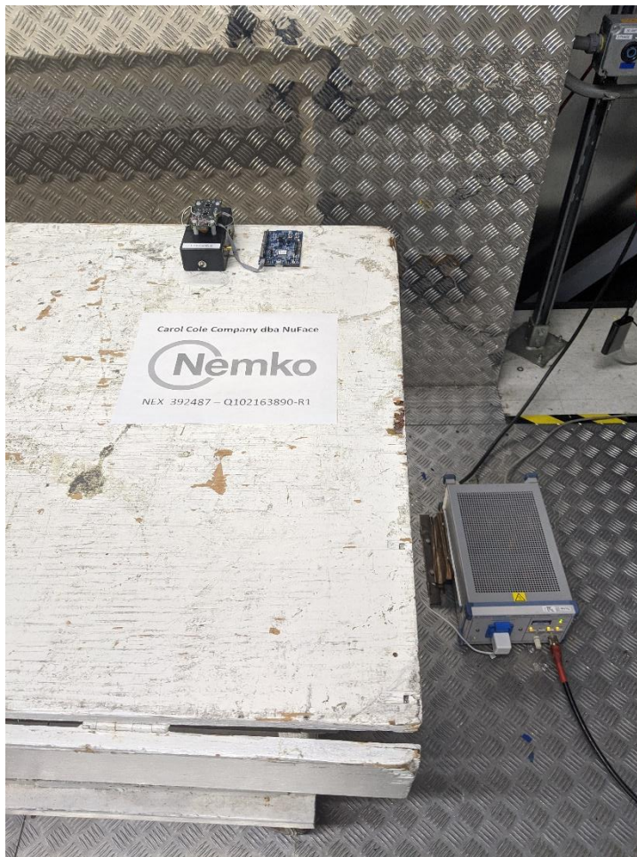
Figure 5 - Conducted AC emissions, front view
