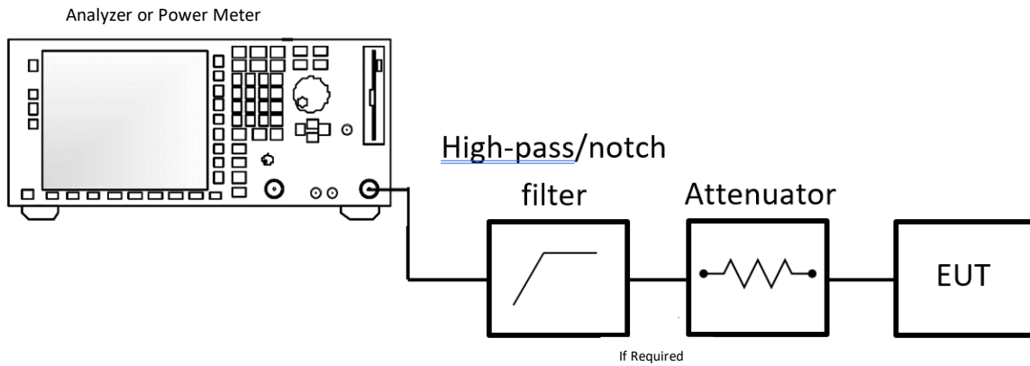
Figure 4 – Power Meter/Spectrum Analyzer Output Power and PSD
