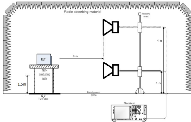
Figure 3 - Radiated emissions above 1 GHz
