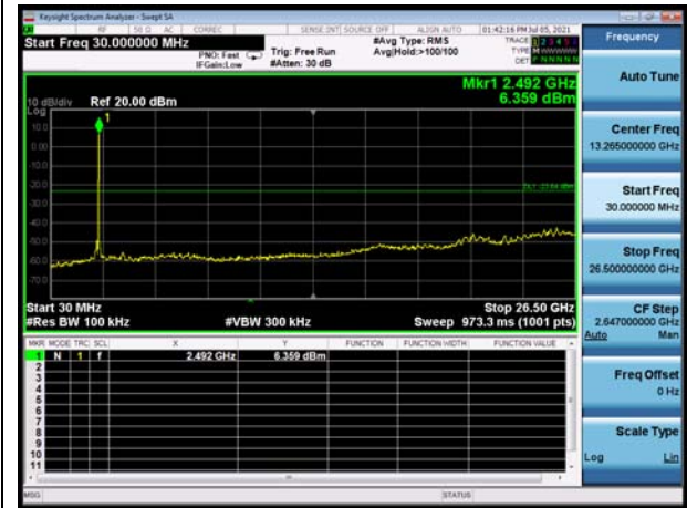
Zigbee CH26
