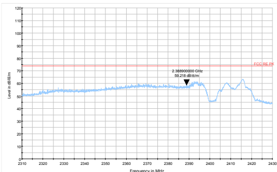
802.11g-Channel 1 Peak
