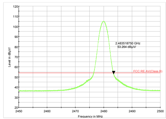
Zigbee-Channel 26: Average
