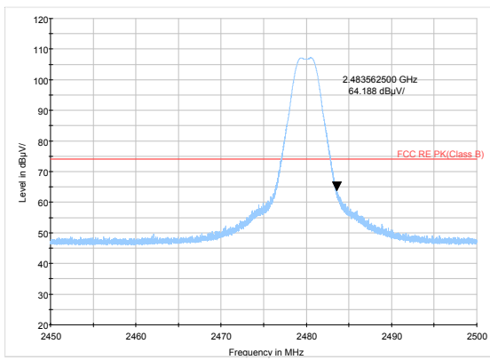
Zigbee-Channel 26: Peak
