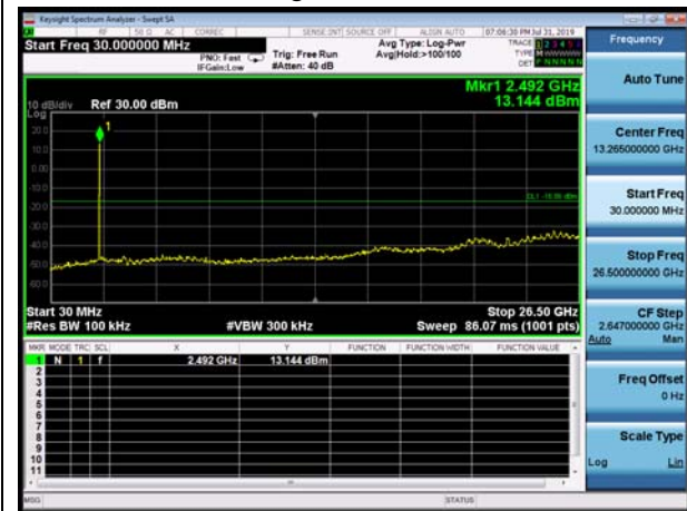
Zigbee CH26
