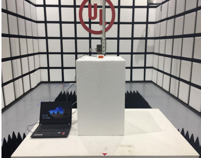
RADIATED RF MEASUREMENT SETUP (ABOVE 1 GHz)
