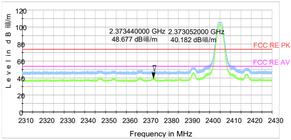
Zigbee-Channel 11: Peak & Average
