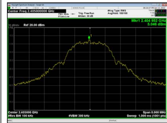
Zigbee, Channel No.: 11
