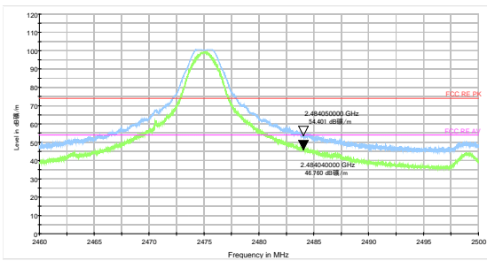
Zigbee-Channel 25: Peak + Average
