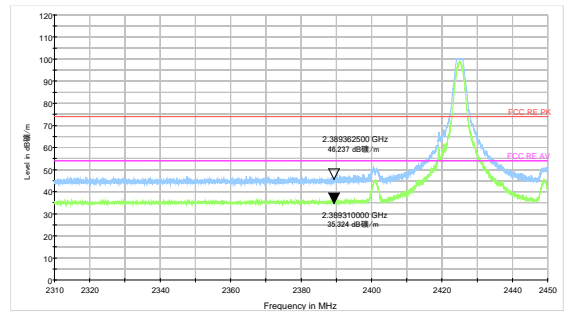
Zigbee-Channel 15: Peak + Average
