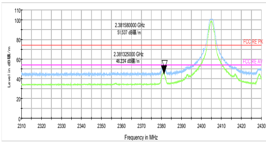
Zigbee-Channel 11: Peak + Average
