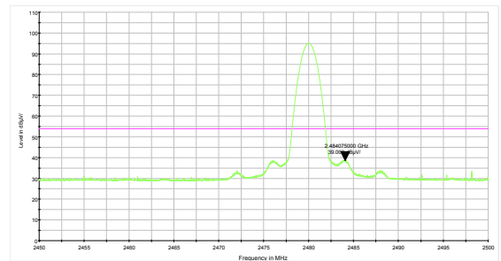
Zigbee-Channel 26: Average
