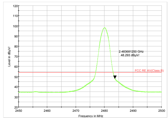
Zigbee-Channel 26: Average
