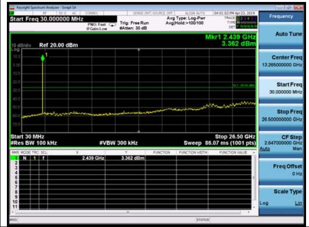
Zigbee CH18
