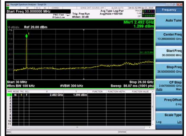
Zigbee CH26
