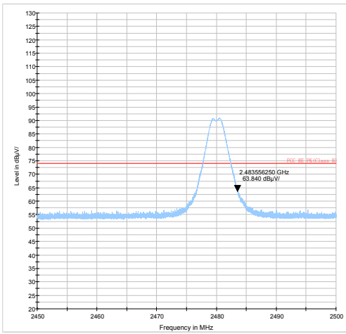
Zigbee-Channel 26: Peak
