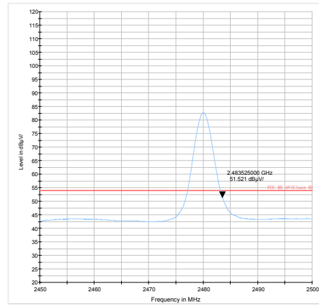
Zigbee-Channel 26: Average
