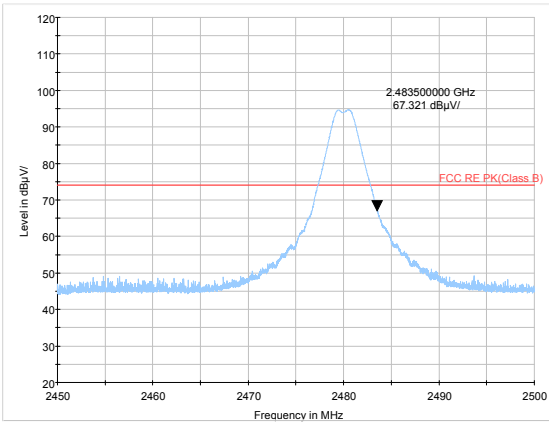
Zigbee-Channel 26: Peak
