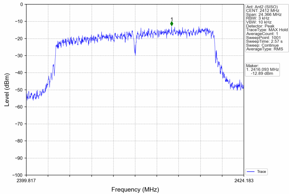
802.11ax(HEW20)_LCH_2412MHz_RU242_Left_Ant2 (SISO)_NTNV
