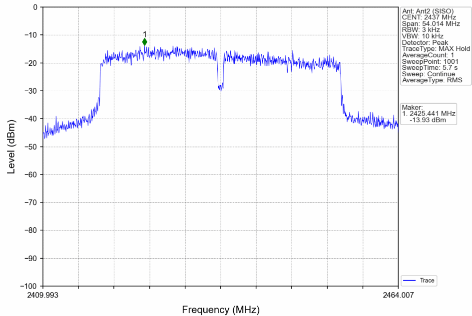
802.11ax(HEW40)_MCH_2437MHz_RU484_Left_Ant2 (SISO)_NTNV
