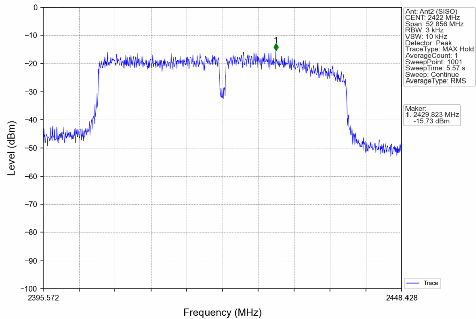
802.11ax(HEW40)_LCH_2422MHz_RU484_Left_Ant2 (SISO)_NTNV
