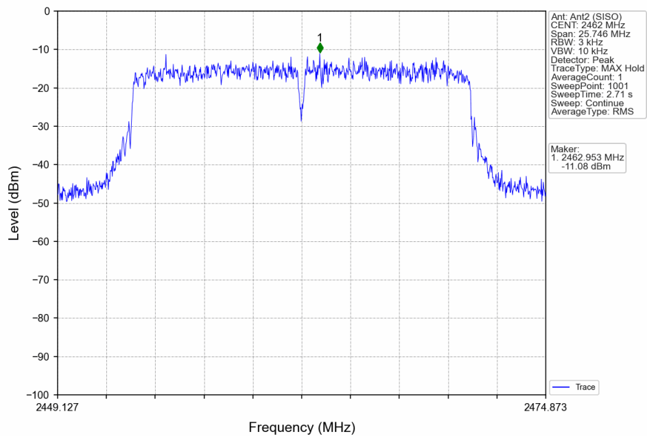
802.11ax(HEW20)_HCH_2462MHz_RU242_Left_Ant2 (SISO)_NTNV
