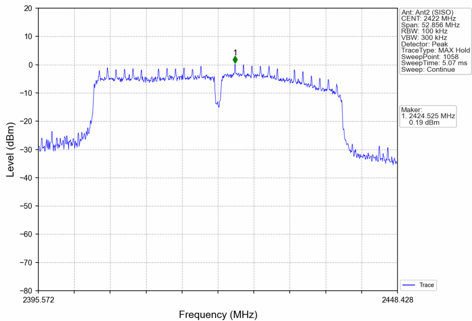
802.11ax(HEW40)_LCH_2422MHz_RU484_Left_Ant2 (SISO)_NTNV
