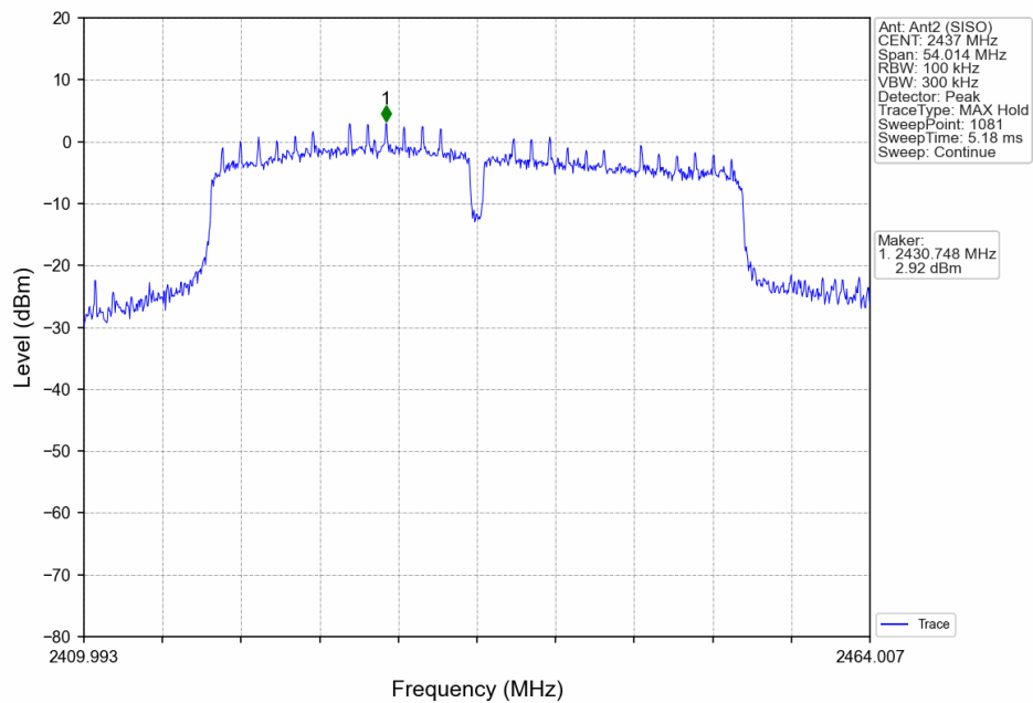
802.11ax(HEW40)_MCH_2437MHz_RU484_Left_Ant2 (SISO)_NTNV
