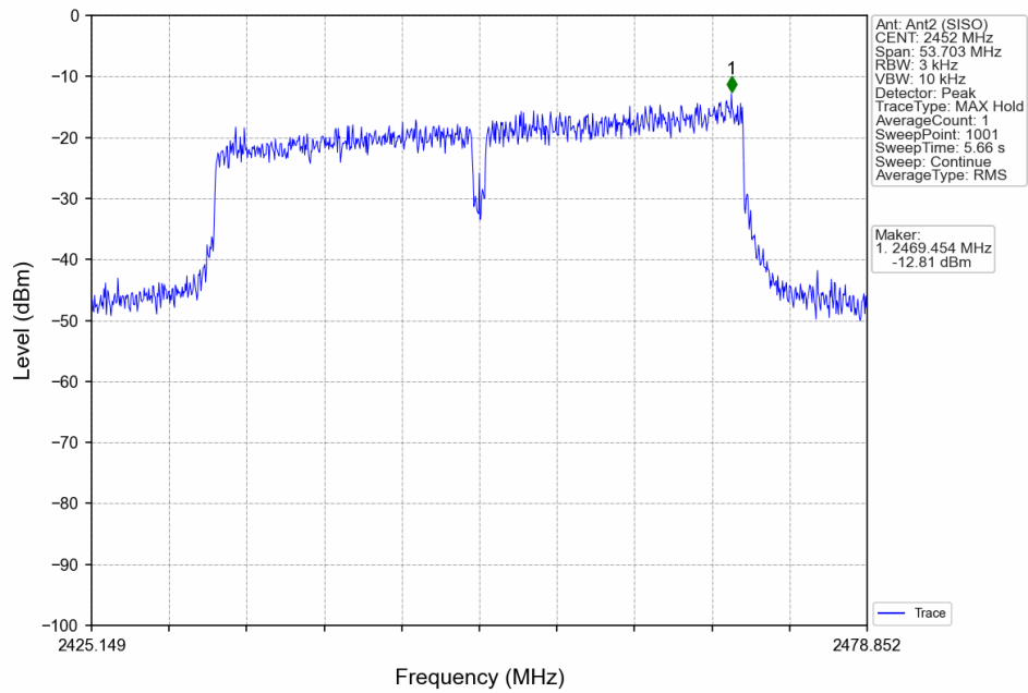
802.11ax(HEW40)_HCH_2452MHz_RU484_Left_Ant2 (SISO)_NTNV
