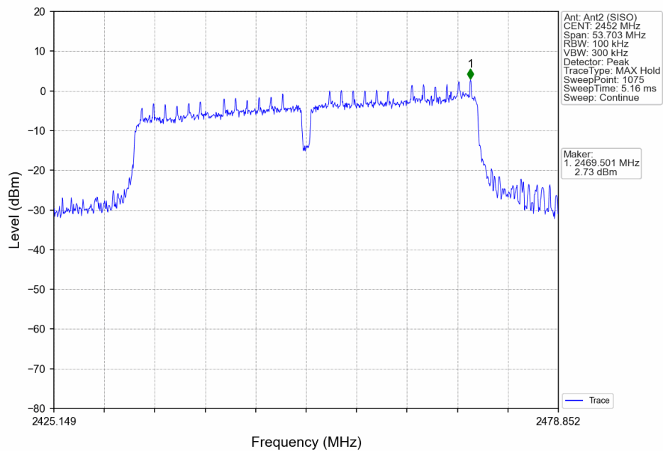
802.11ax(HEW40)_HCH_2452MHz_RU484_Left_Ant2 (SISO)_NTNV
